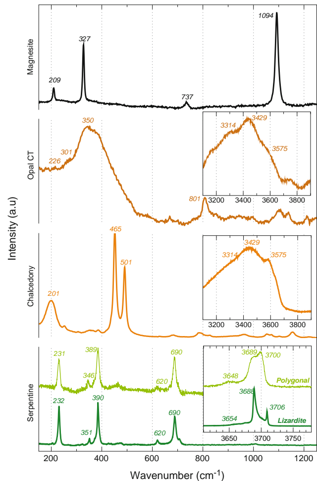
Fig. 5 Typical Raman spectra observed for serpentine (lizardite and polygonal), chalcedony, opal-CT and magnesite composing the serpentinite sole of the New Caledonia ophiolite
