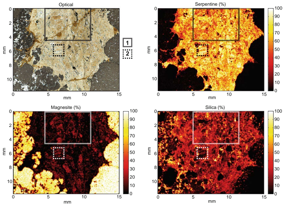
Fig. 7 Spatial repartition and quantification of mineral phases (in %) calculated on each pixel of the mapped area (Fig. 2d), based on \mu -XRF measurements (EDAX Eagle III). Square-delimited regions correspond to areas used to construct correlation diagrams in Fig. 8
