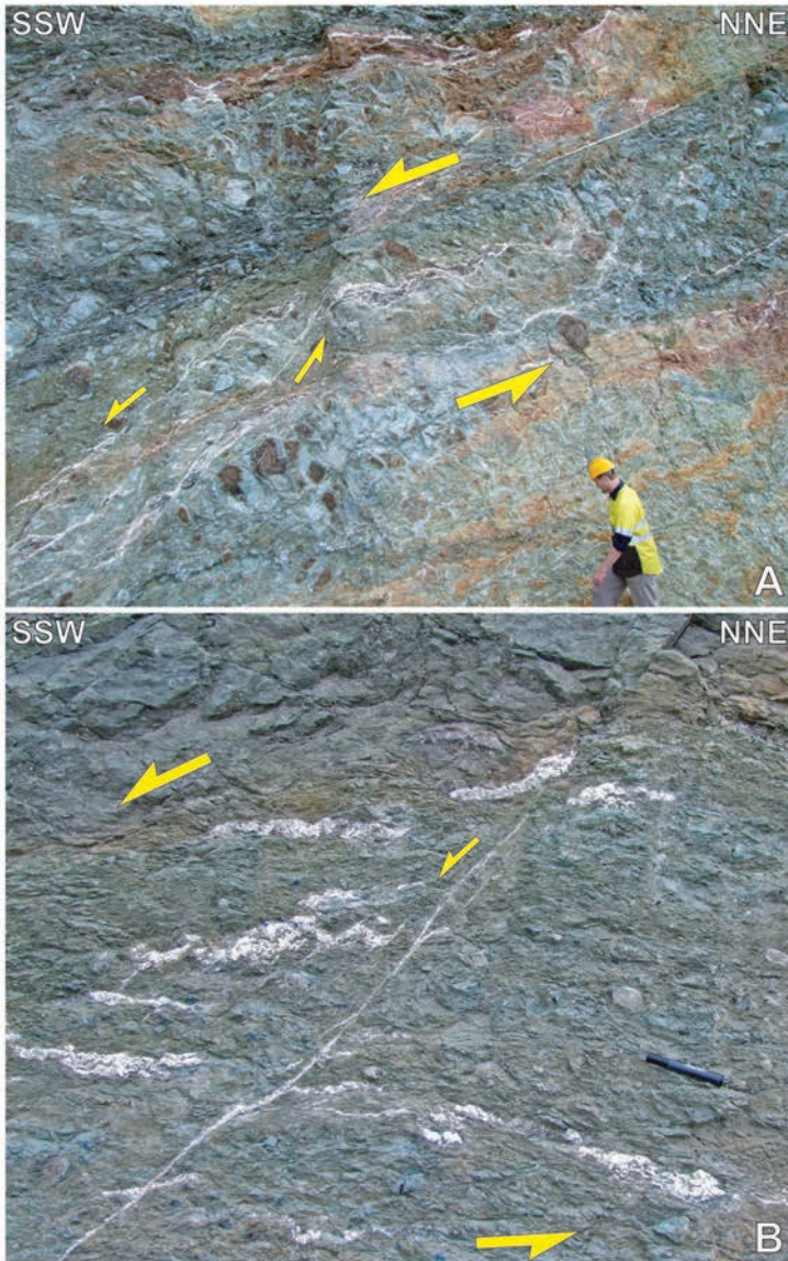
Figure DR1. Additional field views in the serpentine sole of the Koniambo Massif. A, a low-dipping shear zone and associated 'type 1' magnesite veins. In this example, three subtypes of vein may be distinguished: (i) a planar vein running along, and parallel to, the roof of the shear zone, (ii) subplanar veins inside, and oblique to, the shear zone, representing Riedel- or C'-type shear planes, (iii) a folded composite vein inside, and broadly parallel to, the shear zone. Folding seems to result from both buckling and drag folding along the shear planes. B, a mylonite zone hosting 'type 1' magnesite veins. A first subtype consists of sheared veins paralleling the schistosity. A second subtype consists of thinner veins along Riedel- or C'-type shear planes.
