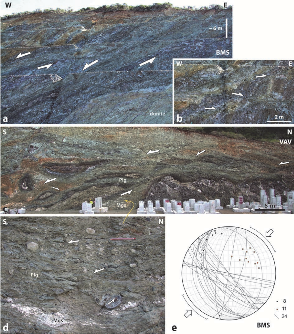
Figure 11 Field views of the serpentinite sole in the Vavouto peninsula, along the BMS (a & b) and VAV (c & d) sections. Plg, polygonal serpentinite; Mgs, magnesite. e) Stereogram (lower hemisphere, equal-area projection) showing the orientation, along the BMS section, of large shear planes (shown as orange squares representing poles of planes), of planar magnesite veins (shown as great circles) in between major shear zones, and of fold axes (shown as black dots) of folded magnesite veins within the shear zones.
