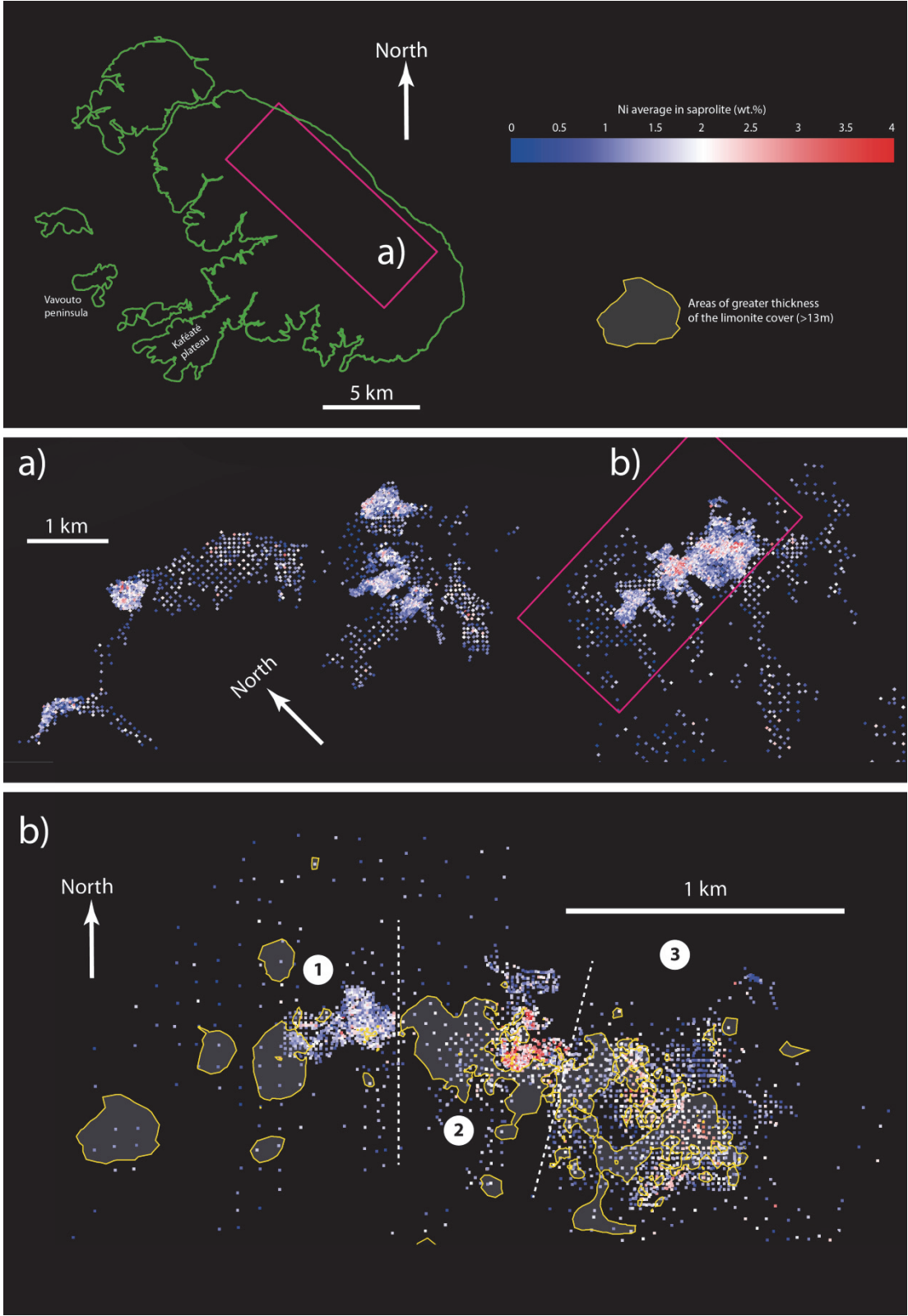
Figure 7 a) Average Ni content in the saprolite calculated for each borehole (each point on the figure) in the main exploited area. b) Focus on the Ni richest area where boreholes distribution is not too variable and where their density is high. The area of maximum thickness of the limonite cover is also represented
