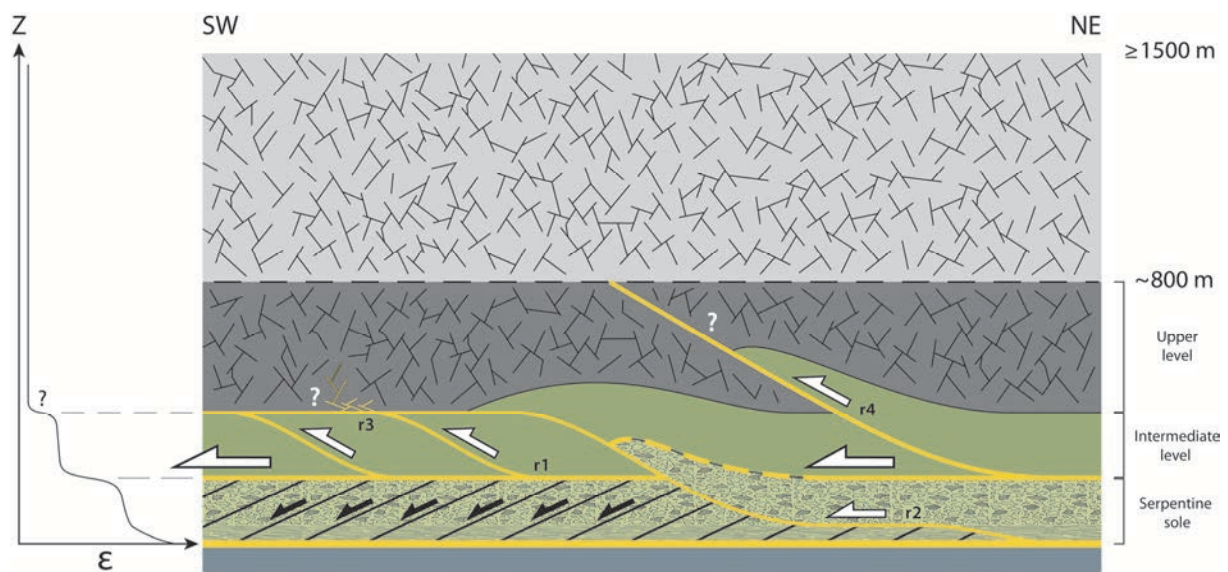
Figure 16 Schematic cross-section depicting the vertical distribution of deformation within the Peridotite Nappe by the time top-to-SW shearing occurred along the serpentine sole. 'r1' to 'r4' are geometric relationships discussed in the text. The thickness and the topography of the nappe are poorly constrained and are likely to have changed during deformation.
