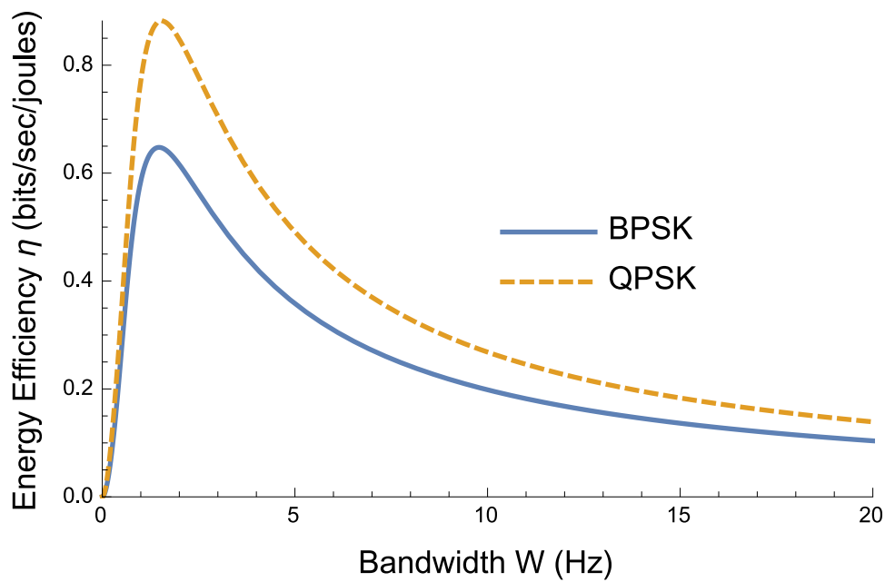
Figure 3.9: Energy efficiency vs. Bandwidth ( W ).
