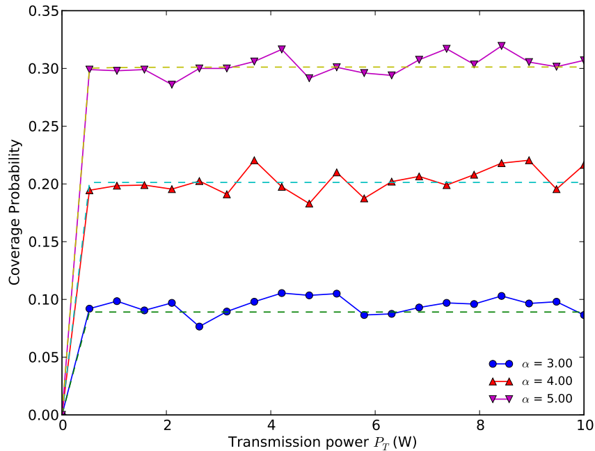
Figure 4.5: Coverage probability P_{\text{cov}} vs. transmit power P (W) for different values of \alpha and \beta = 2 \times 10^{-7} . P_{\text{cov}} asymptotically saturates to a constant value with indefinite increase in P .
