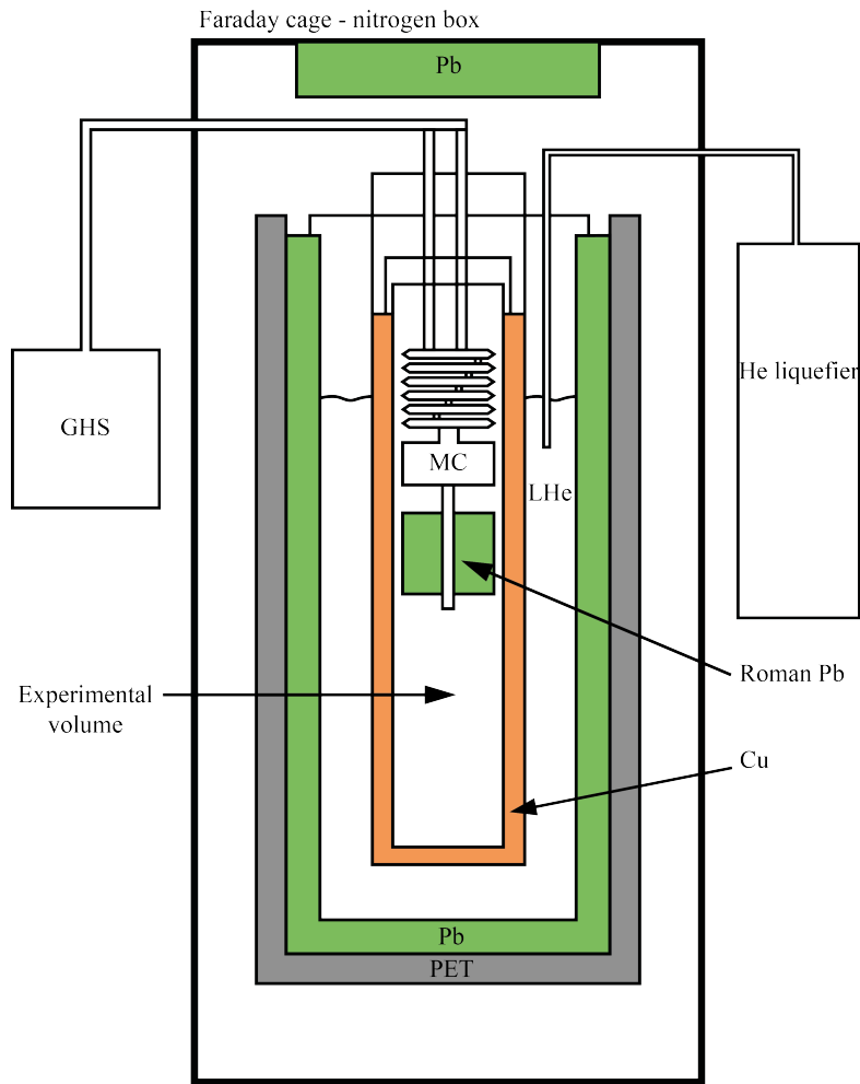
FIGURE 3.6: Scheme of the R&D cryostat in the Hall C of LNGS.
