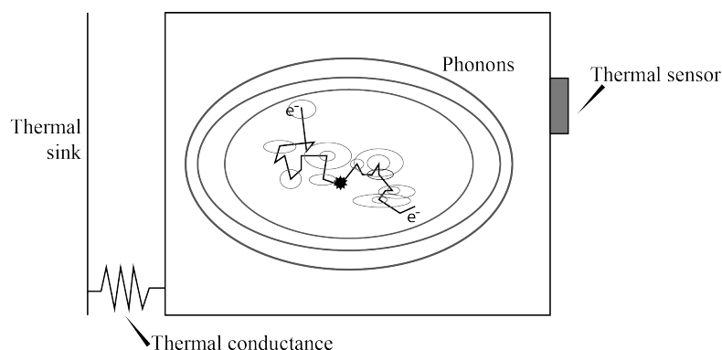
FIGURE 1.11: A bolometer consists in an absorber element where any radiation deposits its energy and increases the temperature above the thermal bath. The temperature change can be measured directly by a resistive thermometer and it is proportional to the deposited energy.
