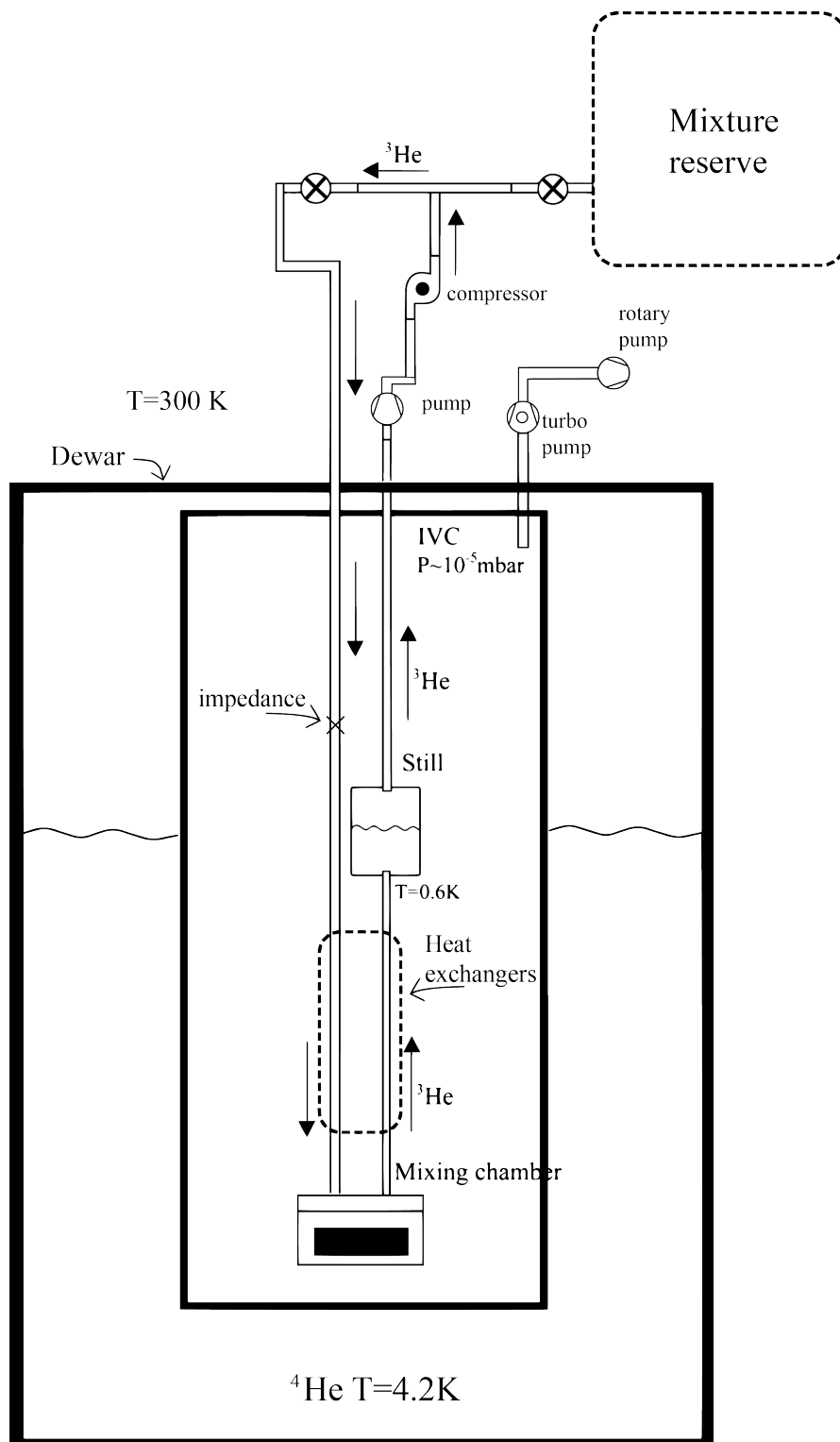
FIGURE 3.2: Scheme of a typical dilution refrigerator.
