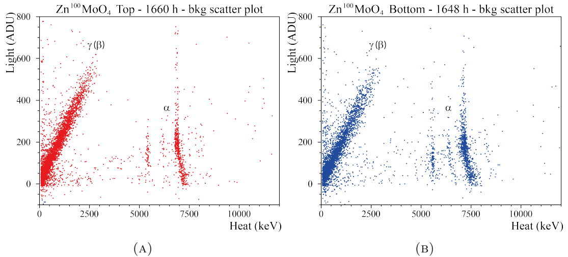
FIGURE 6.28: (A) Scatter plot for the Zn 100 MoO 4 top enriched crystal. (B) Scatter plot for the Zn 100 MoO 4 bottom enriched crystal.
