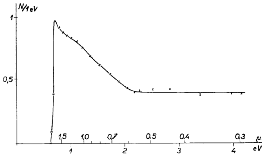
FIGURE 5.10: Number of electron-hole pairs generated in germanium by the absorption of the total energy of one electronvolt as a function of the energy of the incident radiation [67].
