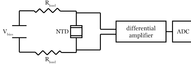
FIGURE 2.3: NTD polarization circuit.
