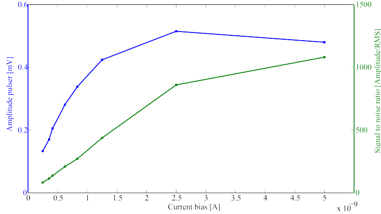
FIGURE 6.14: The sensitivity curve (blue line) and the associated signal to noise ratio (green line). The dots correspond to the available bias, the point with bias equal to 2.5 nA shows the best sensitivity and the working point at 5 nA provides the best signal-to-noise ratio. 5 nA is the correct bias option.
