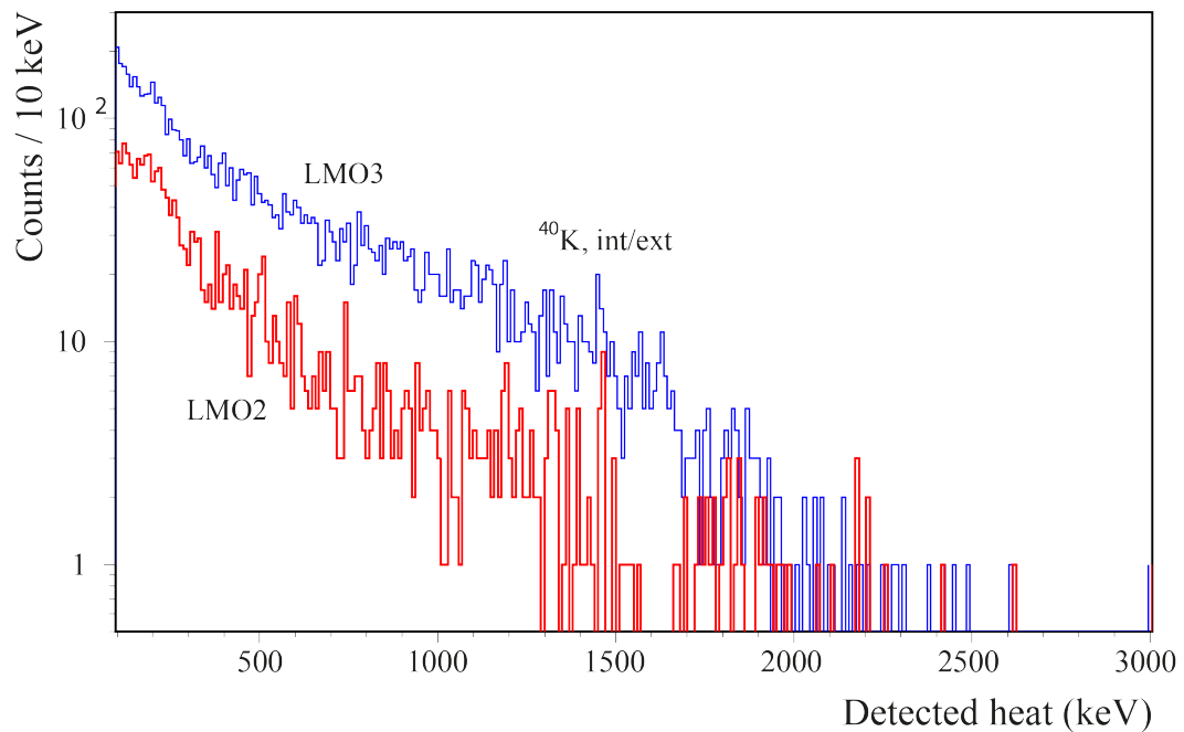
FIGURE 7.15: \gamma(\beta) background spectra of \sim 135 h: LMO3 (blue line), LMO2 (red line).
