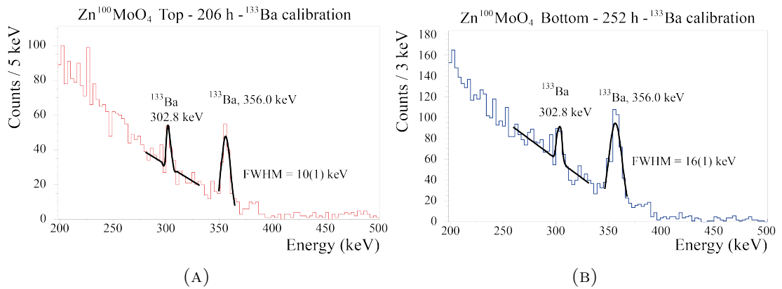
FIGURE 6.29: (A) 133 Ba calibration Zn 100 MoO 4 Top. (B) 133 Ba calibration Zn 100 MoO 4 bottom.
