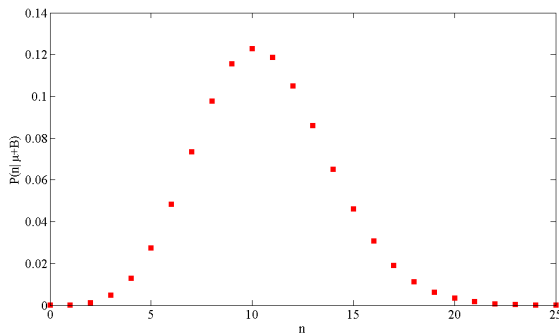
FIGURE A.3: The poissonian distribution with \mu=3.14 and \bar{B}=7.5 .
