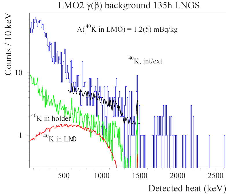
FIGURE 7.17: LMO2 \gamma background energy spectra fitted with the MC simulated spectrum for ^{40}\text{K}
