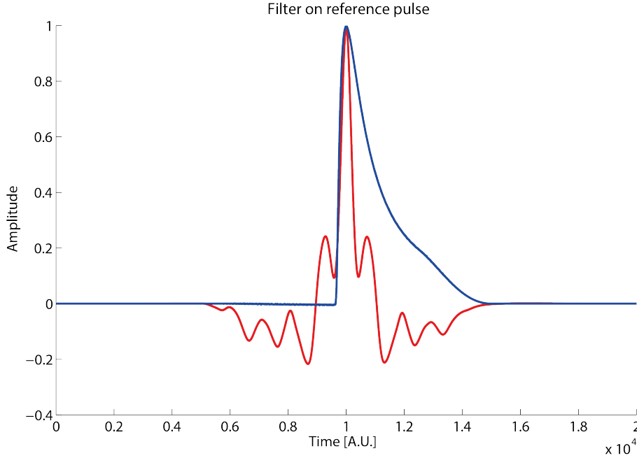
FIGURE 4.7: Blue - real reference pulse. Red - reference pulse filtered with the Gatti-Manfredi matched filter.
