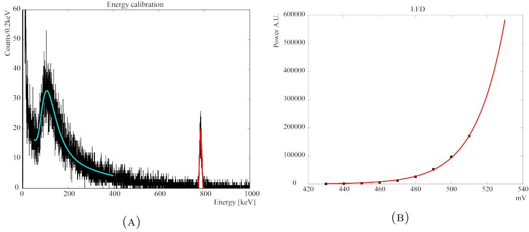
FIGURE 5.20: (A) Detector calibration with the cosmic muons (blue line). (B) LED characterization.
