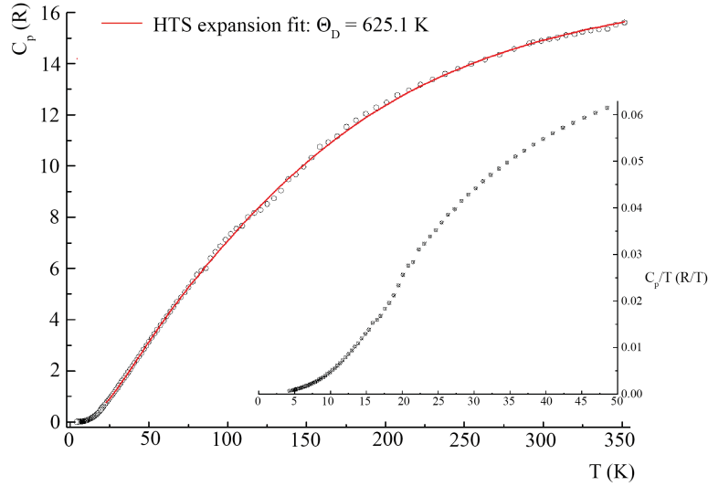
FIGURE 6.10: Specific heat measurement; the fit (red line) is performed with the HTS above 23 K. The inset shows a detail at low temperature.
