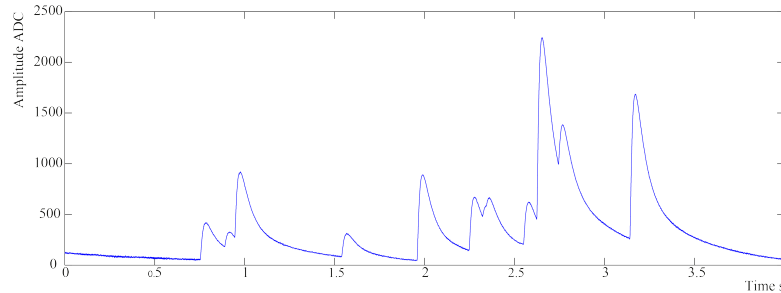
FIGURE 6.17: A dataset of four second with a 160 g ZnMoO 4 detector aboveground. A large pileup can be observed.
