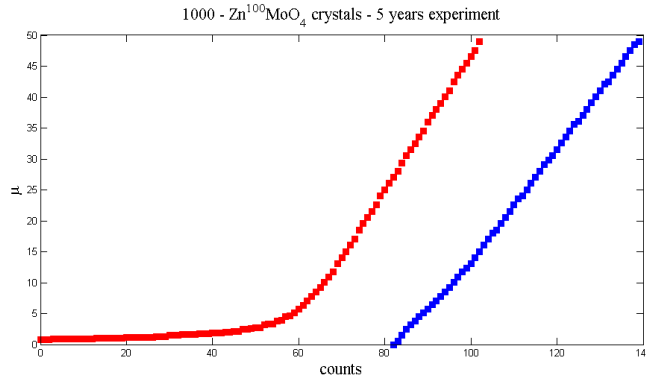
FIGURE A.7: Confidence belt for \bar{B} = 71 cts
