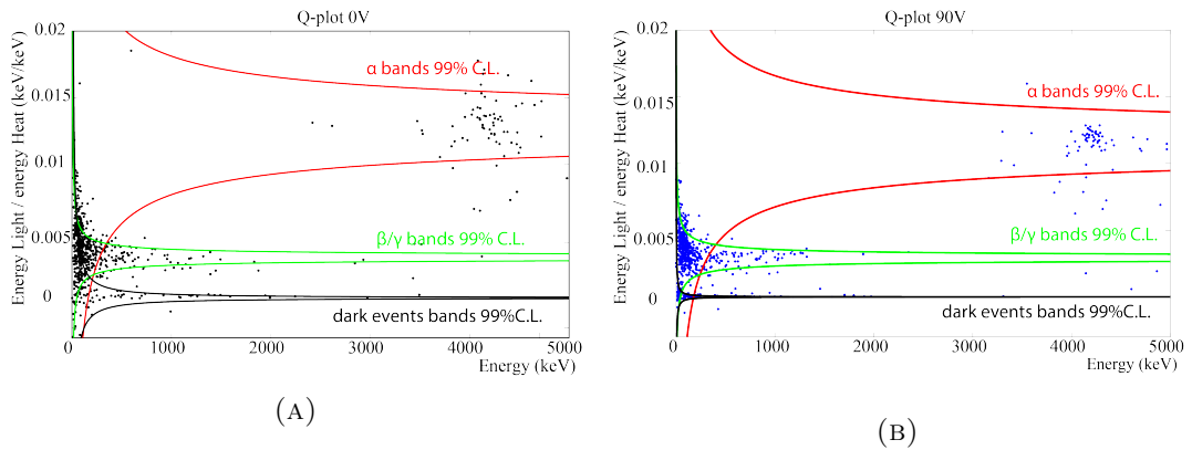
FIGURE 5.19: (A) Q plot with V_{bias}=0 V. (B) Q plot with V_{bias}=90 V.
