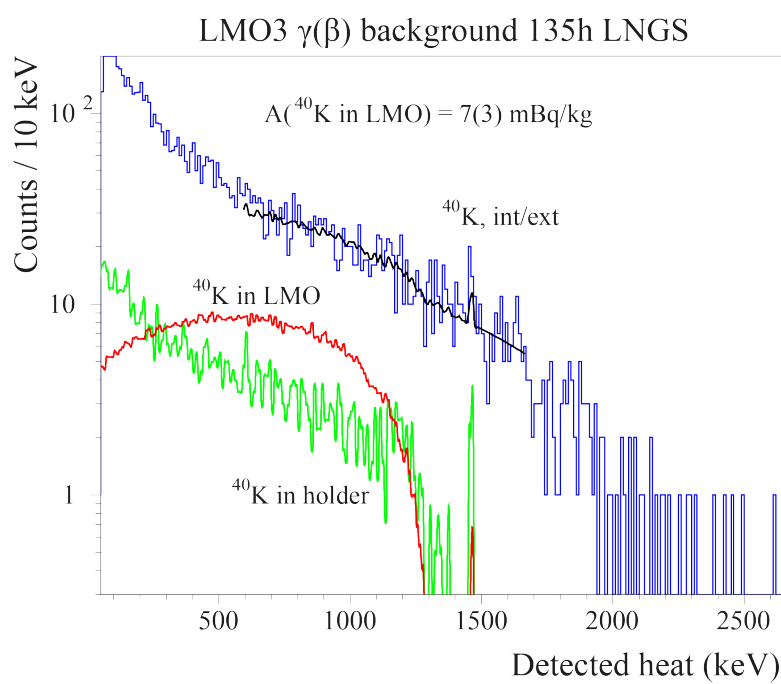
FIGURE 7.18: LMO3 \gamma background energy spectra fitted with the MC simulated spectrum for ^{40}\text{K}
