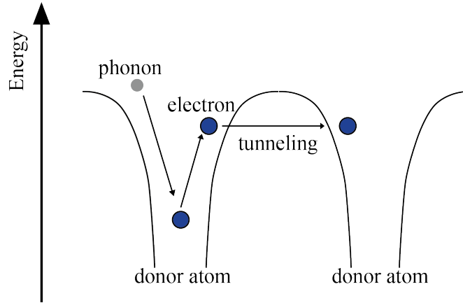
FIGURE 2.2: Simple scheme of the Variable Range Hopping mechanism. The phonon transmits its energy to the electron that can 'jump' to the near dopant site.
