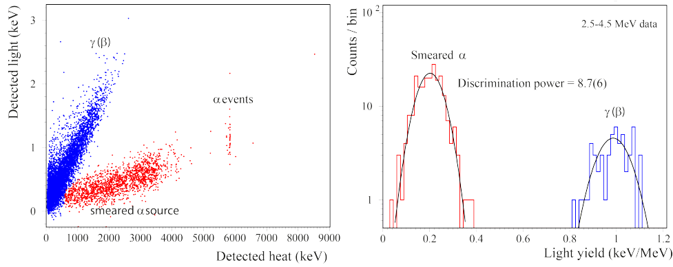
FIGURE 7.14: (LEFT) Scatter Plot. (RIGHT) Histogram of the LY in the 2.5-4.5 MeV energy range.
