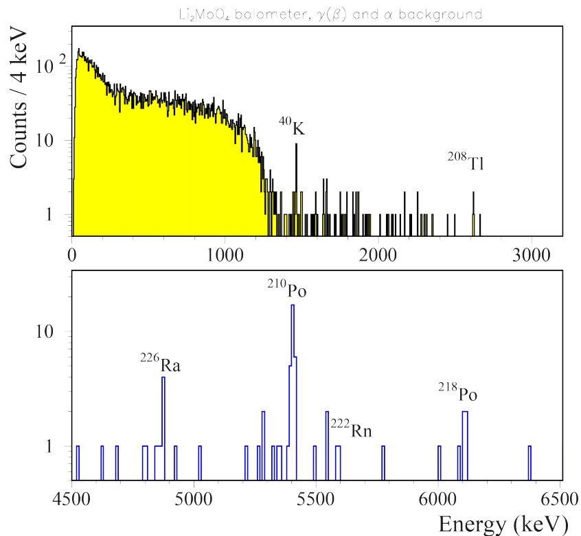
FIGURE 7.8: Background spectra of the LMO1 acquired underground during 237 h. (TOP) \gamma spectrum. (BOTTOM) \alpha spectrum.
