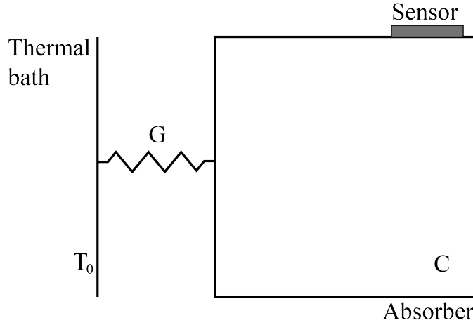
FIGURE 2.1: A bolometer could be schematically summarized as an absorber and a thermal sensor linked to a thermal bath with a thermal link.
