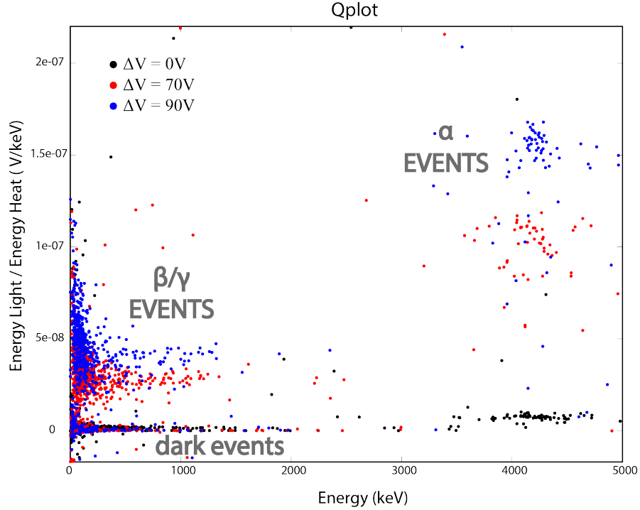
FIGURE 5.18: Comparison of three Q-plots with different V_{bias} . The light output is shown as a function of the voltage response of the detector.
