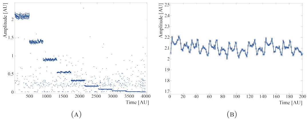
FIGURE 5.13: (A) Amplitude of the LED pulses changing the voltage across the LED. (B) Zoom of the time pattern of the LED response with 900 mV squared pulses.
