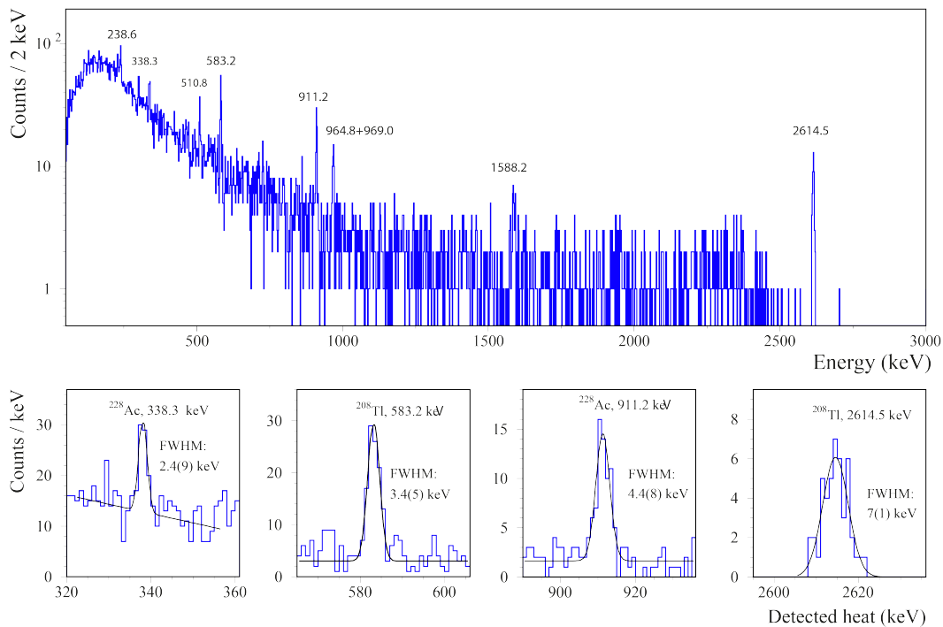
FIGURE 7.13: ^{232}\text{Th} calibration of LMO3. The insets below are details of the measured \gamma 's photo-peaks.
