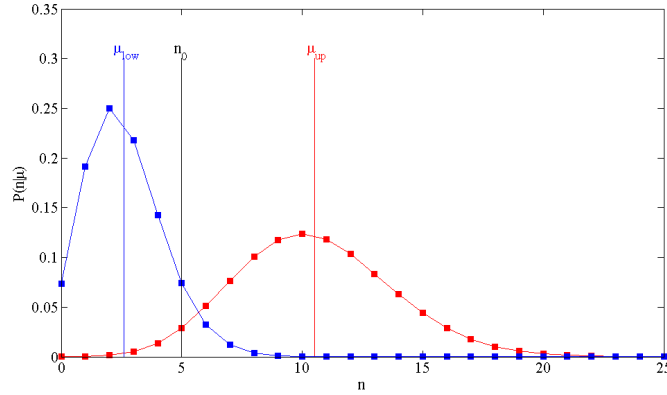
FIGURE A.1: The confidence limit calculated for an observed number of events n_0=5 , and \alpha=0.9 . In the figure the poissonian distributions for \mu_{low} (blue) and \mu_{up} (red) are shown.
