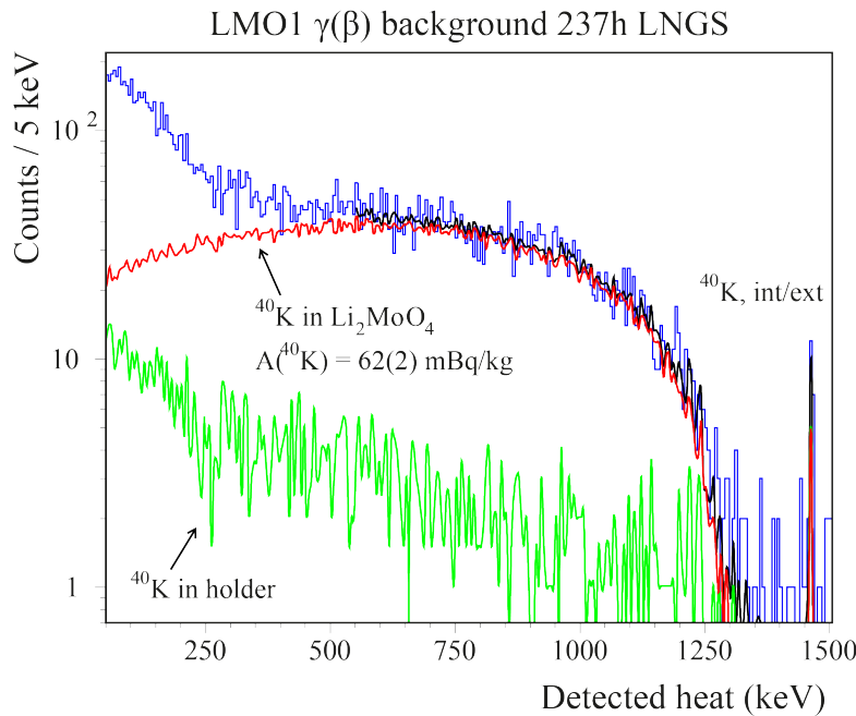
FIGURE 7.16: LMO1 \gamma background energy spectra fitted with the MC simulated spectrum for ^{40}\text{K}
