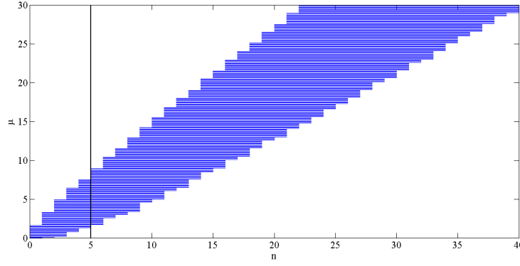
FIGURE A.4: The confidence belt obtained for an expected background \bar{B}=1 ; the black line indicates where the measurement n_0=5 intercepts some confidence belts. The union of the values of \mu corresponding to this belt is the confidence interval.
