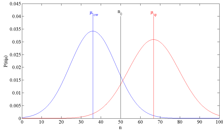
FIGURE A.2: The confidence interval calculated for an observed number of events n_0=50 , and \bar{B}=100 within the 90% of C.L. In the figure the gaussian distributions for \mu_{low} (blue) and \mu_{up} (red) are shown.
