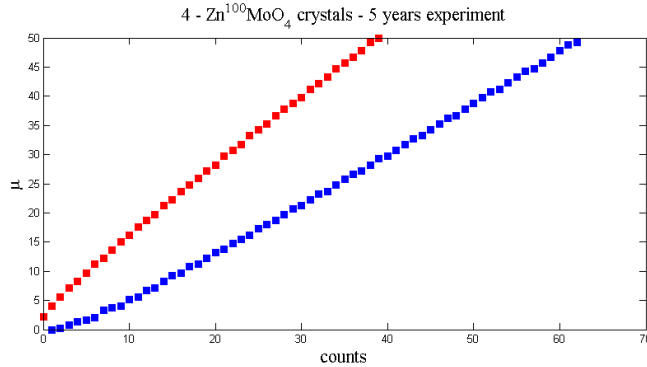
FIGURE A.5: Confidence belt for \bar{B} = 2.85 \times 10^{-1} cts
