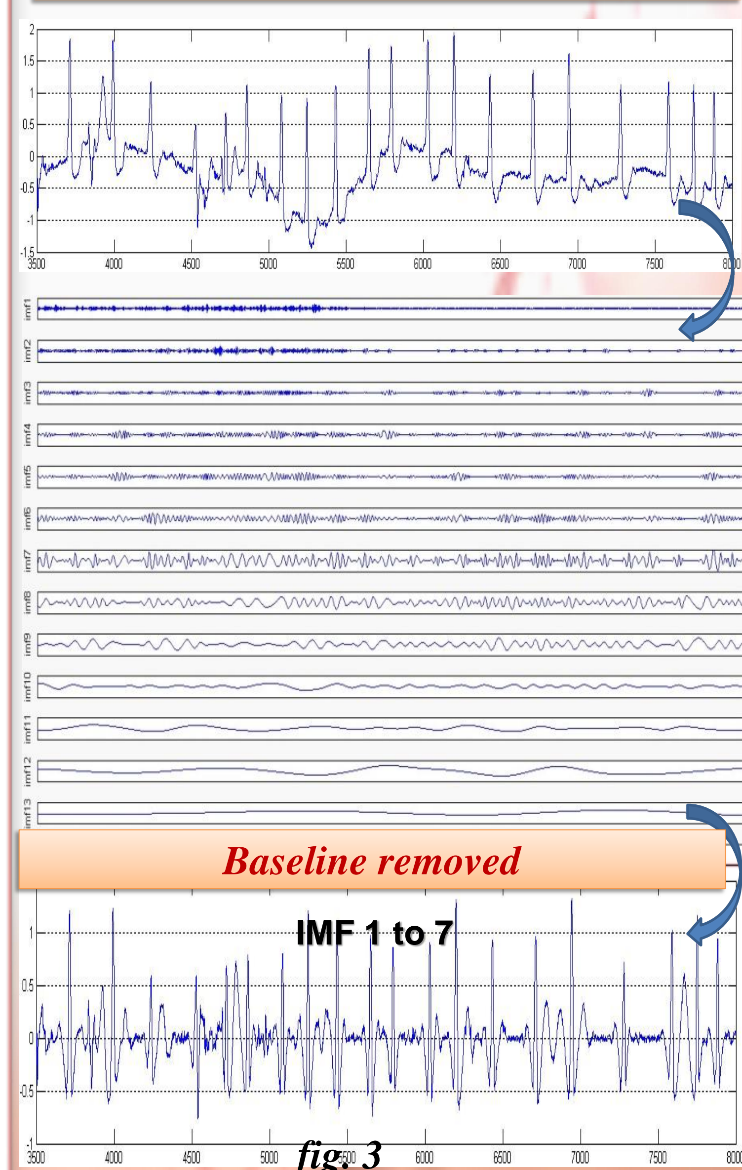
ECG signal processed using EMD
