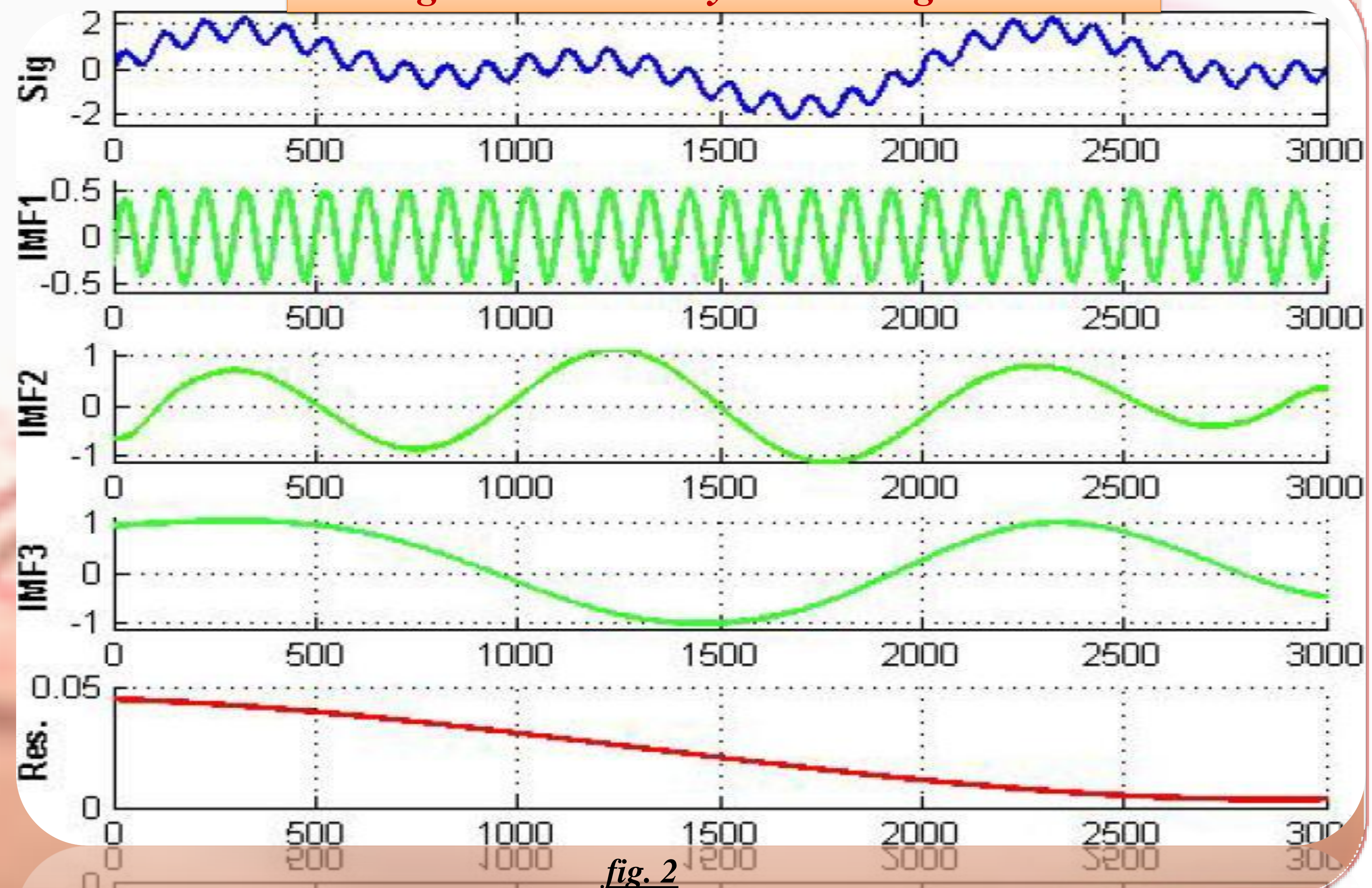
signals obtained by EMD's Algorithm
