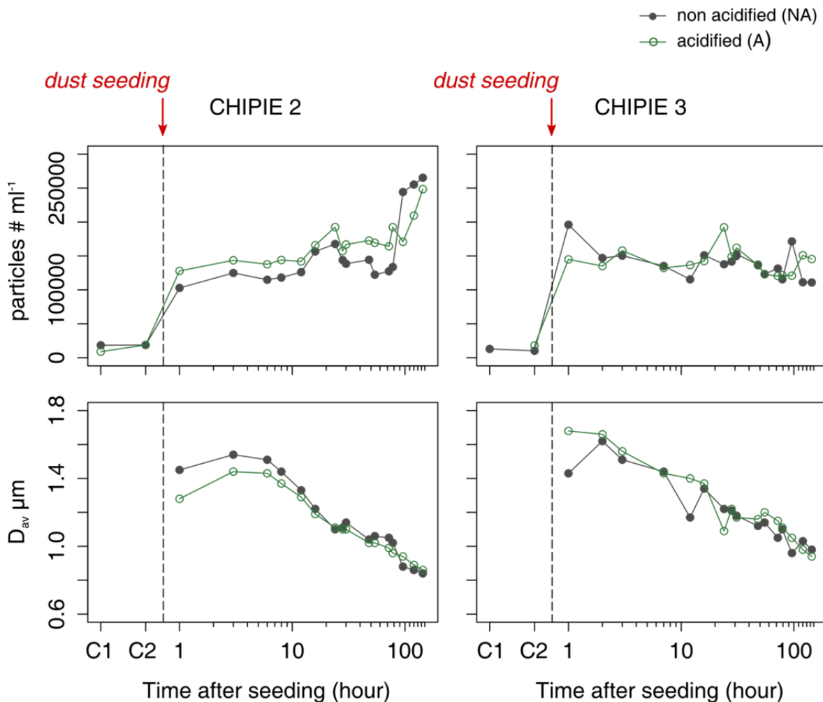
Figure 2: Evolution of the particle concentration (# mL -1 ) and the average diameter (μm) in the minicosm non-acidified “NA” (grey line) and the minicosm acidified “A” (green line) over CHIPIE 2 and 3.
