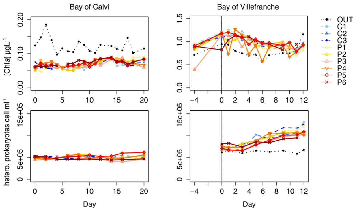
Figure 1: Evolution of the concentration in chlorophyll a (Chla) and the abundance of heterotrophic prokaryotes (hetero. prokaryotes) along the course of the experiments in the Bay of Calvi (summer 2012) and Villefranche (winter 2012) outside and inside all mesocosms. The period between day -4 and day 0 corresponds to the acidification phase.
