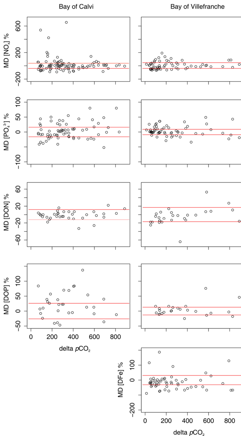
Figure 5: Relative mean deviation (MD; in %) of the concentrations of inorganic and organic nutrients as a function of delta pCO 2 (μatm) for each mesocosm at each time-point along the course of both experiments in the Bay of Calvi (BC) and in the Bay of Villefranche (BV). For each sampling date, the measured concentration in each perturbed mesocosm was subtracted from the arithmetic mean of concentrations in the 3 controls. The relative MD was estimated the ratio of this value to the mean concentration in the 3 control and expressed as a percentage. Delta pCO 2 represents the difference in pCO 2 level between the various treatments and the 3 controls for each time-point. Horizontal red lines correspond to the mean relative standard deviation of the 3 controls for each parameter over the duration of each experiment.
