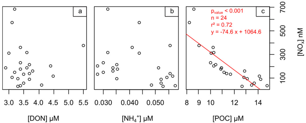
Figure 8: Nitrate + nitrite ( [NO_x] ) vs dissolved organic nitrogen ( [DON] ) (a), [NO_x] vs ammonium ( [NH_4^+] ) (b), and [NO_x] vs particulate organic carbon ( [POC] ) (c) during the experiment in the Bay of Villefranche (BV). The red line corresponds to the linear regression between [NO_x] and [POC] ( r^2 = 0.72 , p_{value} < 0.001 ). Sampling and analytical protocols for ammonium and POC measurements are described in Al-Moosawi et al. (in preparation, this issue) and Gazeau et al. (in preparation, this issue-c).
