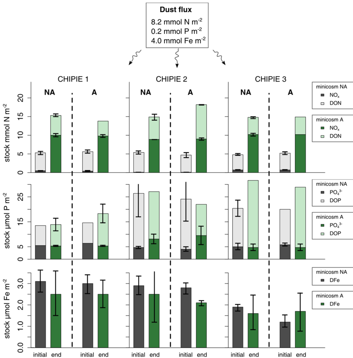
Figure 8: Comparison of the stock of N ( NO_x + DON_{UV} ; mmol m^{-2} ), P ( PO_4^{3-} + DOP_{UV} ; \mu mol m^{-2} ) and DFe ( \mu mol m^{-2} ) at T_{initial} and T_{end} . By considering a dissolution percentage of 100 % and according the chemical composition in the dust analog, the dust flux of 10 g m^{-2} should bring 8.2 mmol N m^{-2} , 0.2 mmol P m^{-2} and 4.0 mmol Fe m^{-2} . The error bar at T_{initial} corresponds to the standard deviation on the mean stock from the samples at "C1" and "C2". The error bar at T_{end} corresponds to the standard deviation on the mean stock from the samples at "T120" and "T144".
