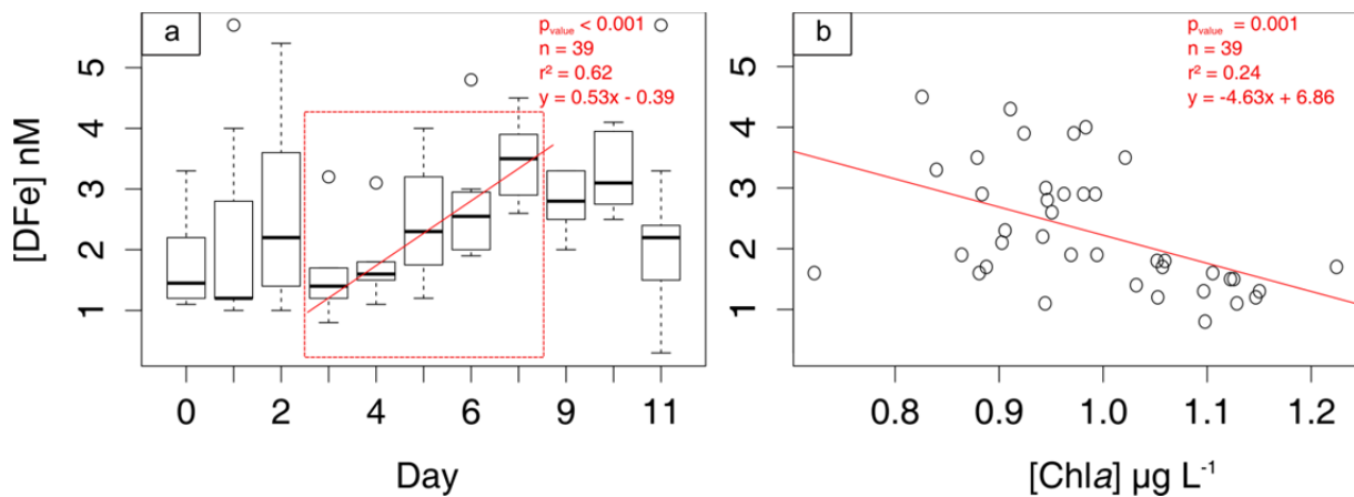
Figure 9: Box-plot of the dissolved iron concentrations ( [DFe] ) for all mesocosms along the course of the experiment conducted in the Bay of Villefranche in winter 2013. The red line represents the linear regression of [DFe] (without outlier values) as a function of time between day 3 and day 7 ( r^2 = 0.62 and p_{value} < 0.001 ) (a). Regression linear between [DFe] and the concentration of chlorophyll a ( [Chla] ) between day 3 and day 7 ( r^2 = 0.24 and p_{value} = 0.001 ) (b).
