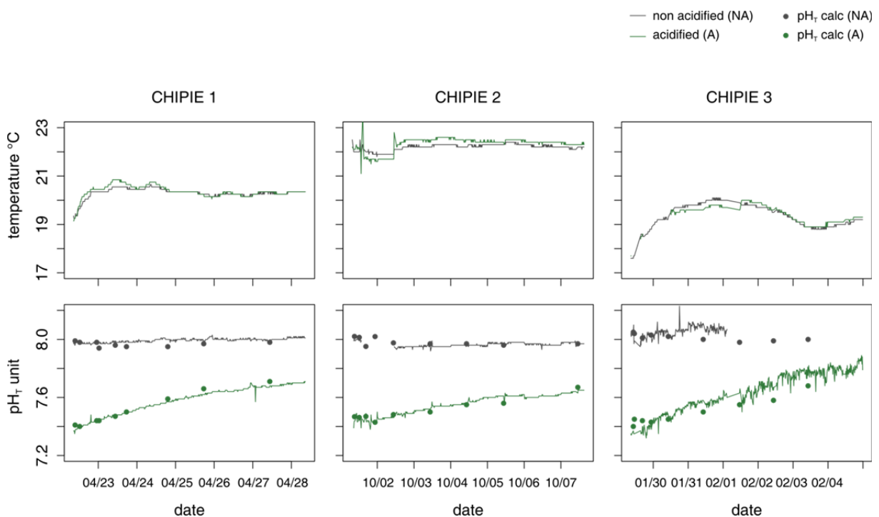
Figure 1: Follow-up of the seawater temperature ( ^\circ\text{C} ) and \text{pH}_T by Consort D230 datalogger in both minicosms. The circles represent \text{pH}_T calculated from the discrete measurements of total alkalinity ( A_T ) and dissolved inorganic carbon ( C_T )
