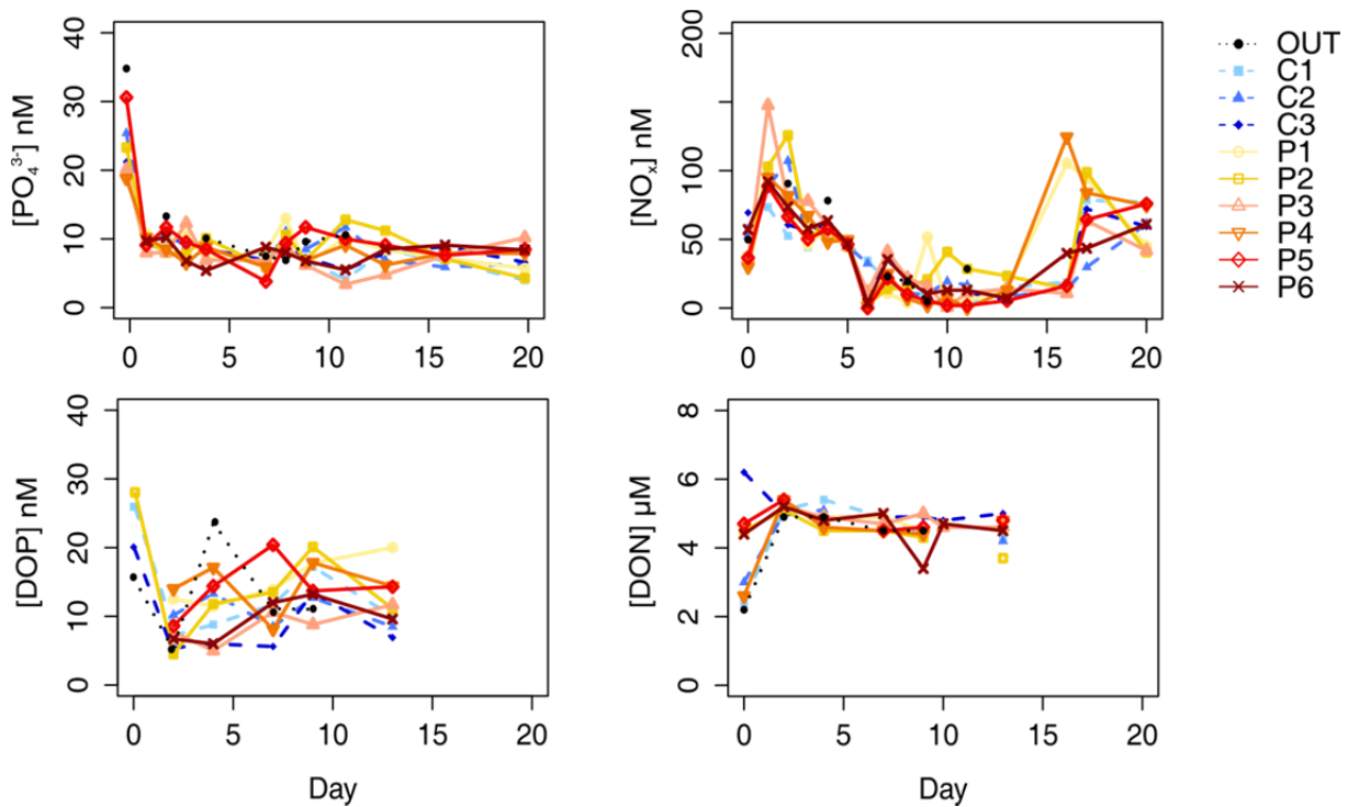
Figure 2: Evolution of the concentrations of inorganic and organic nutrients (nitrate + nitrite: NO_x , phosphate: PO_4^{3-} , dissolved organic nitrogen: DON and dissolved organic phosphorus: DOP ) outside ('OUT') and inside all mesocosms along the course of the experiment in the Bay of Calvi in summer 2012.
