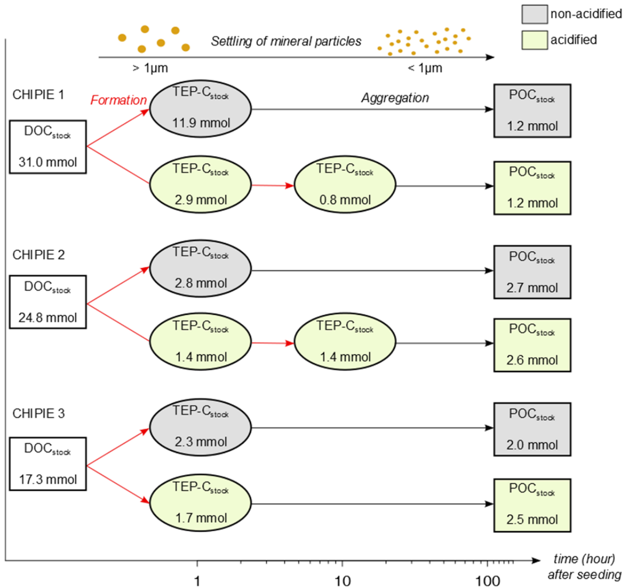
Figure 3: Estimation of the organic carbon stock (in mmol C) in both minicosms in the 3 pools: dissolved and particulate organic carbon ( DOC_{stock} and POC_{stock} ) and transparent exopolymer particles ( TEP-C_{stock} ), while mineral particles were sinking. DOC_{stock} , TEP-C_{stock} and POC_{stock} have been estimated from the DOC concentration at the sampling "C1" ( \mu\text{mol L}^{-1} ), the carbon content in TEP at T1-1.5 and T12-14 ( \mu\text{g L}^{-1} ) and the mass of POC exported at the end of the experiments.
