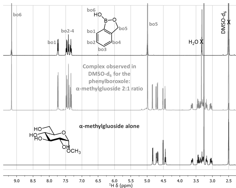
Figure II-32. ^1\text{H} NMR spectra of phenylboroxole alone, 2:1 phenylboroxole: \alpha -methylglucoside ratio and \alpha -methylglucoside alone in DMSO-d 6
