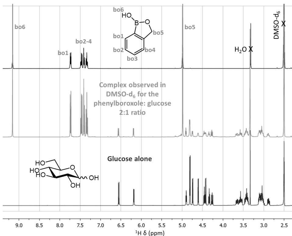
^1\text{H} NMR spectra of phenylboroxole alone, 2:1 phenylboroxole:glucose ratio and glucose alone in DMSO- \text{d}_6
