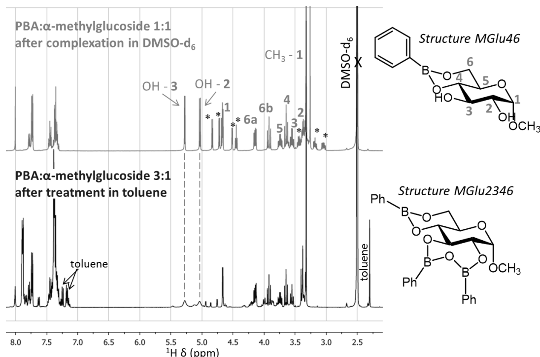
Figure II-28. Comparison of the 1 H NMR of the complex of PBA:α-methylglucoside obtained in DMSO-d 6 or after treatment in toluene (the stars correspond to the free α-methylglucoside)
