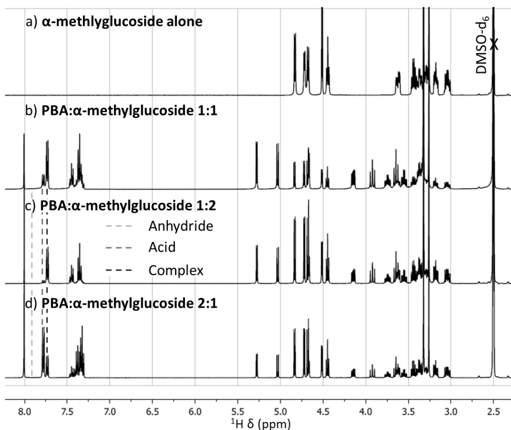
Figure II-20. ^1H NMR spectra of PBA and \alpha -methylglucoside mixtures in DMSO- d_6
