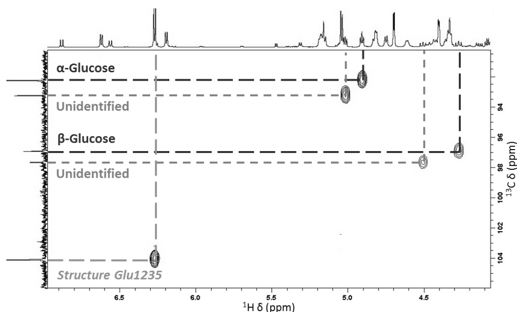
Figure II-24. HSQC in DMSO- d_6 of the 1:1 PBA:glucose ratio zoomed on the anomeric carbons – Reaction time: 8h
