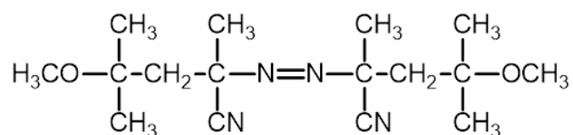
Figure III-18. V-70 (2,2'-azobis(4-methoxy-2,4-dimethyl valeronitrile)) structure
