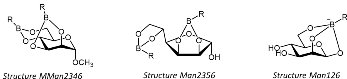
Figure II-15. Structures found in the literature for the complexation of boronic acid on \alpha -methylmannose ( Structure MMan2346 ) or on mannose ( Structure Man2356 and Man126 )
