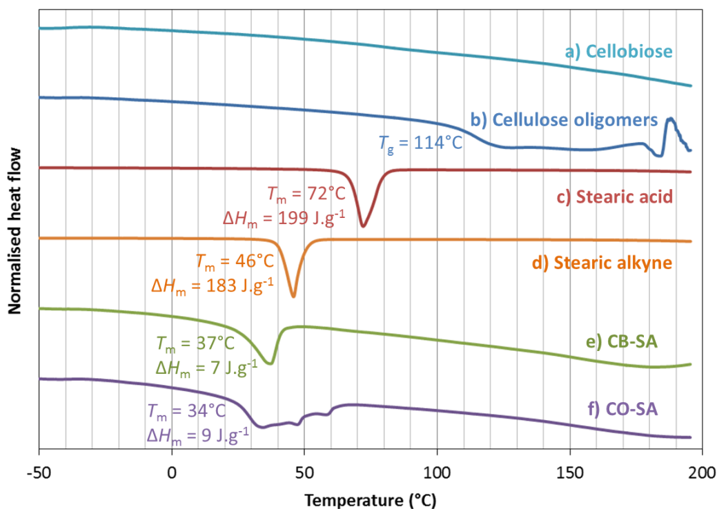
Figure V-24. DSC graphs ( N_2 , 20^\circ C \cdot min^{-1} ) of several compounds
