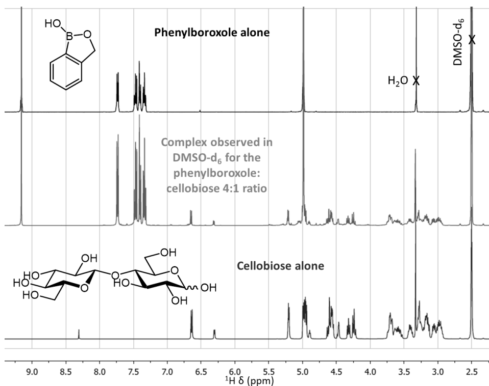
^1\text{H} NMR spectra of phenylboroxole alone, 4:1 phenylboroxole:cellobiose ratio and cellobiose alone in DMSO- \text{d}_6
