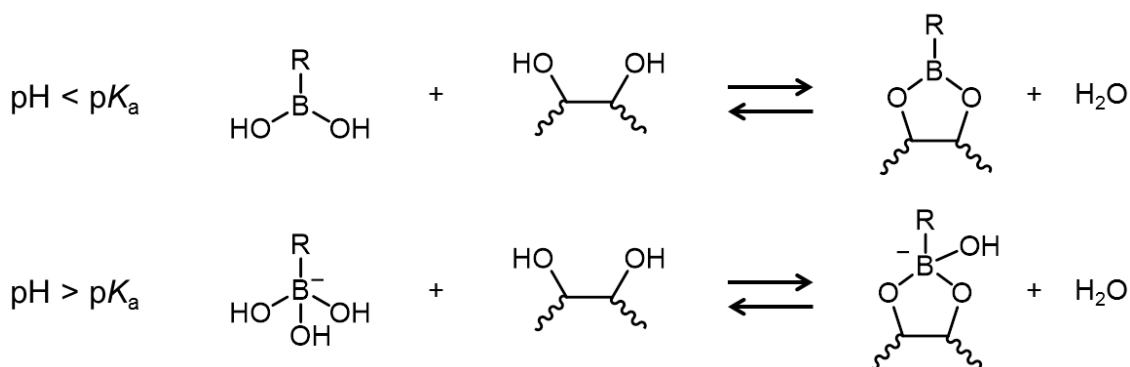
Figure II-5. Complexation of boronic acids on diol depending on the pH
