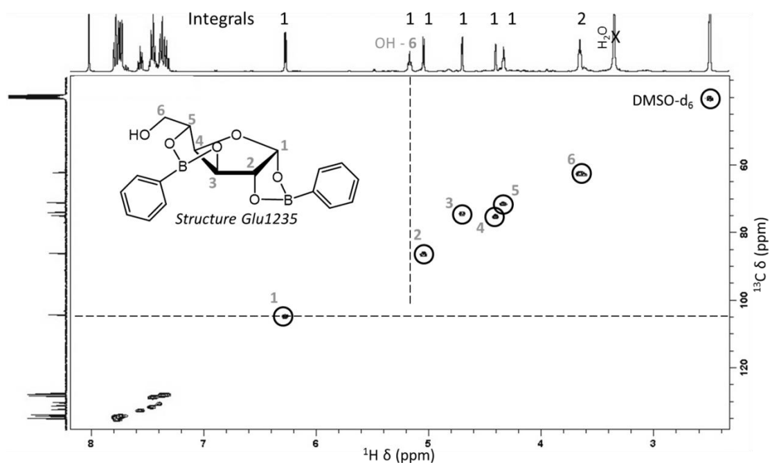
Figure II-23. Attributed HSQC for the 2:1 PBA:glucose ratio in DMSO- d_6
