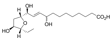
ent -9-( RS )-12- epi -ST- \Delta^{10} -13-PhytoF
