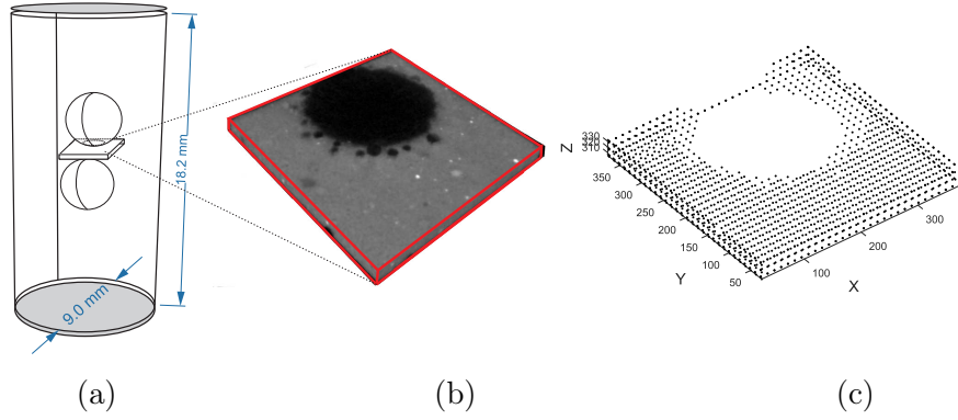
Figure 8.22: Sub-volume considered for comparisons of microcracking propagation in the lightweight plaster sample: (a) location in the sample; (b) associated CT image; (c) 3D correlation points on the surface used to define the boundary conditions.
