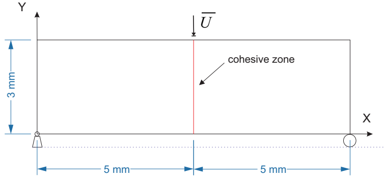
Figure 3.20: Symmetric three-point bending test problem: Geometry and boundary conditions.
