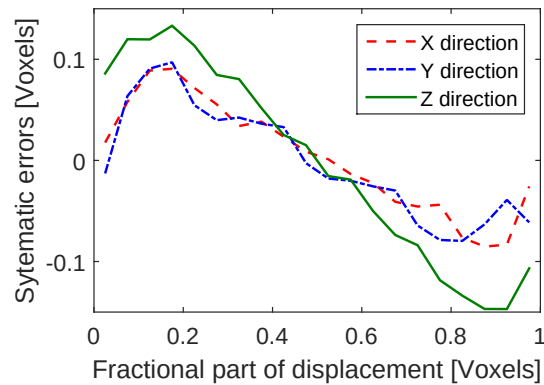
Figure 6.25: Systematic errors analysis for specimen PlasterF3
