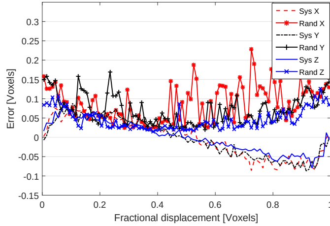
Figure 5.9: The systematic and random errors of selected well correlation points
