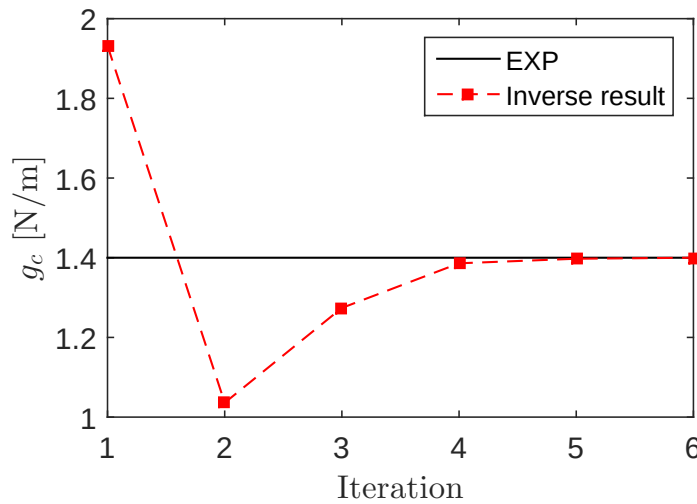
Figure A.6: Evolution of the parameter g_c during the inverse identification procedure (validation test).
