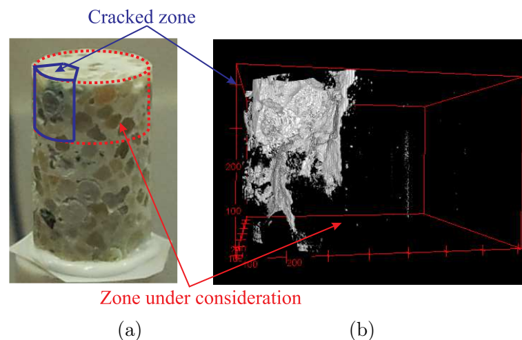
Figure 5.18: The segmentation of cracked areas in the subtracted image: 3D view of the damaged region
