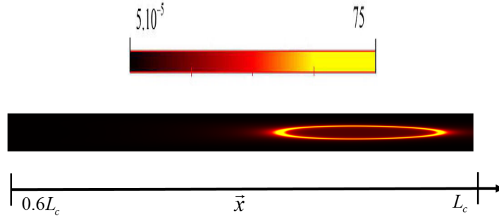
FIGURE 5.22: 2D field of the normalized gas-phase heat release rate at t = 1.65 t_{AI}
