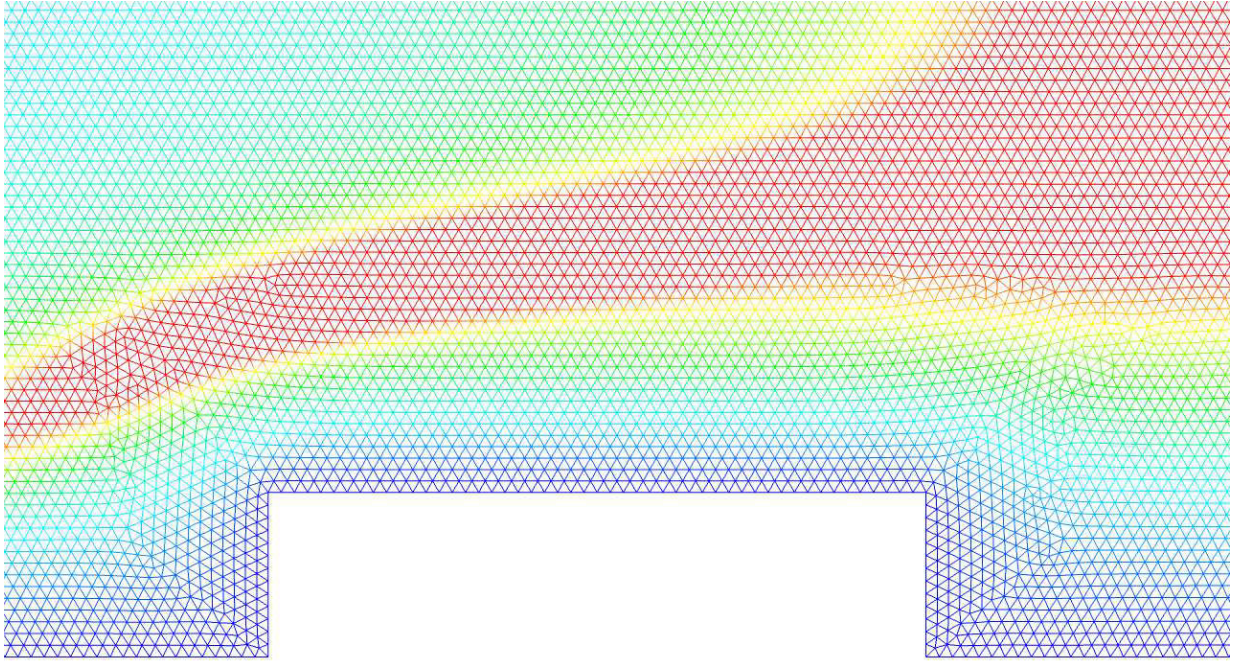
FIGURE 6.7: Spatial resolution of the gas-phase heat release rate near an obstacle
