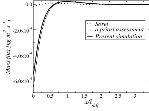
(A) Mass fluxes for CO_2 species
