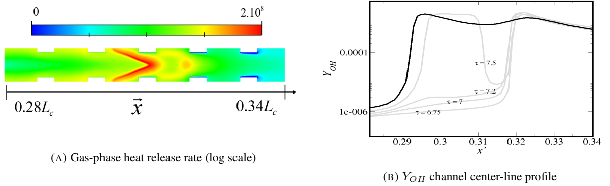
FIGURE 6.15: Propagation dynamic for the OS case at t = 7.75 t_{AI}
