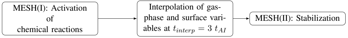
FIGURE 5.5: Summary of the meshing strategy, t_{interp} and t_{AI} respectively stand for the interpolation time and the physical time at which chemical reactions are activated.
