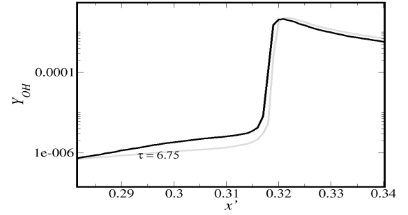
(B) Y_{OH} channel center-line profile
