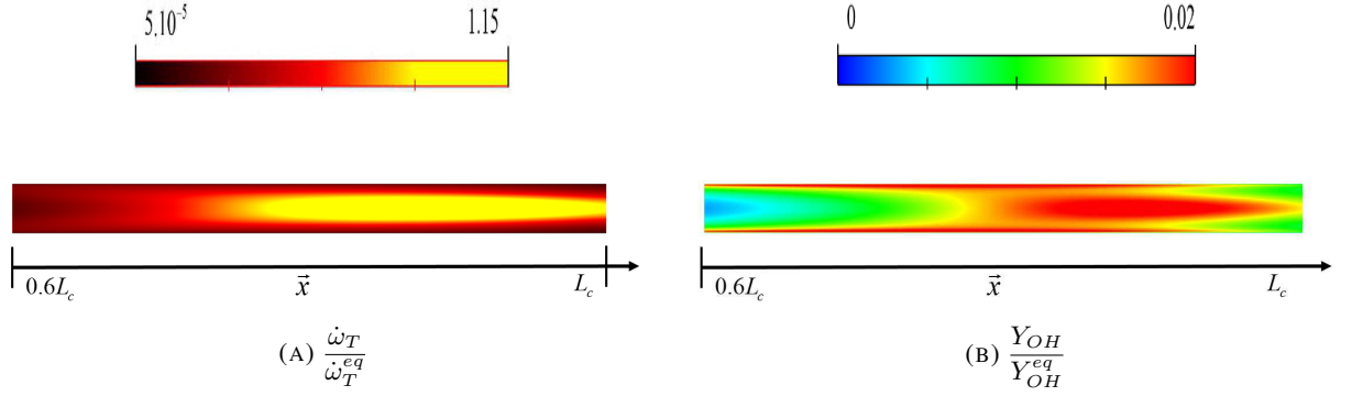
FIGURE 5.21: 2D Normalized gas-phase heat release rate (left) and OH concentration maps (right) at t = 1.5 t_{AI}
