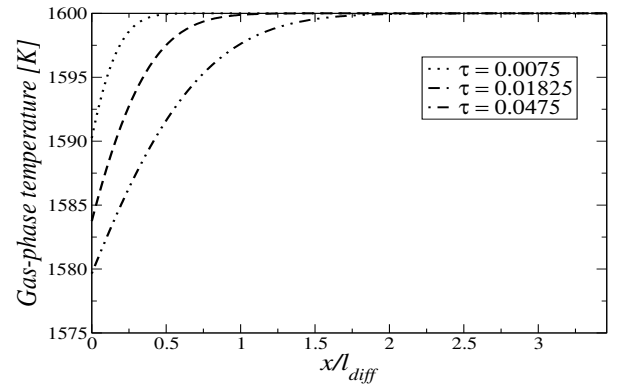
(B) Gas-phase temperature
