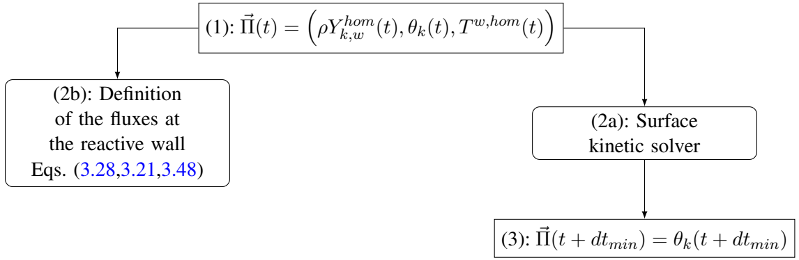
FIGURE 3.7: Coupling AVBP with the surface kinetics solver and boundary flux correction
