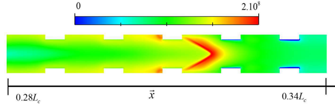
FIGURE 6.11: Propagation dynamic for the OS case at t = 6.75 t_{AI} : Gas-phase heat release rate (log scale)
