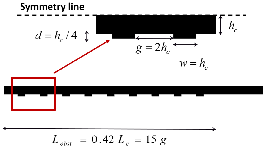
FIGURE 6.3: Schematic of the catalyst channel with cavities
