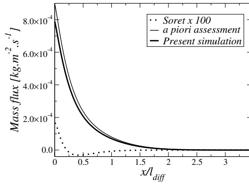
(E) Mass fluxes for CO species
