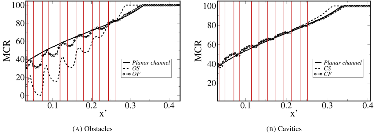
FIGURE 6.9: MCR for both types of Pt -coating : obstacles vs. cavities
