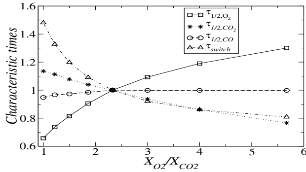
FIGURE 4.16: Characteristic times versus initial molar ratio (X_{O_2}/X_{CO_2})|_{t=0} . The case (X_{O_2}/X_{CO_2})|_{t=0} = 2.33 is taken as a reference
