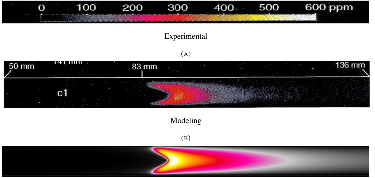
FIGURE 5.8: 2D OH concentration maps for case (c)
