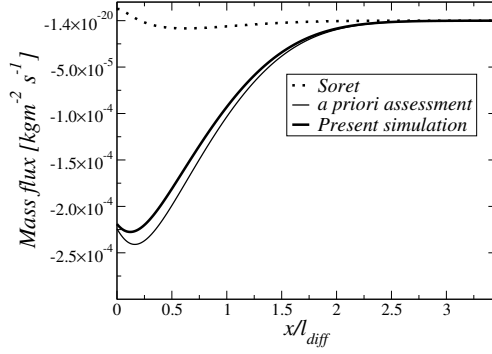
(C) Mass fluxes for O_2 species
