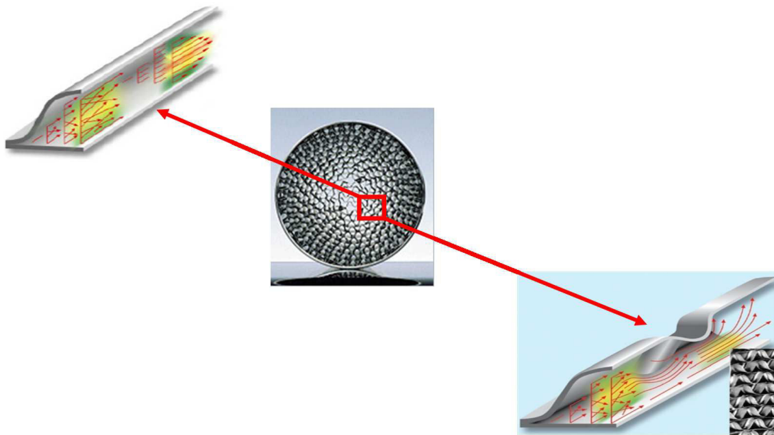
FIGURE 1.4: Introduction of a transfer promoter in the shape of a semi-spherical rib on the wall of a monolithic catalyst [5]
