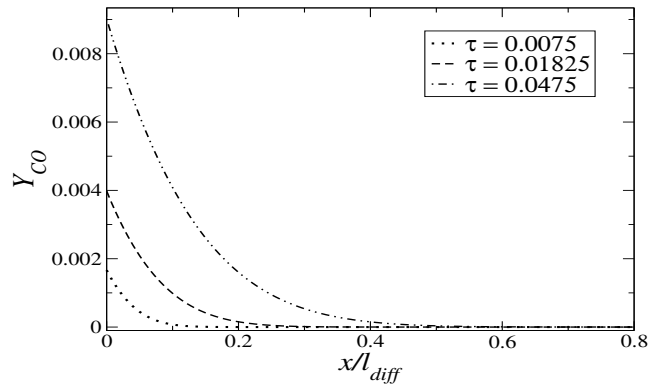
(C) Gas-phase CO profile
