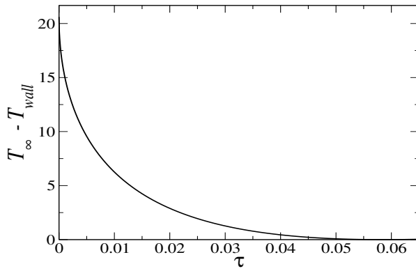
(A) Wall temperature
