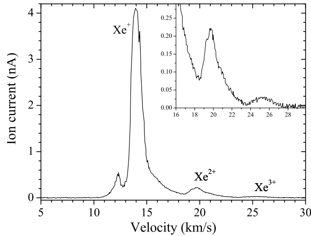
Figure 4.5: E \times B probe measurement 40 cm downstream of the PPI exit plane, under operation at 200 V and 1.0 mg/s of xenon. A small extra hump is seen before the main Xe^+ peak, and cannot be explained as of yet. This structure was also observed in previous works 16 .
