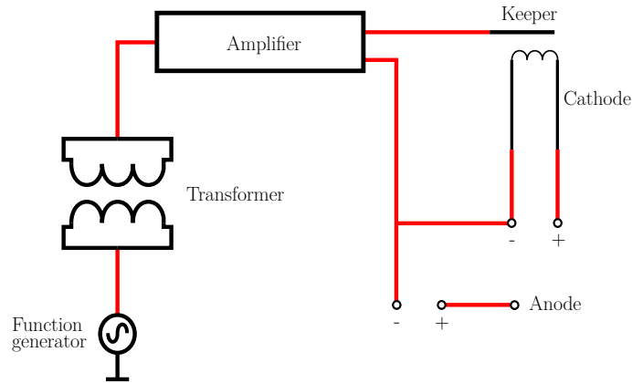
Figure 1.3: Electrical set-up of the keeper modulation.
