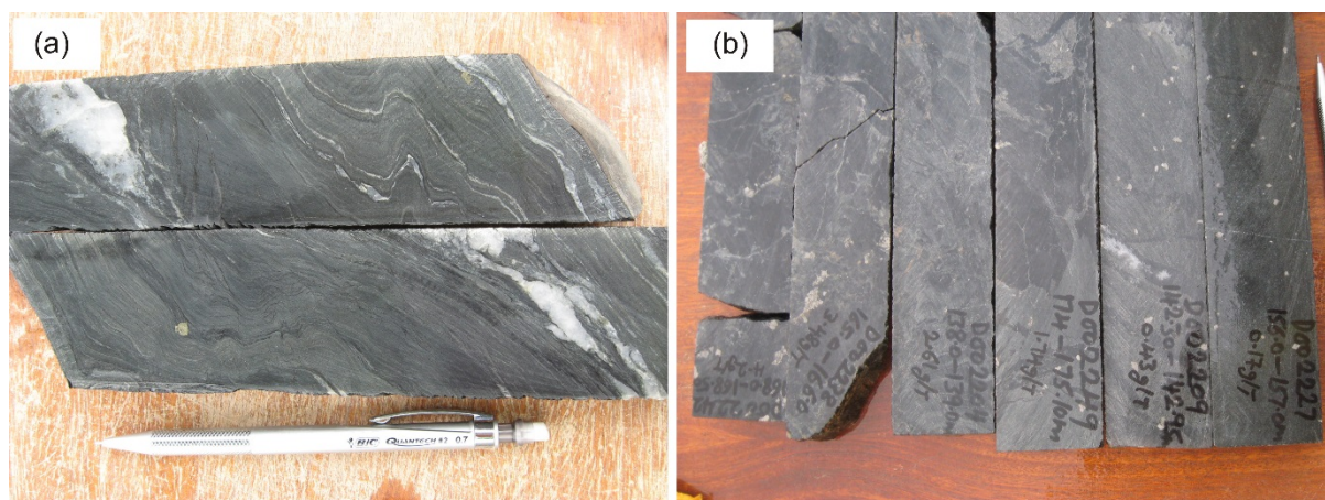
Fig. 6.2. Drill core of sediments in the Wa-Lawra belt (a) borehole showing graphitic shale deformed in a ductile fashion showing folding (b) borehole showing volcanoclastic rock affected by brittle deformation (brecciation).
