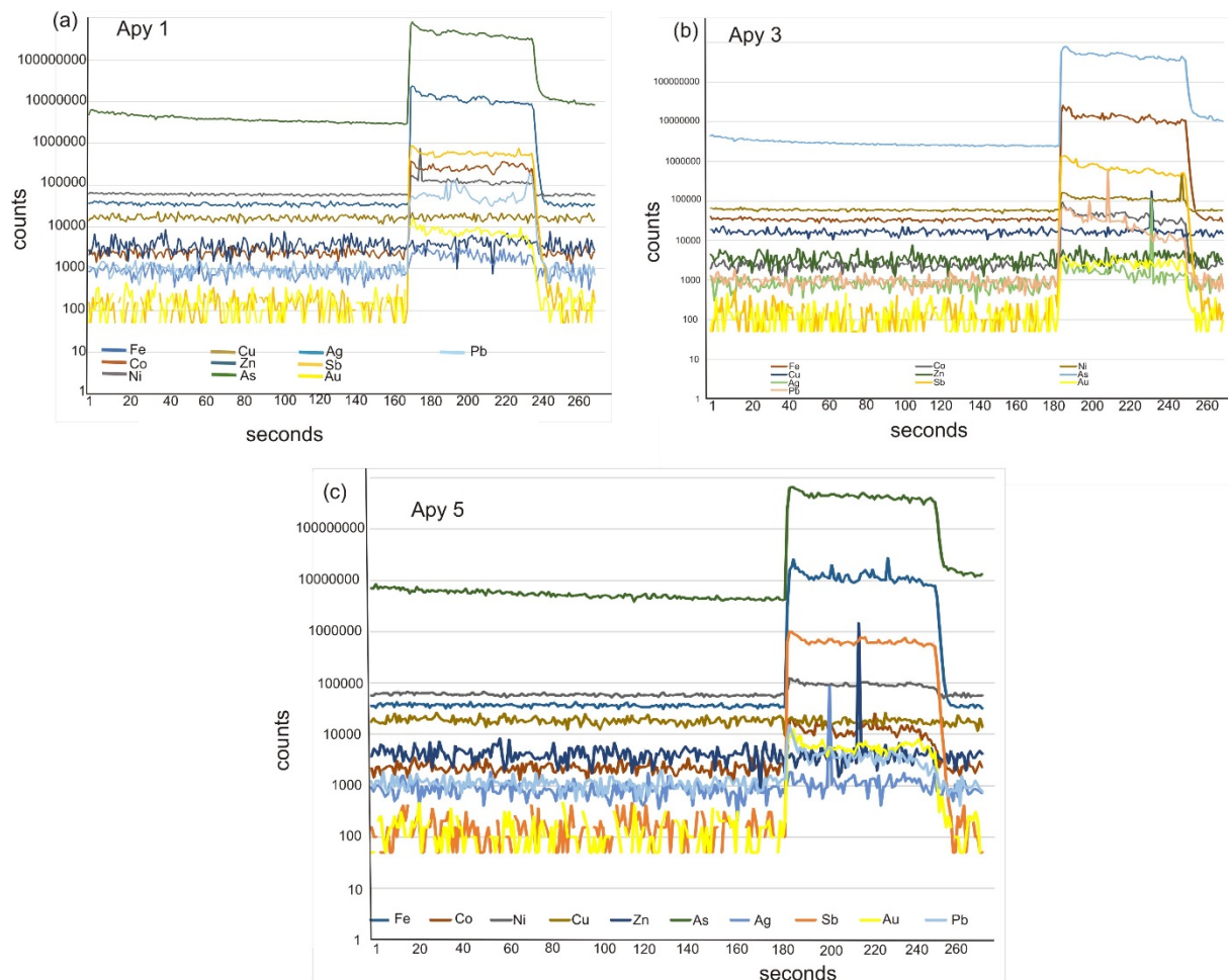
Fig. 4.16. Representative time-resolved depth spectra for arsenopyrite analysed within the Kunche deposit indicating the occurrence of gold and other element. Fe and As exhibits flats responds which is typical of major elements in arsenopyrite. The parallel trends of Au and Ag suggest they formed as nanoparticles or in solid solution.
