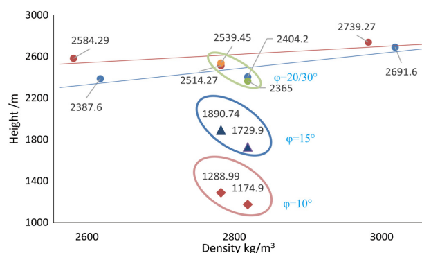
Fig. 10. Relief influenced by host rock friction angle and density contrast under compressional boundary conditions. A representative point at the faults' intersection (point O), as well as the maximum uplifted height of each model. Topographic height respectively increases by 200 m and 300 m at point O when increasing by 200 \text{ kg/m}^3 the host rock density. Topographic height when using host rock friction angles of 30^\circ or 20^\circ produce similar heights (elliptic domain in light green in figure (d)). Setting a friction angle to 15^\circ and 10^\circ (respectively covered by the blue and light red ellipses), drops the topography by about 600 m. In all experiments, the contrast in density has a smaller effect on topography than the host rock friction angle. (For interpretation of the references to colour in this figure legend, the reader is referred to the web version of the article.)
