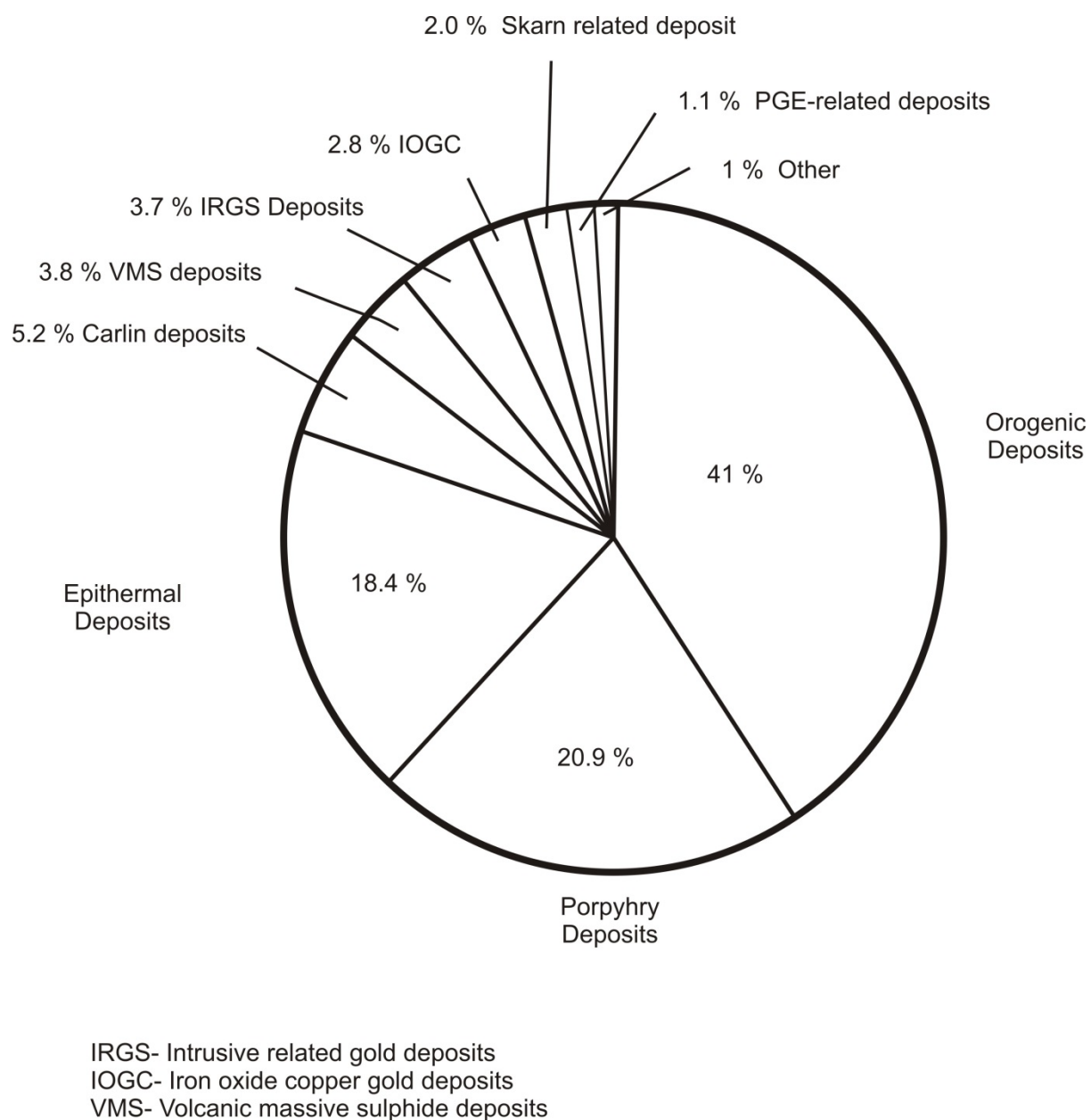
Fig. 1.1. Pie chart showing the cumulative gold endowment through time in the various gold deposit types in the world as at December, 2013 (Lipson, 2014)
