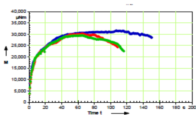
Figure. 5.6. Torque versus time curves obtained during vane tests mix-design C1 (yield stress of 20kPa)
