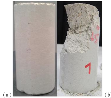
Figure 6.18. Typical compression failure modes of cement mortar type C1 without fiber: (a) extruded plain mortar; (b) after static loading.
