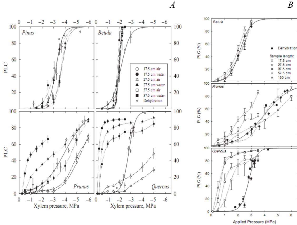
Figure 18. Effects of sample length on xylem VCs obtained with Cavitron and air-injection techniques on different segment lengths.
