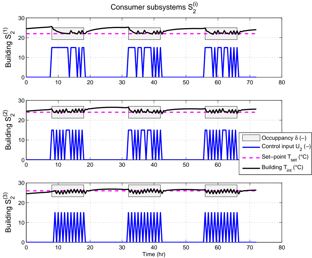
Figure 5.3: Consumer controllers performance.
