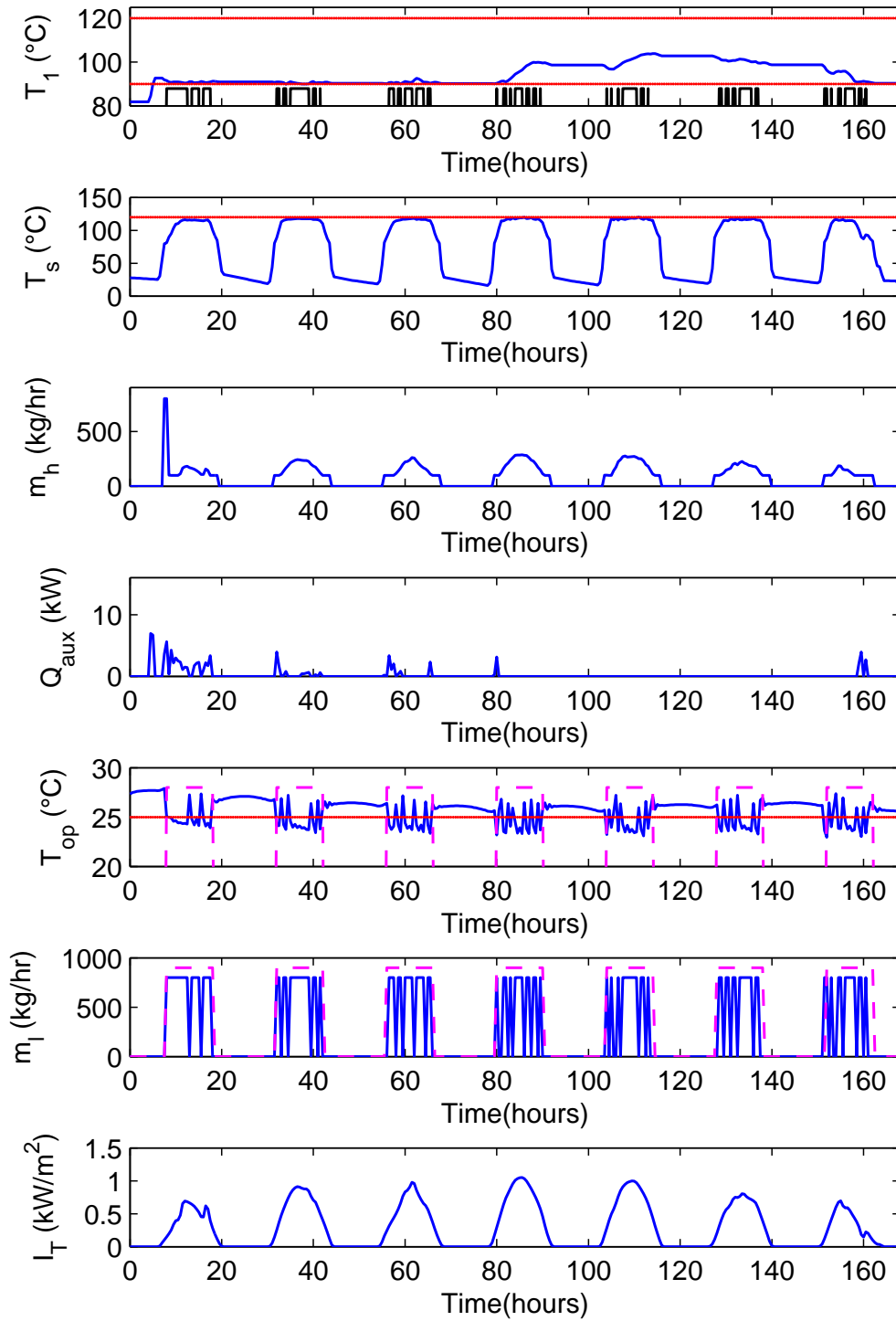
Figure 6.12: MPC strategy considering T_1 = 82 °C, T_{op} = 27 °C and b = 3 .
