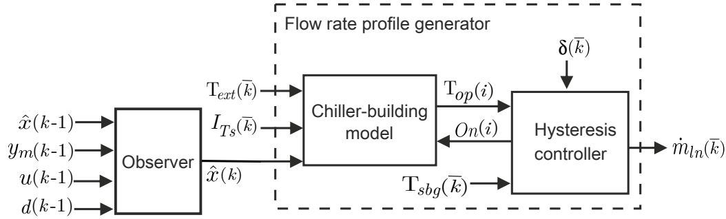
Figure 6.6: Consumer controller structure. Observer inputs: previous state vector \hat{x}(k-1) , measured building operative temperature y_m(k-1) , previous control signal u(k-1) and disturbances d(k-1) . Chiller-building model inputs: exterior temperature T_{ext}(\bar{k}) over the prediction horizon, total radiation of the building south-oriented wall I_{T_s}(\bar{k}) over the prediction horizon, current estimated state vector \hat{x}(k) and current control signal calculated by the hysteresis controller O_n(i) . Hysteresis controller inputs: occupancy profile \delta(\bar{k}) over the prediction horizon, current building operative temperature calculated by the model T_{op}(k) and building set-point T_{sbg}(\bar{k}) over the prediction horizon. The output of the hysteresis controller is the generated energy demand profile \dot{m}_{ln}(\bar{k}) over the prediction horizon.
