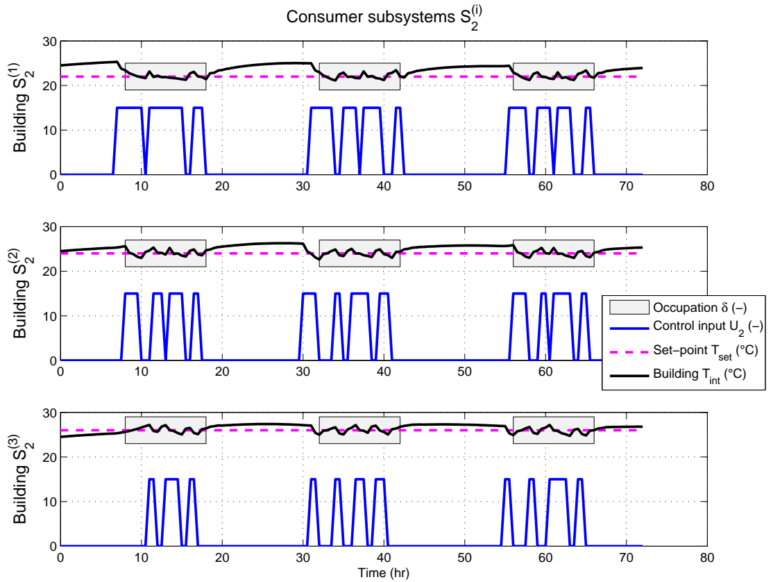
Figure 5.7: Consumer controllers behavior when N_h = 8 and b = 3 .
