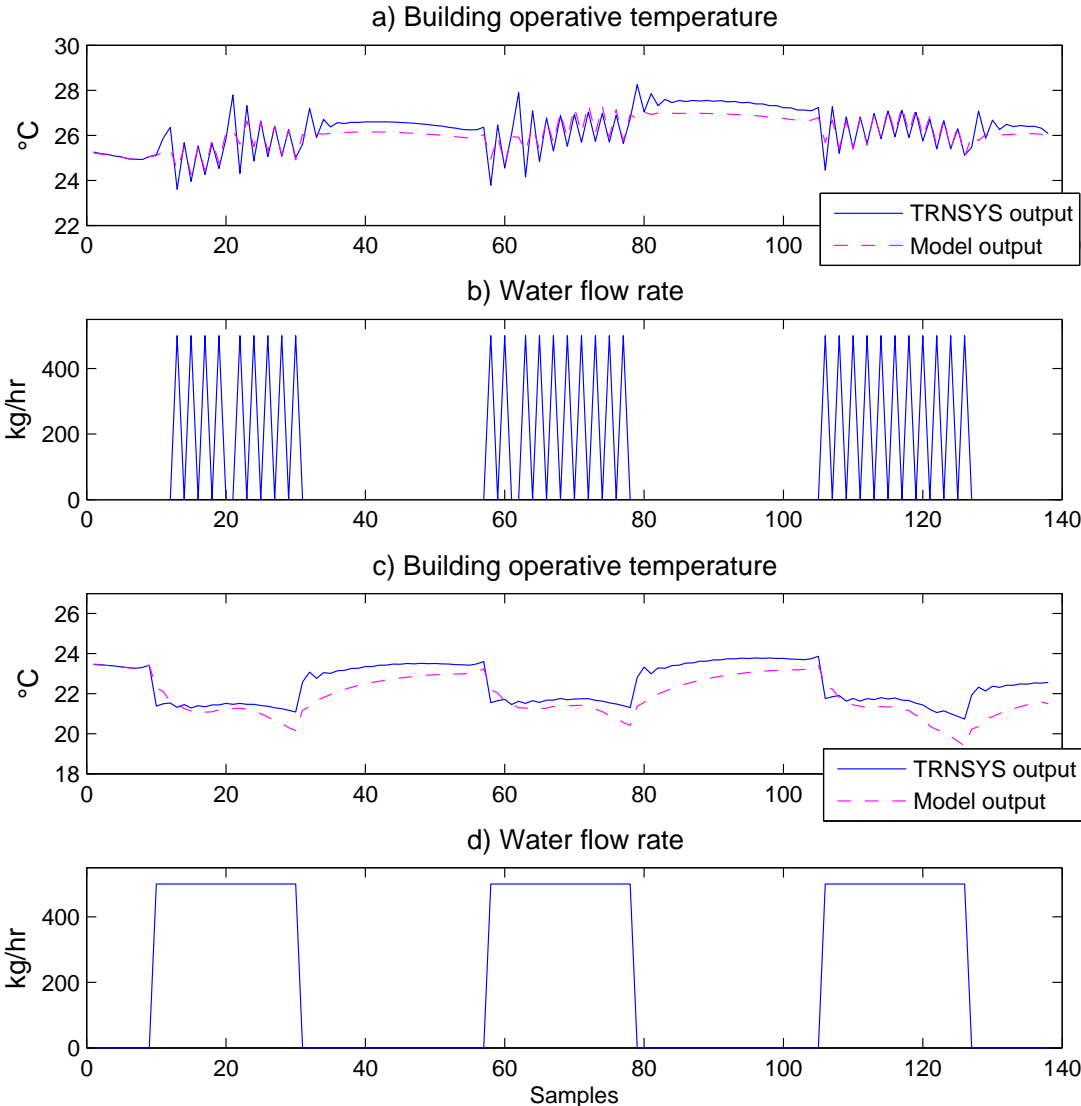
Figure C.2: Model comparison.
