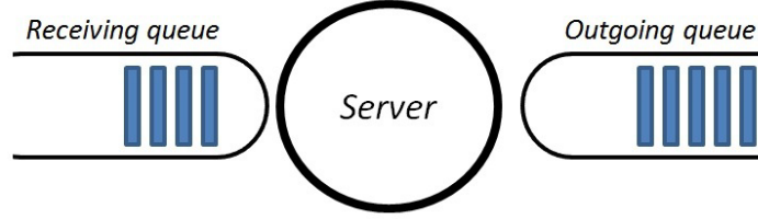
Figure 3.1: Node model
