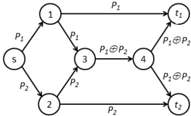
Figure 1.1: Butterfly example
