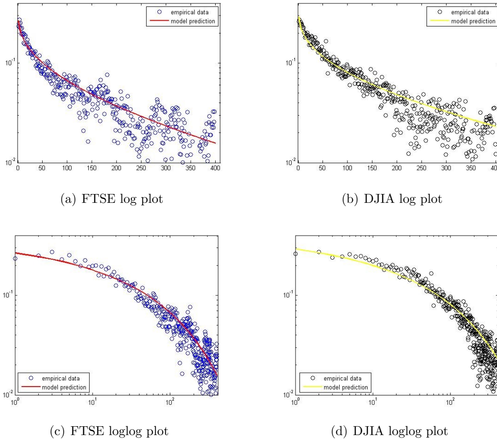
Figure 5.4: Volatility autocorrelation
