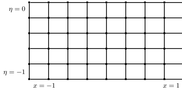
Figure 6.1: Partition of \Omega with N_x = 8 and N_\eta = 5 .
