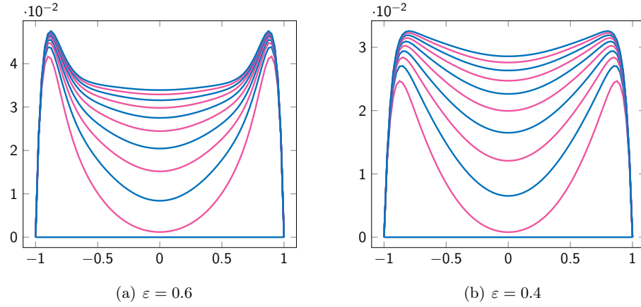
Figure 6.4: Approximate solution u_{\tau,h} for f(x) = x^8 + 0.1 with \lambda = 1 and different \varepsilon > 0 .
