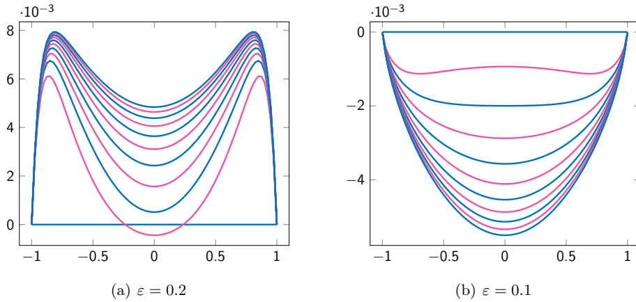
Figure 6.5: Approximate solution u_{\tau,h} for f(x) = x^8 + 0.1 with \lambda = 1 and \varepsilon \in \{0.1, 0.2\} .
