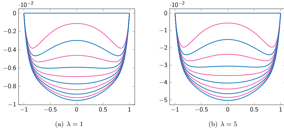
Figure 6.9: Approximate solution u_{\tau,h} to the small-aspect ratio model with u_* \equiv 0 for f(x) = x^8 + 0.1 and different \lambda .
