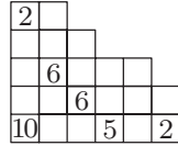
FIGURE 2.4. Illustration pour \mu = (6, 6, 5, 3, 2) .
