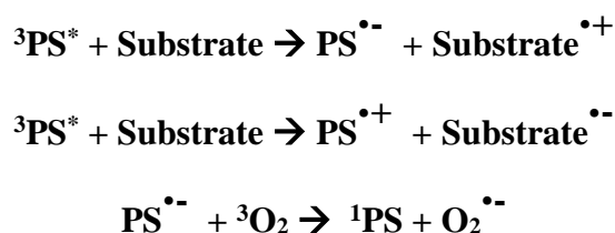
Equation 2: Primary photochemical reactions of photosensitive compounds.
