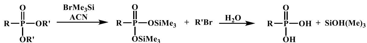
Figure 87: Cleavage of phosphonate diesters to phosphonic acid using BrMe 3 Si.
