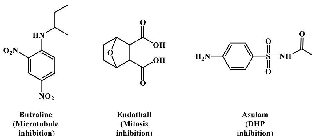
Figure 60: Examples of non-selective herbicides acting on cell division.
