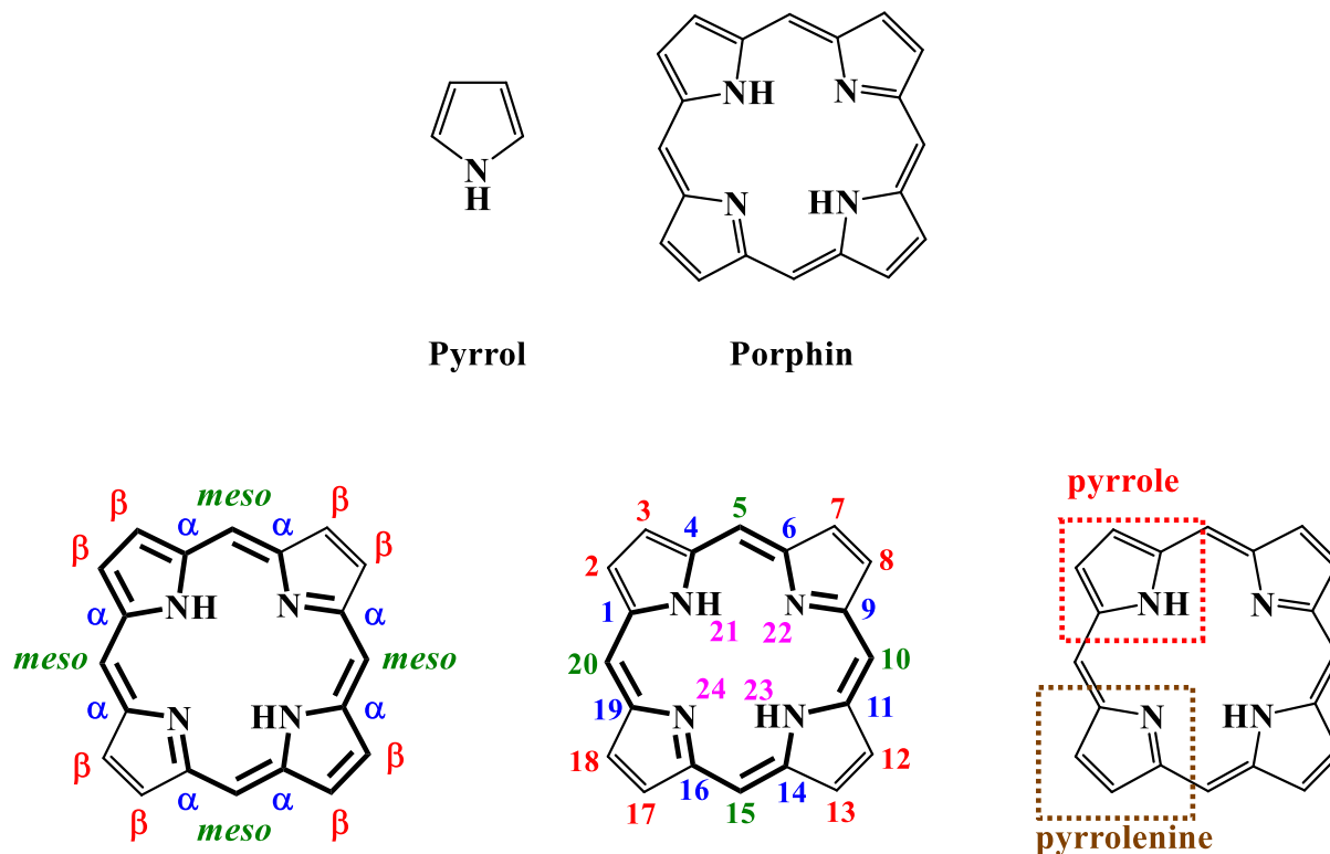
Figure 7: Numbering and naming of the porphyrin positions by means of porphyrin core according to the IUPAC (International Union of Pure and Applied Chemistry).
