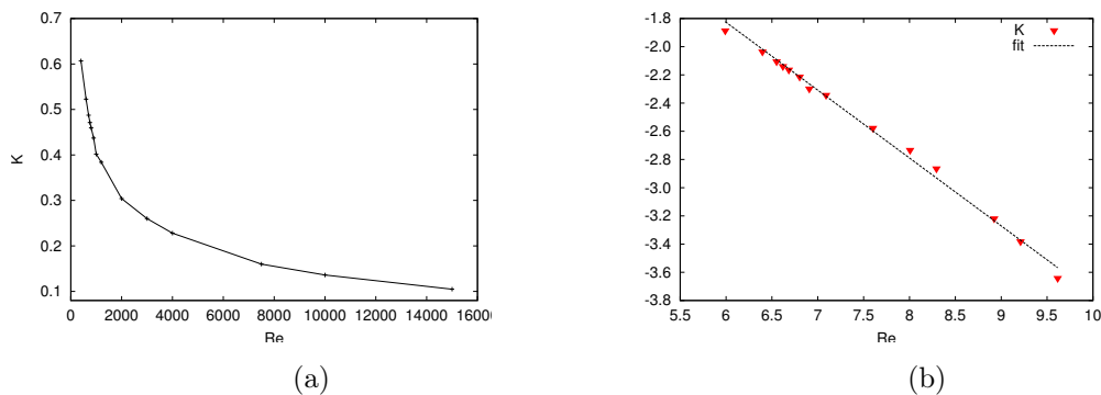
Figure 4.25: (Color online) Total (time-averaged) kinetic energy K in the precession frame as a function of the Reynolds number R_e : (a) in linear scale and (b) in log-log scale with the fit R_e^{-0.48} .
