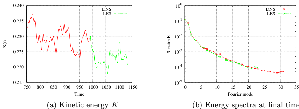
Figure 4.40: Comparisons of DNS and LES results at R_e = 4000 . (a) Evolution of total kinetic energy K(t) (zoom of figure 4.24b), (b) kinetic energy azimuthal spectra at final time as a function of the Fourier modes ( 0 \leq m \leq 31 with DNS and 0 \leq m \leq 23 with LES).
