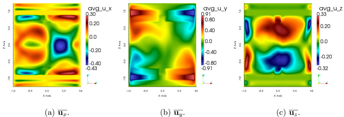
Figure 4.10: Representation of the mean Cartesian components of the velocity field in a plane ( x, z ) at R_e = 1000 .
