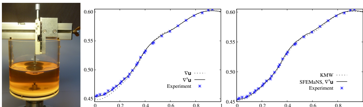
Figure 5.5: (a) Experimental set up with the needle measuring the free surface elevation (courtesy of L. Martin Witkowski); (b) Free surface elevation by SFEMaNS with \nabla\mathbf{u} (dotted line) and \nabla^s\mathbf{u} (solid line) and experimental results (symbol *); (c) Numerical solution by SFEMaNS with \nabla^s\mathbf{u} (solid line), numerical (KMW, dotted line) and experimental (symbol *) results by [53].
