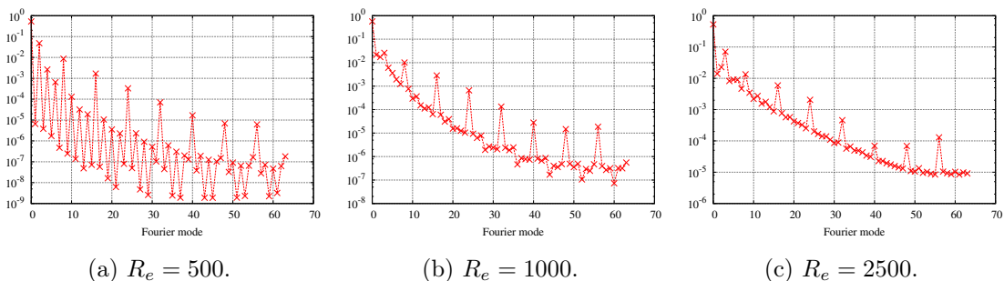
Figure 4.14: Modal kinetic energy of each Fourier mode ( 0 \leq m \leq 63 ) at final time for R_e \in \{500, 1000, 2500\} .
