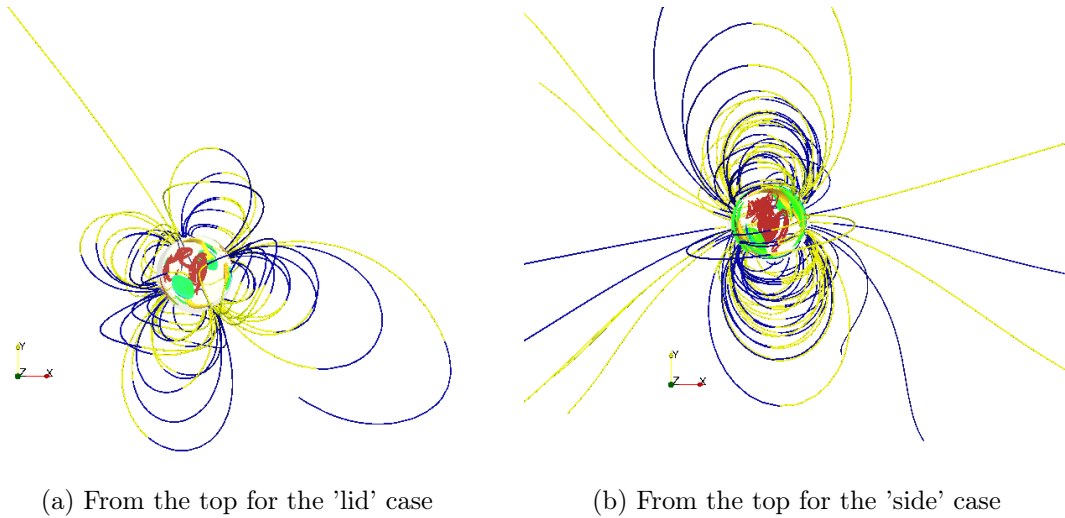
Figure 4.35: Conducting walls: Snapshots at (a) R_e = 1200, R_m = 1000 for the 'lid' case and (b) R_e = 1200, R_m = 900 for the 'side' case showing vorticity field lines (red lines inside the cylinder) and magnetic field lines colored by the axial component [yellow (blue) for positive (negative) h_z component].
