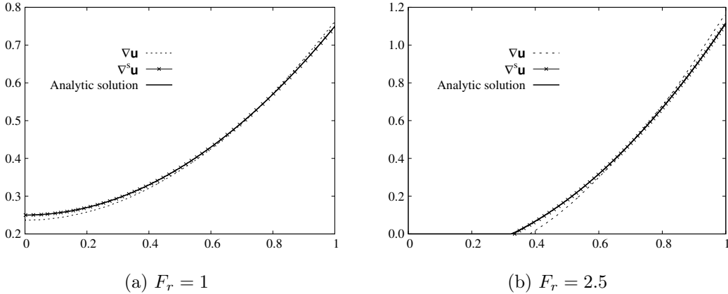
Figure 5.3: Free surface elevation \zeta(r) for the Newton's bucket configuration: analytical solution (solid line), numerical solution with \nabla\mathbf{u} (dotted line), numerical solution with \nabla^s\mathbf{u} (symbol \times ): (a) wet case, (b) dry case.
