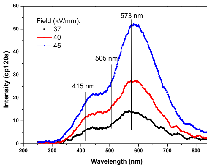
Figure 3-19 EL spectra of XLPE films under 50 Hz AC stress.
