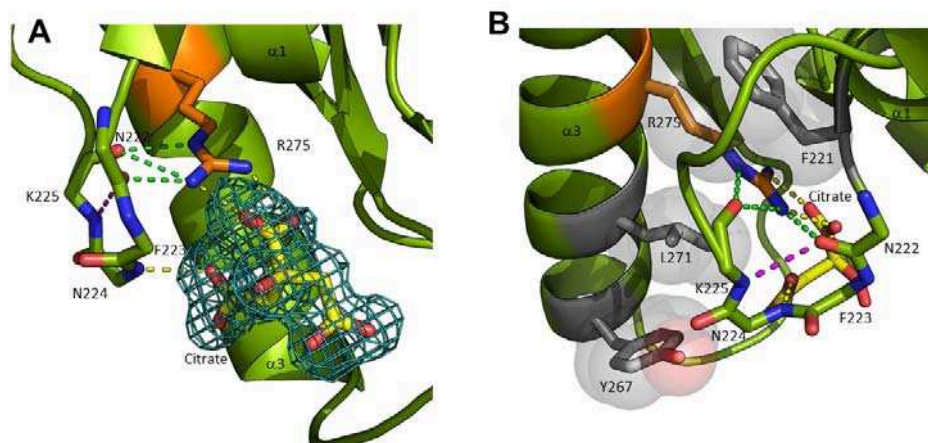
Figure 3. A. View of the citrate inside the binding site represented in stick mode and its electron density in the omit map contoured at 3\sigma . Conserved arginine 275 is represented as orange stick while the backbone of \beta -turn \alpha 1 - \beta 2 is represented as green stick. Interactions between the citrate and C-KpOmpA are represented as yellow dashed lines and interactions between R275 sidechain and the backbone are shown as green dashed lines. Interaction between CO of N222 and NH of K225, residues i and i+3 of \beta -turn \alpha 1 - \beta 2 respectively, is represented as magenta dashed line. B. Side view of the citrate in the binding site. Conserved hydrophobic residues F221, L271 and Y267 are represented as sticks and transparent grey spheres.
