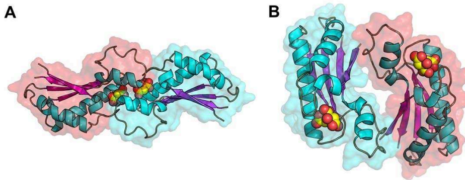
Supplementary Figure S3. A. Dimer formed by the first interface of dimerization involving the loop \alpha 1 - \alpha 2 , loop \beta 2 - \alpha 3 and the helix \alpha 4 . B. Dimer formed by the third interface of dimerization and involving the strand \beta 1 and the series of \beta -turn from the bulge.
