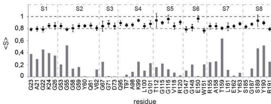
Figure 5. Histogram representation of amide bond order parameter (black box) per assigned residue (data in Supplementary Table S1). Grey bars represent the value of |( \cos^2\beta - 1 ) / 2| , where \beta is the angle the amide bond angle with respect to the long principal axis of the system (i.e. \beta -barrel), which is assumed to be closed to the principal axis of the rotational diffusion motion ( \beta values were computed from the known 3D structure of KpOmpA, pdb 2K0L).
