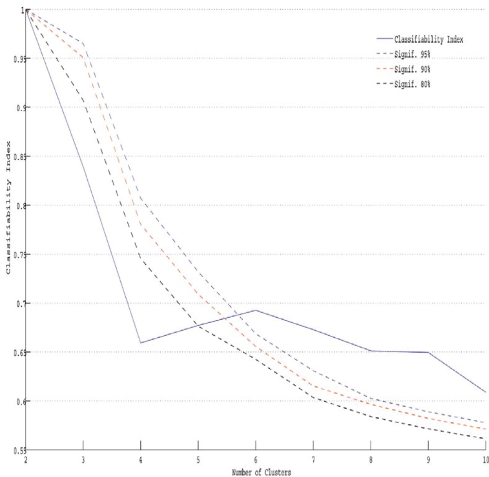
Figure 3.19 Classifiability index c as a function of the number of regimes k (solid line). The significance levels at 95%, 90% and 80% (dashed lines) are computed according to a first-order Markov process.
