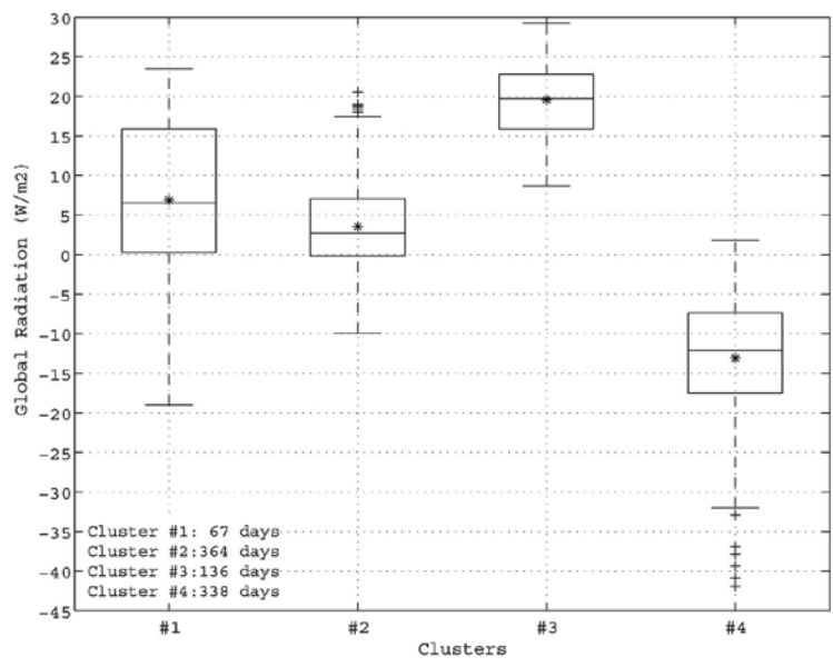
Figure 4.15 Box-and-whisker plots for the spatial average SSR anomalies amount for 4 clusters (intra-class variability) Nov 2004 to Apr 2005. The boxes have lines at the lower quartile, median and upper quartile values. Cluster sizes are labeled on the figure.
