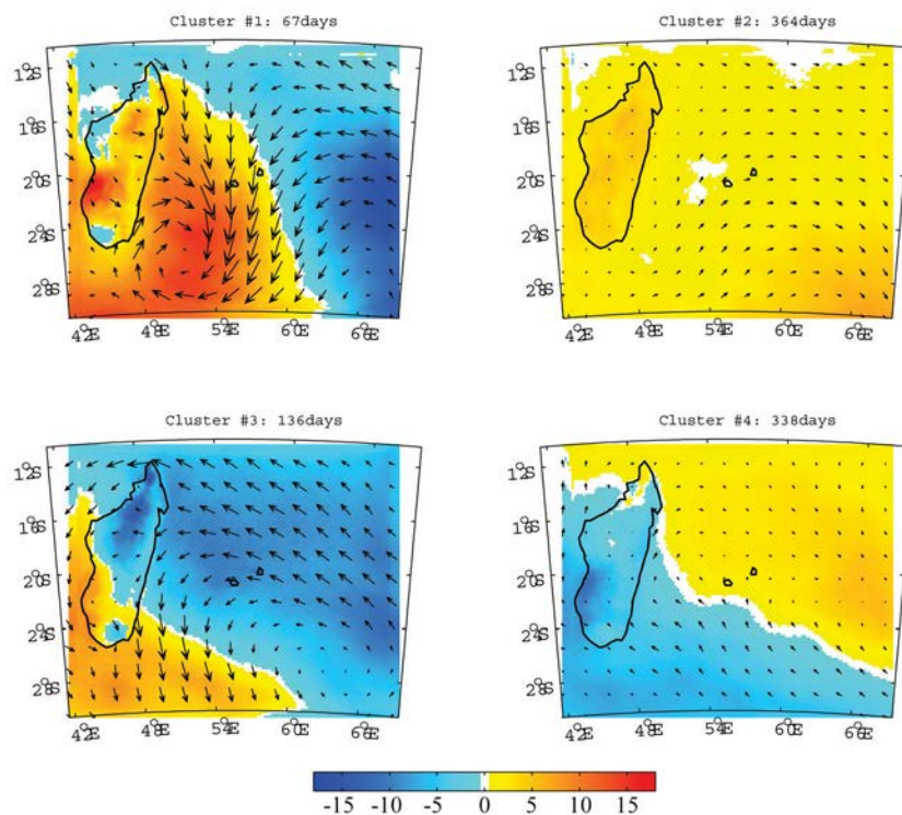
Figure 4.18 Spatial distribution of composite Q2-UV10 anomalies ( 10^{-4} \cdot \text{kg/kg} ; m/s) associated with the 4 clusters for Nov 2004 to Apr 2005. The number of days for each cluster is labeled on the figure.
