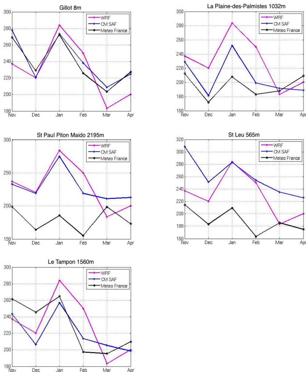
Figure 4.3 WRF simulated monthly means and CM SAF compared to Météo France data at 5 stations separately for austral summer 2004-2005 ( W/m^2 ).
