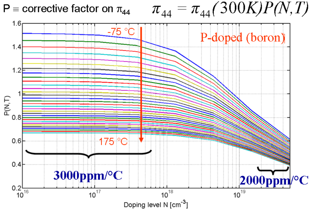
Figure 25: Piezoresistive coefficient variation with doping
