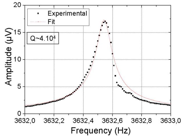
Figure 68: frequency response of an accelerometer in vacuum
