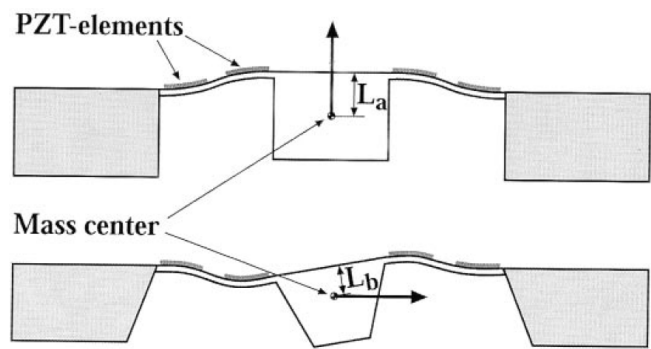
Figure 7: Three-axis accelerometer based on PZT detection [Kunz01]
