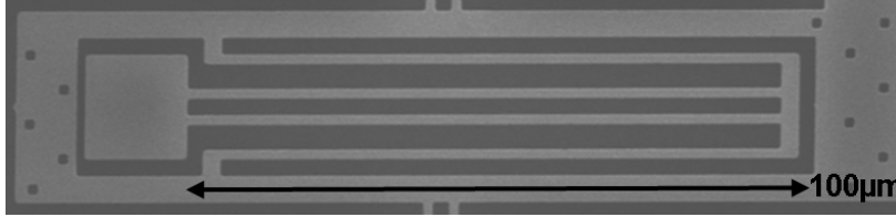
Figure 48: SEM image of a folded guiding spring
