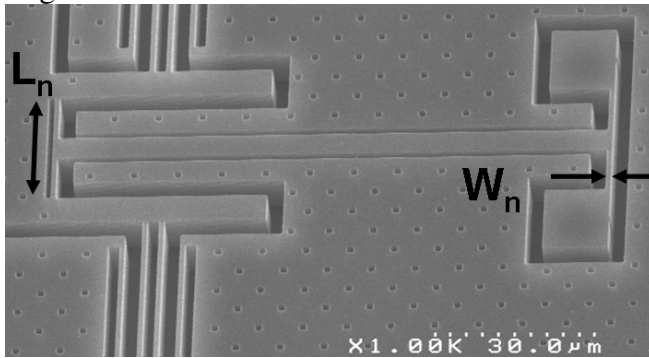
Figure 50: SEM image of an H-shape spring
