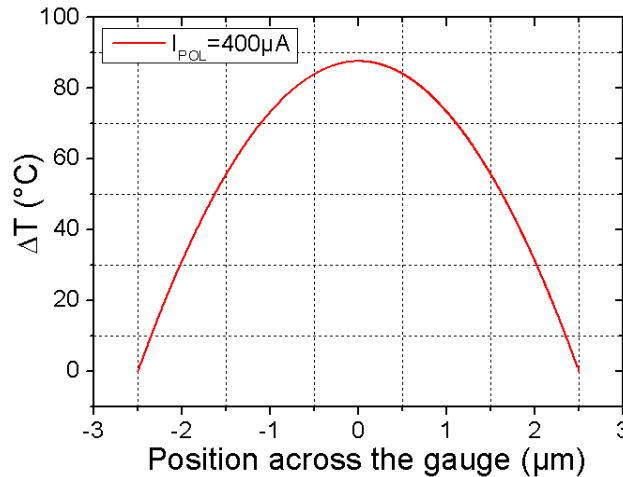
Figure 28: Temperature profile across the nanogauge ( I_{POL}=400\mu A )
