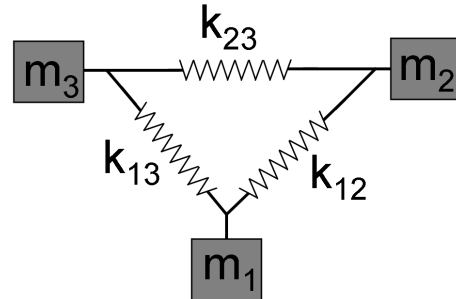
Figure 165: Scheme of springs in a \Delta geometry
