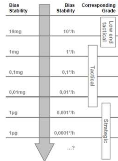
Figure 2: Bias stability requirements for accelerometer and gyroscopes depending on the application
