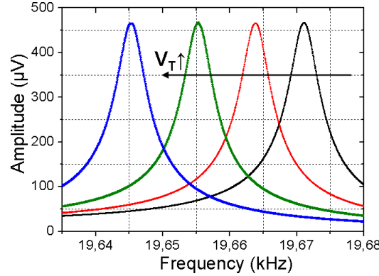
Figure 111: Experimental validation of the trimming electrode
