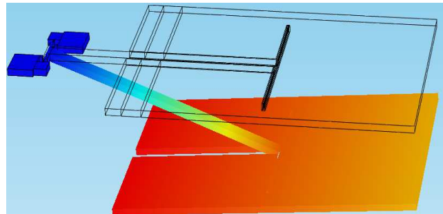
Figure 80: Detection Eigen mode (displacement field - frequency~2302Hz). In this case, a large stress is induced in the nanogauges
