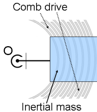
Figure 65: Top view of angular comb drive design
