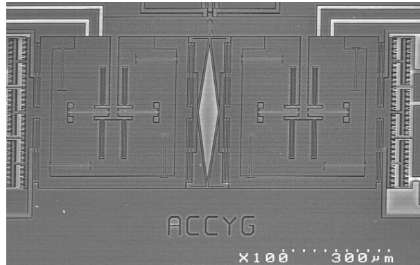
Figure 103: SEM picture of the fabricated gyroscope [Wal12]
