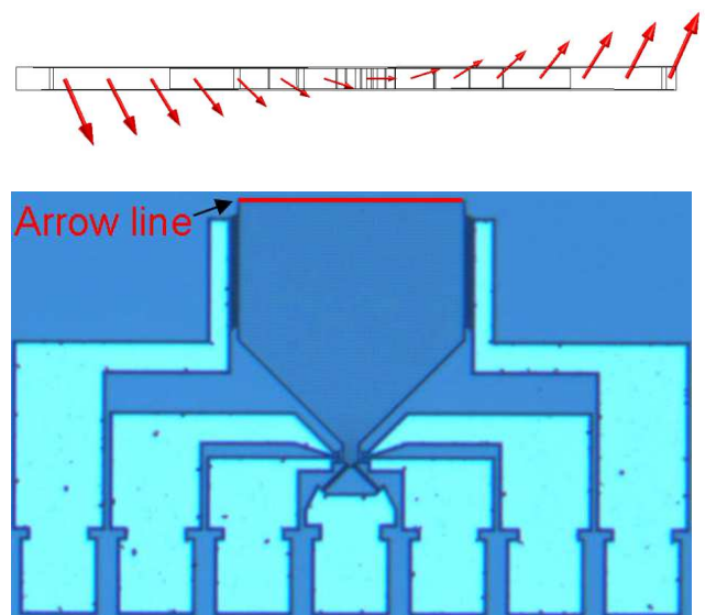
Figure 72: Simulated representation of the out-of-plane movement obtained
