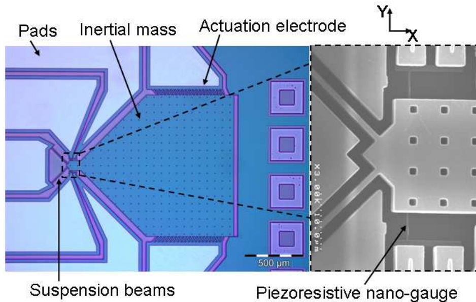
Figure 59: Top view of an in-plane accelerometer
