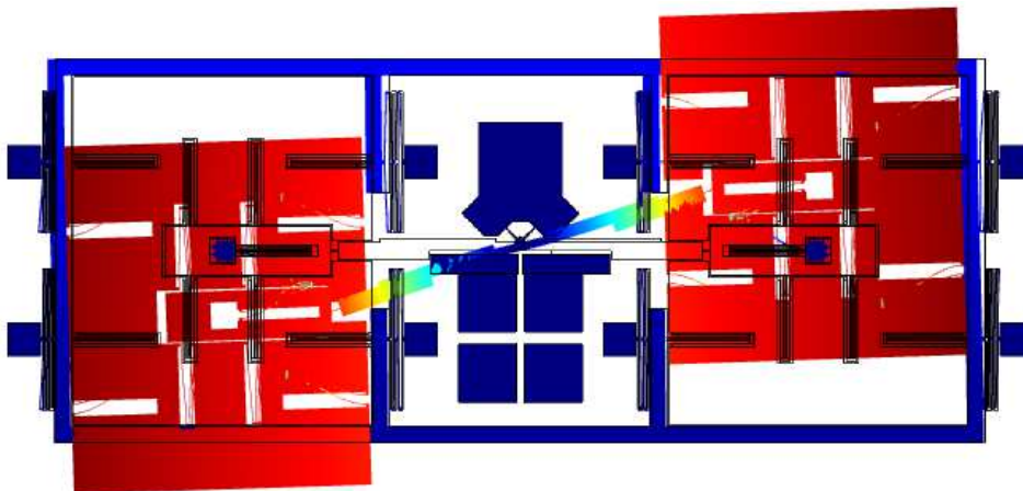
Figure 130: Sense mode of the coupled accelerometer-gyroscope (20.5kHz)
