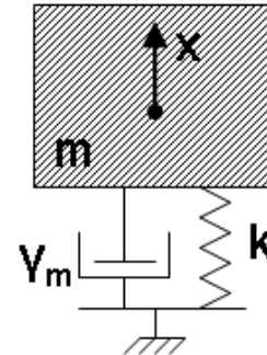
Figure 149: Equivalent mechanical scheme of a quasi-static sensor
