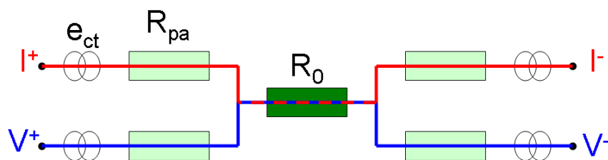
Figure 162: Four point measurement polarization scheme
