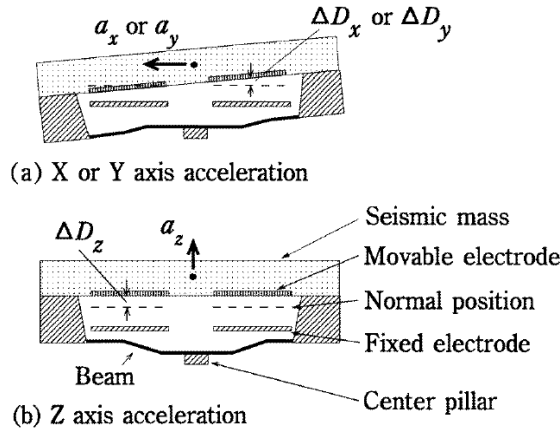
Figure 4: Implementation of capacitive three-axis accelerometer by [Min96]
