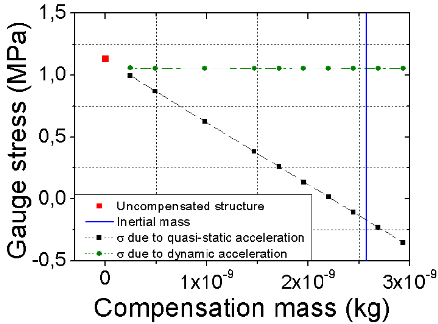
Figure 141: Simulated gauge stress due to mass compensation
