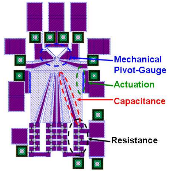
Figure 160: Top view of a damped accelerometer using circular comb drive
