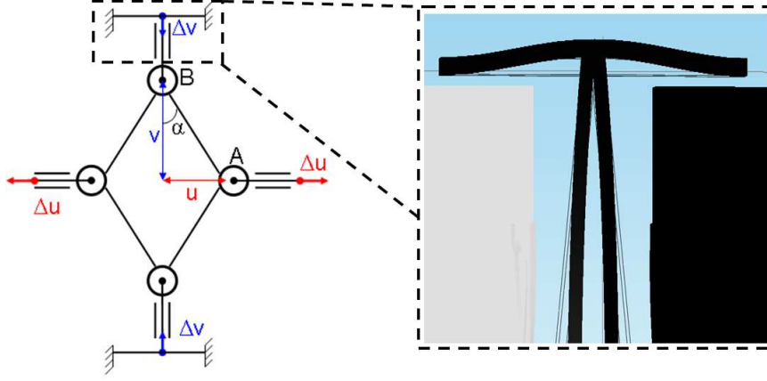
Figure 53: Modelling of the anti-phase mode
