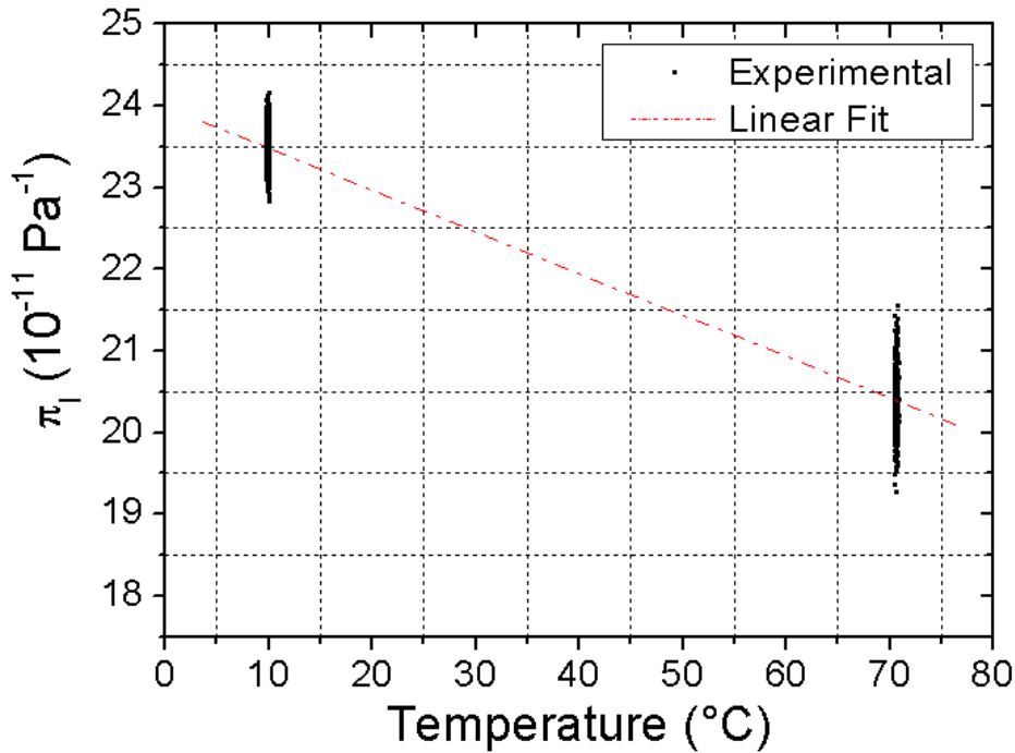
Figure 24: Piezoresistive coefficient for different temperatures
