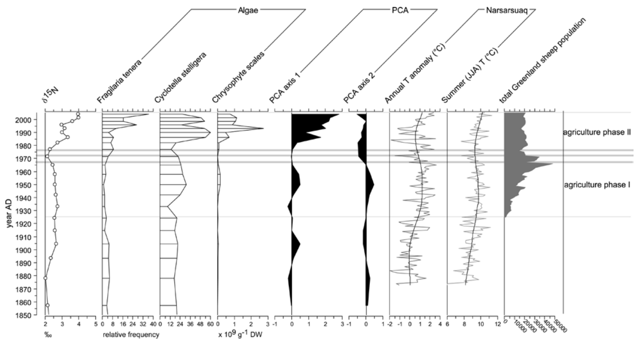
Fig. 5.7 Stratigraphic diagram showing variations in \delta^{15}\text{N} , Fragilaria tenera , Cyclotella stelligera , and chrysophyte scales, the synthesis PCA axes 1 and 2, the mean annual temperature anomaly from the Narsarsuaq meteorological station, June, July and August (JJA) temperature from Narsarsuaq, and the total population of sheep in Greenland for the last 150 years. Grey bands mark the recent documented sheep population crises.
