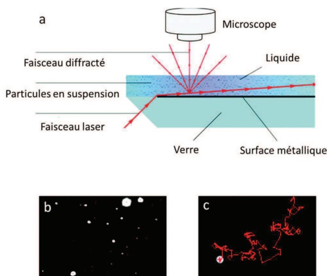
Figure 56. Principe du Nanosight
