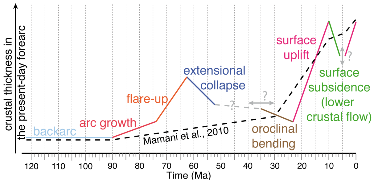
Figure VI. 1: Diagram showing the schematic evolution of crustal thickness in the present-day forearc of southern Peru as proposed in this dissertation (in color). The evolution based on geochemical data proposed by Mamani et al. (2010) is reported for comparison (black dotted line). No vertical scale.
