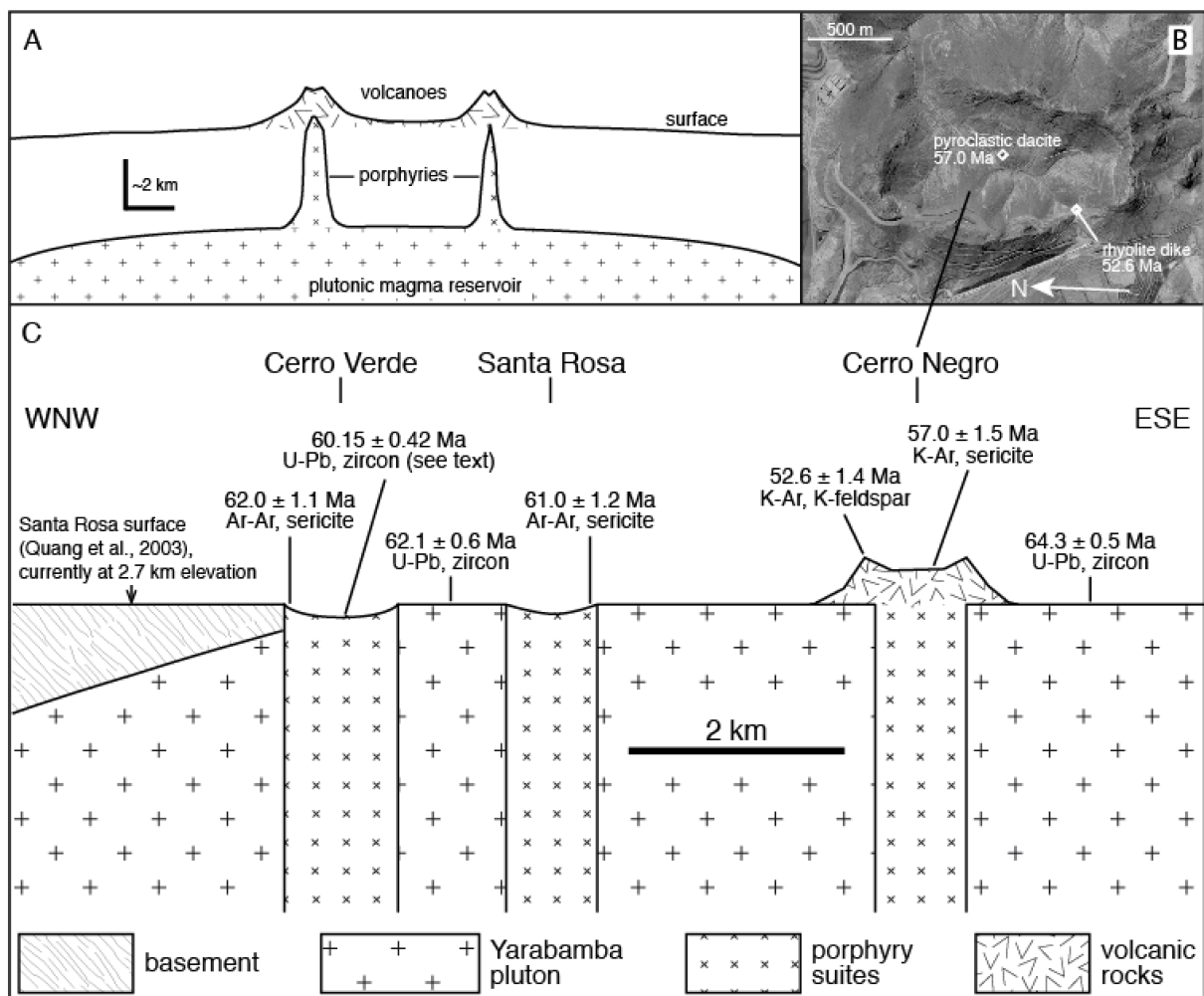
Figure III.6: A. Cartoon cross-section illustrating the emplacement model for porphyries after Sillitoe (2010). B. Satellite image of the Cerro Negro paleovolcanoe (16.548°S–71.556°W) and localization of the different disponible ages. C. Sketch of the geological relationships in the Cerro Verde mining district. No vertical scale. See references for ages in Table III.1
