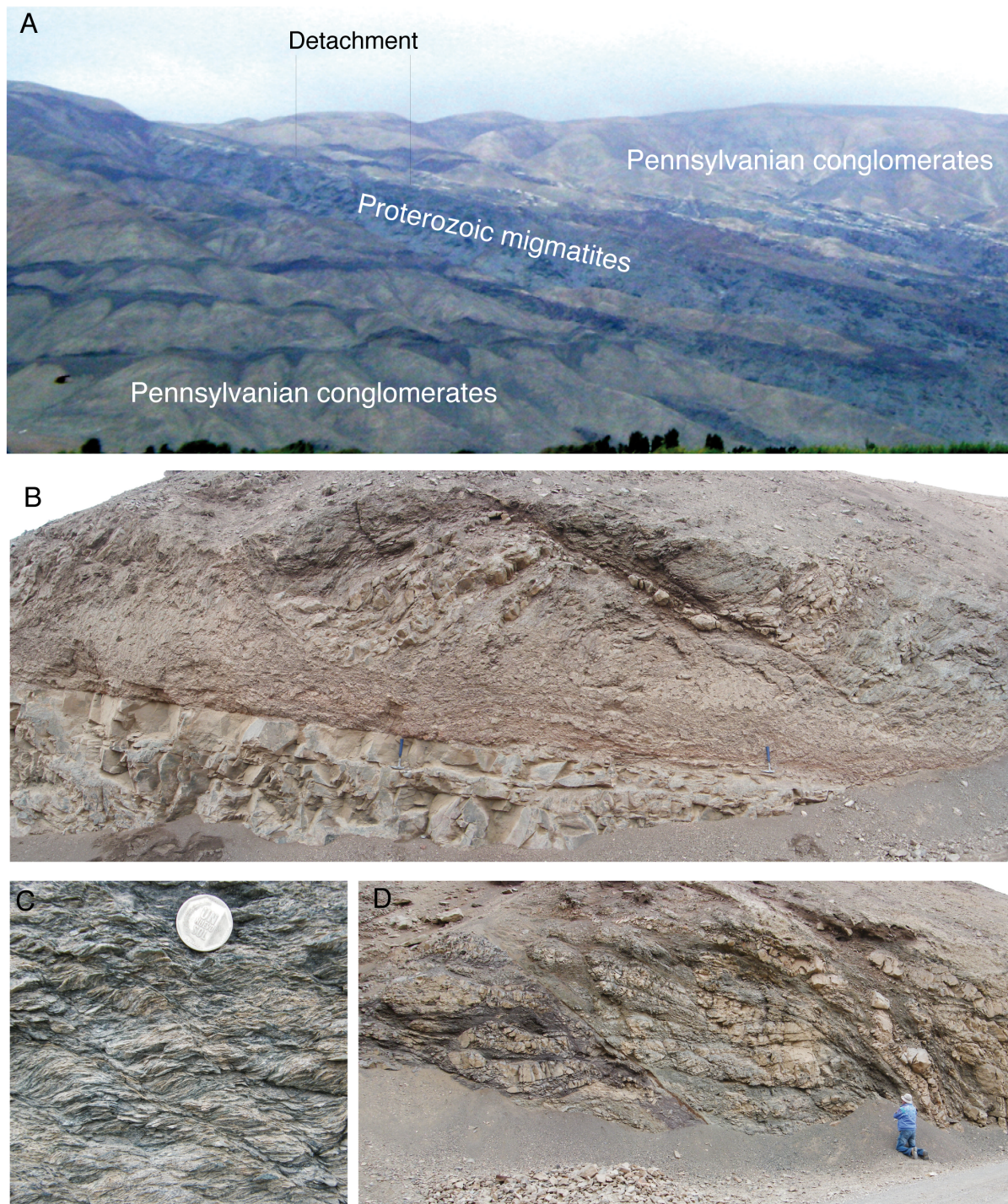
Figure I.6: Evidences of margin extension during the Paleozoic: the Ocoña detachment. A: The detachment fault creates a structural slab in the landscape, well expressed in the Ocoña valley. B: The Ocoña detachment fault zone (hammers for scale); C: C-S structures in the Proterozoic migmatites few meters under the detachment fault; D: Extensional deformation in the Pennsylvanian deposits.
