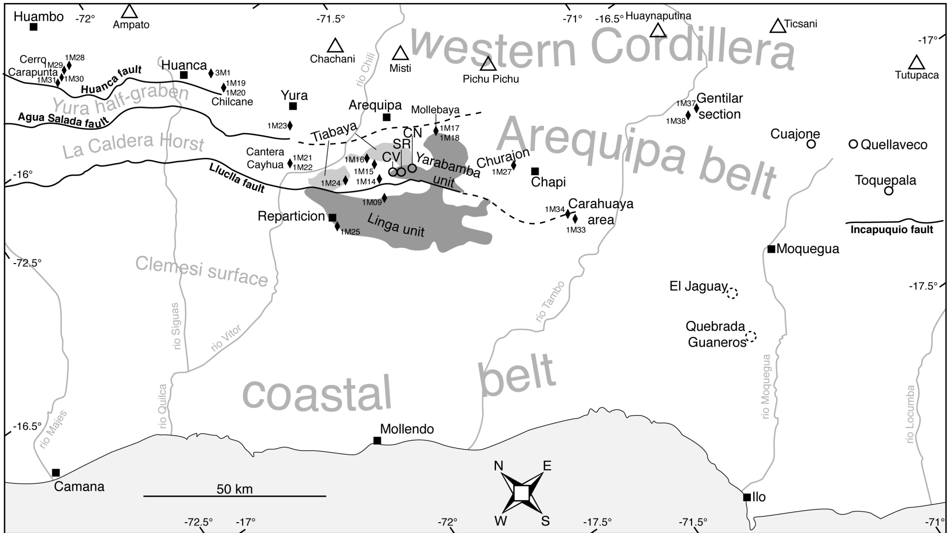
Figure III.4: Simplified map of the forearc of southern Peru showing the main locations names used in the text. Names of faults are in bold and located on their downwarped side. Black squares: cities; open triangles: volcanoes; black diamonds: samples sites; open circles: major dated porphyry copper deposits (CV: Cerro Verde; SR: Santa Rosa and CN: Cerro Negro); open dotted circles: location of relevant outcrops.
