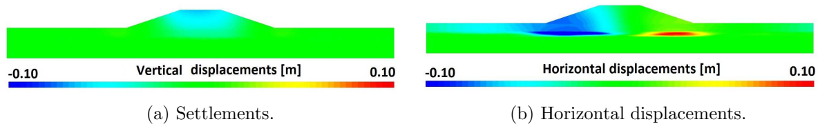
Figure 6.15: Liquefiable layer in depth (Ra9 motion): Deformed shape at the end of the ground motion.
