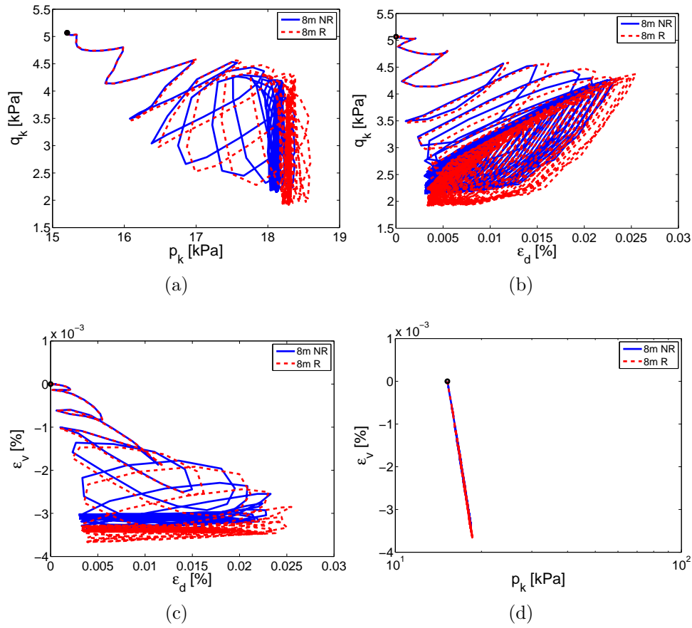
Figure G.21: Mechanical behavior with isotropic mechanism deactivated and zero shear-induced volumetric deformations (8m from base): a) p_k - q_k , b) q_k - \varepsilon_d , c) \varepsilon_v - \varepsilon_d , d) p_k - \varepsilon_v .
