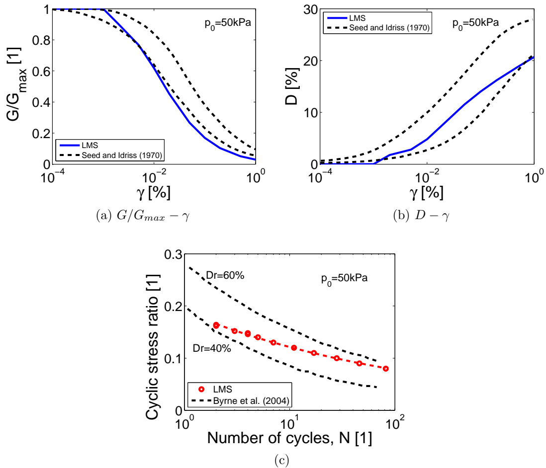
Figure 3.2: Soil response of one material point with the ECP constitutive model ( p_0=50\text{kPa} , K_0=1.0 ): a), b) Shear cyclic drained test compared to Seed and Idriss (1970), c) Cyclic triaxial undrained test: Liquefaction curve compared to Byrne et al. (2004).
