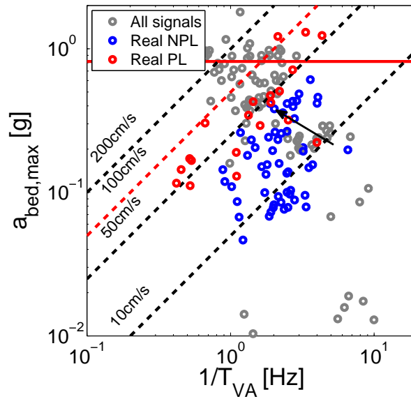
Figure 3.30: Relation between input IM: a_{bed,max} and T_{V,A} - Comparison of NPL / PL.
