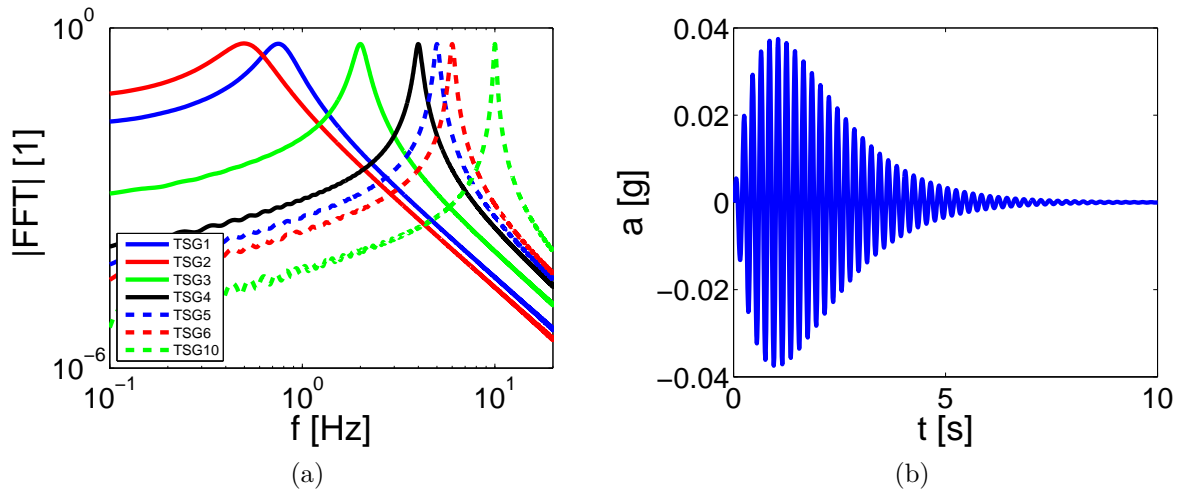
Figure G.1: Input analytical signals: a) Fourier transform, b) Accelerogram of TSG5.
