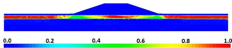
Figure 6.41: Excess pore water pressure ratio ( r_u ) during the mainshock ( t=5s ) of the strong motion (Ra9).
