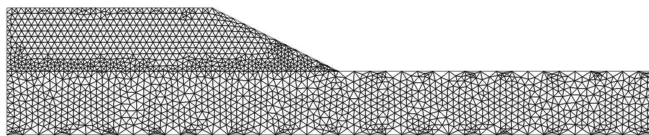
(c) Mesh 3 (15cm)
