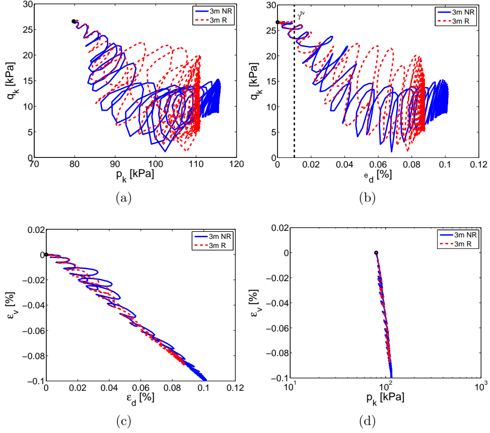
Figure G.10: Mechanical behavior (3m from base): a) p_k - q_k , b) q_k - \epsilon_d , c) \epsilon_v - \epsilon_d , d) p_k - \epsilon_v .
