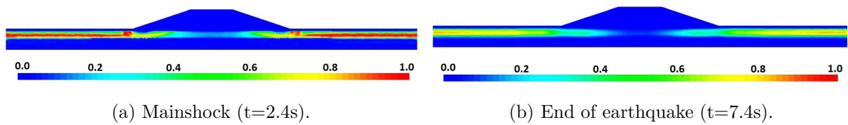
Figure 6.7: Typical dynamic response (irsn168 motion): Excess of pore water pressure ratio r_u .
