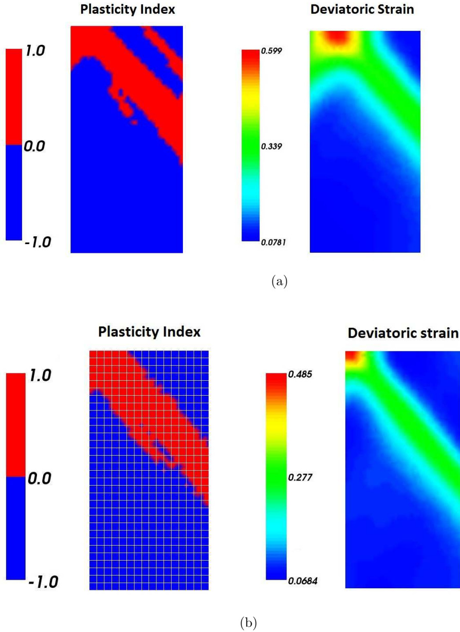
Figure F.9: Biaxial test of Hostun sand (DR=88%) with p_0 = -100\text{kPa} : a) a_1/25 = 26\text{Pa} \cdot \text{m}^2 , t = 0.63\text{s} ( t_{\text{end}} , u_v = 0.025\text{m} ), b) a_1/50 = 13\text{Pa} \cdot \text{m}^2 , t = 0.48\text{s} ( t_{\text{end}} , u_v = 0.02\text{m} ).
