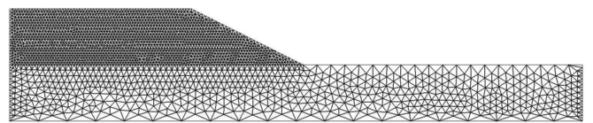
(b) Mesh 2 (10cm)
