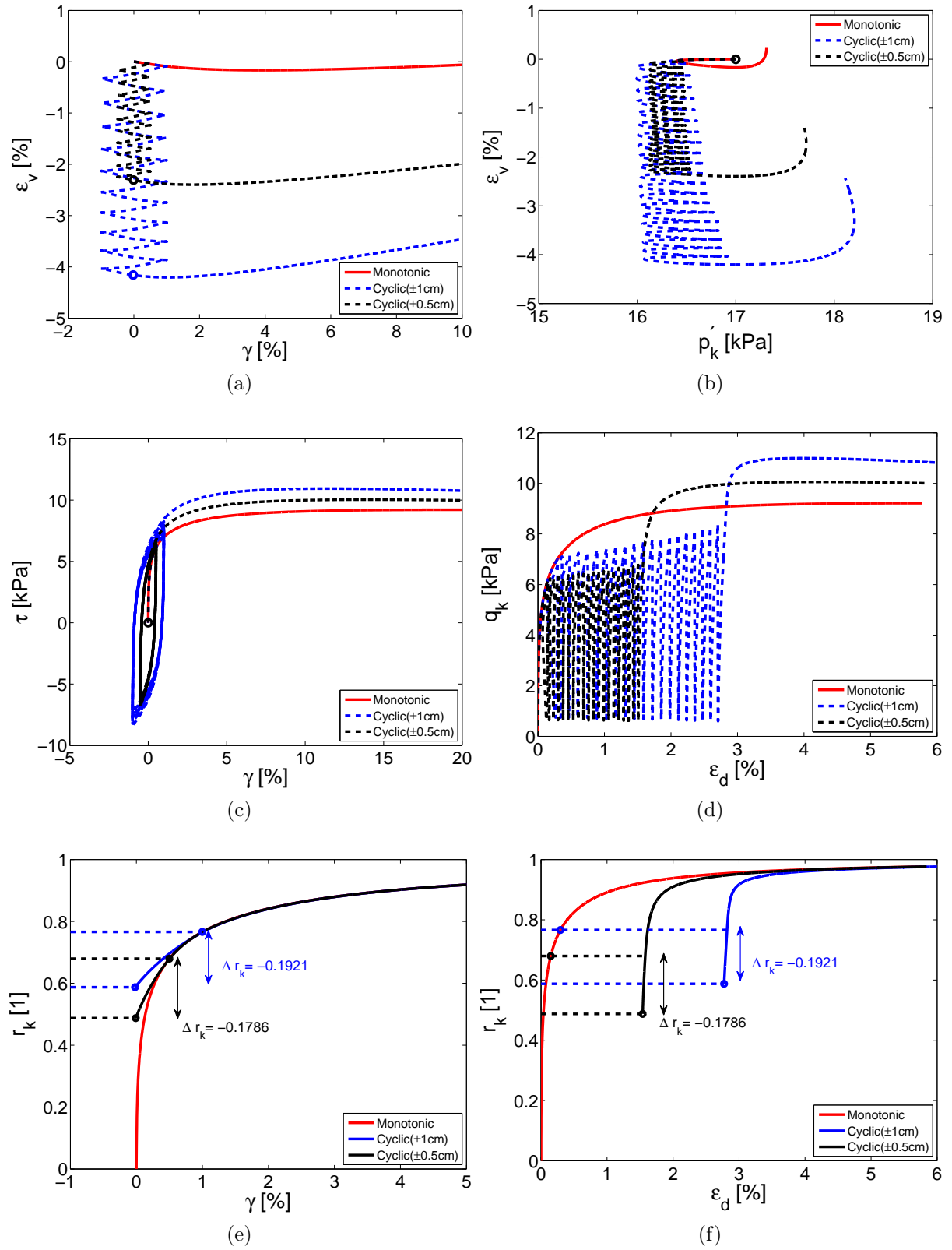
Figure 5.15: Response of one soil element under shear test: a) \varepsilon_v - \gamma , b) \varepsilon_v - p'_k , c) \tau - \gamma , d) q_k - \varepsilon_d , e) evolution of r_k as function of shear strains, f) evolution of r_k as function of deviatoric strains.
