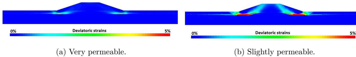
Figure 6.26: Influence of soil's permeability (irsn168): Deviatoric strains \varepsilon_d at the end of the ground motion.
