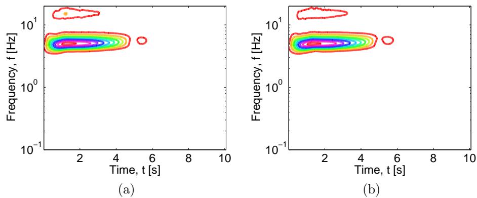
Figure G.15: S-transform for the FF horizontal acceleration with zero shear-induced volumetric deformations: a) Without regularization, b) With regularization.
