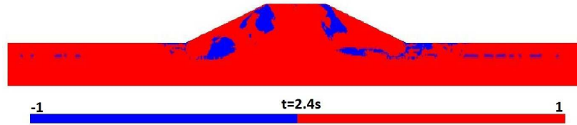
Figure 6.9: Typical dynamic response (irsn168 motion): Contours of second order work at t=2.4s (mainshock).
