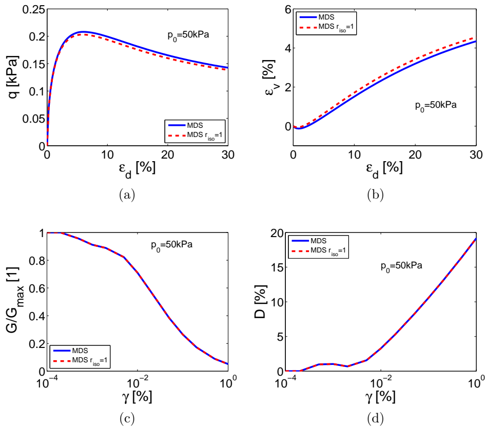
Figure G.12: Soil response of one element with isotropic mechanism deactivated: a,b) Drained triaxial test, c,d) Cyclic shear drained test.
