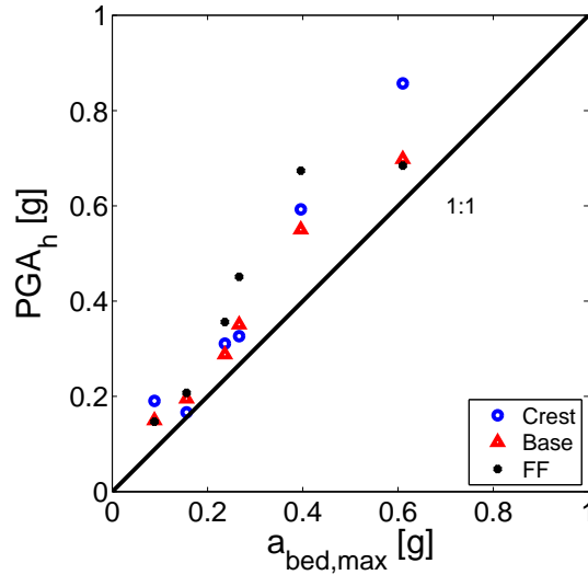
Figure 5.11: Horizontal PGA as function of a_{bed,max} for mesh 4 (25cm).
