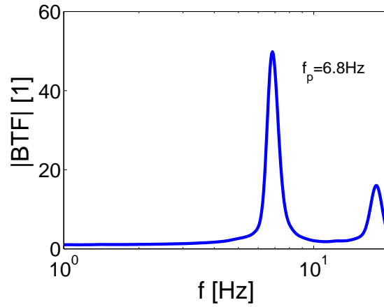
Figure 3.3: Borehole Transfer Function of coupled HM soil column in elasticity.
