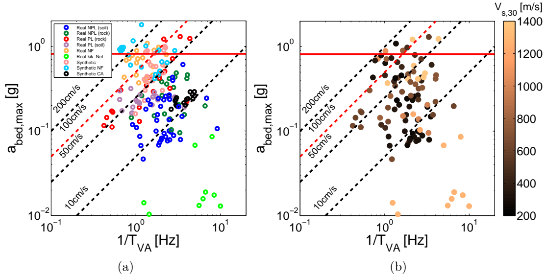
Figure 3.18: Relation between input IM: a_{bed,max} and T_{V/A} : a) Classification of all ground motions, b) Classification of real earthquakes according to V_{s,30} of the site.
