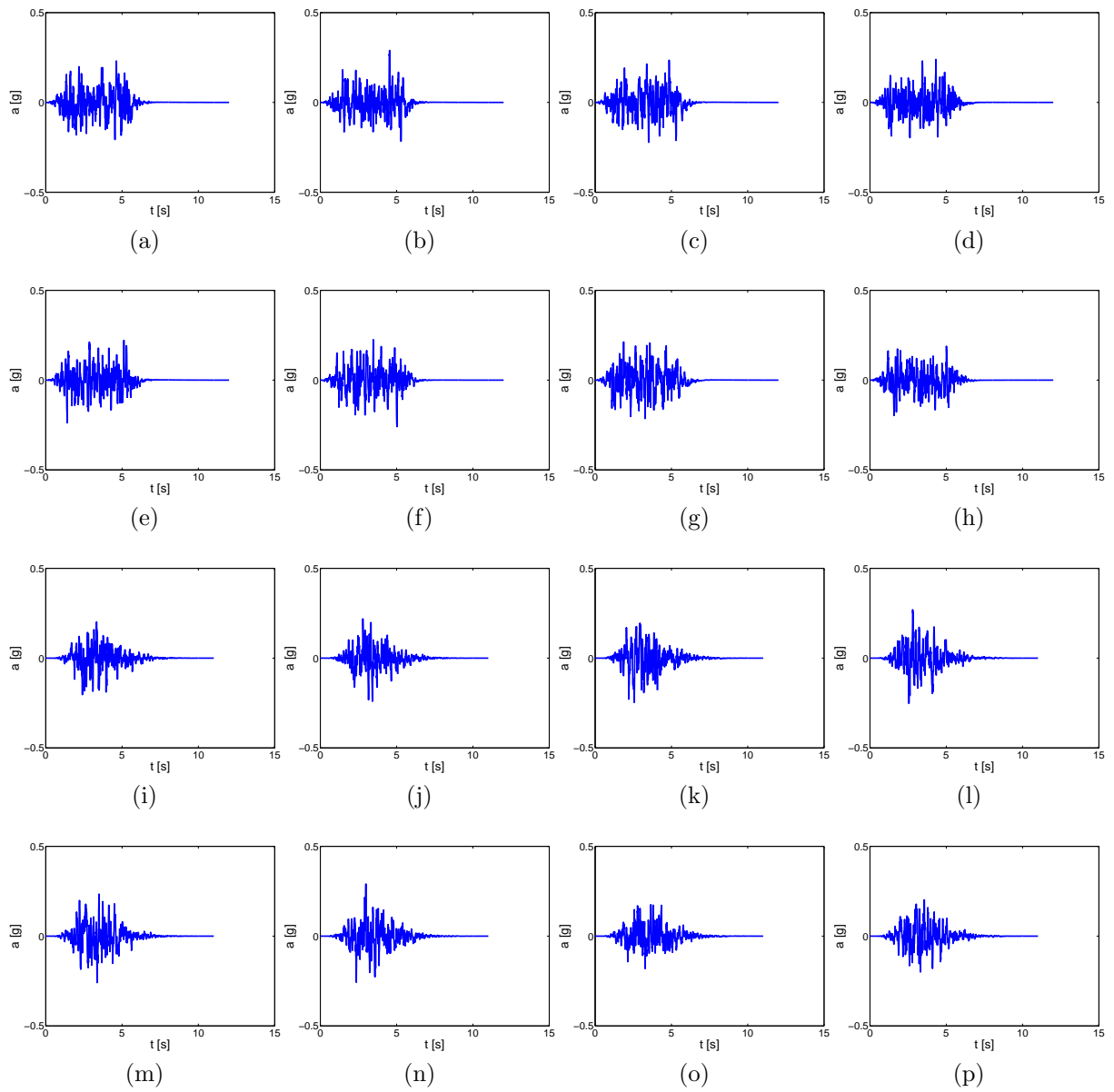
Figure C.15: Accelerograms of synthetic earthquakes generated in Code_Aster .
