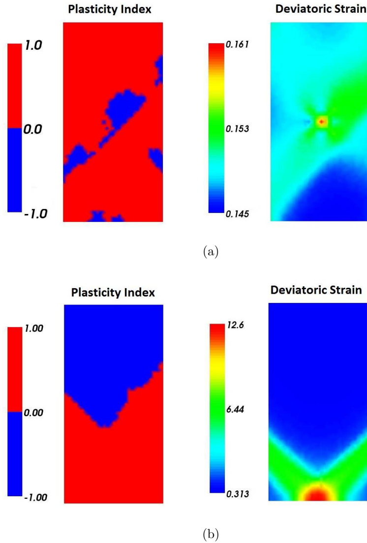
Figure F.6: Biaxial test of Hostun sand (DR=88%) - p_0 = -500 \text{ kPa} , a_1 = 1500 \text{ Pa} \cdot \text{m}^2 : a) t = 0.15 \text{ s} ( u_v = 0.024 \text{ m} ), b) t = 2 \text{ s} ( t_{\text{end}} , u_v = 0.32 \text{ cm} ).
