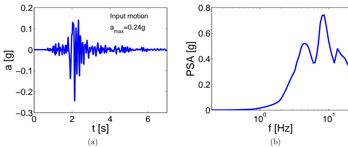
Figure C.12: irsn168: a) Accelerogram, b) Spectrum ( \xi=5\% ).
