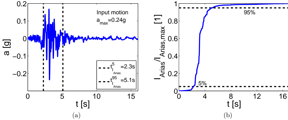
Figure 3.5: Input ground motion (Friuli earthquake): a) Accelerogram, b) Arias intensity.
