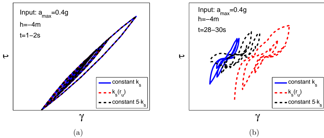
Figure 3.38: Comparison of shear stresses ( \tau ) - shear strains ( \gamma ) of three simulations at h=-4m from the surface for the strong input motion ( a_{\max}=0.4g ): a) t=1-2s , b) t=28-30s .
