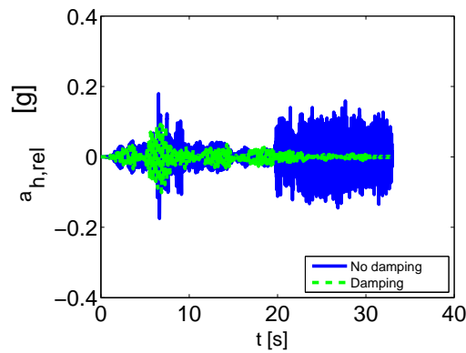
Figure A.2: Comparison of results with and without numerical damping: Horizontal relative acceleration at column's surface.
