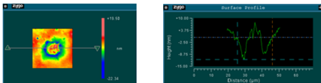
Figure 3.42. A PJ etching profile obtained on glass plate using a barium-titanate microsphere D_s = 87 \mu\text{m} ( F_z = 0.7 \text{ J/cm}^2 )
