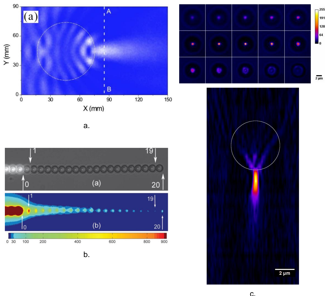
Figure 2.9. Capture of PJ appearance: (a) Spatial distribution of the field intensity at 12 GHz using a Teflon cylinder with a diameter of 60 mm [64]; (b) Nanojet induced mode (NIM) visualization in a chain of 2.9 \mu\text{m} spheres in white-light illumination and without background illumination [60]; (c) A stack of raw images from a 5 \mu\text{m} sphere captured with a steps of 500 nm towards the sphere which and the PJ reconstruction on optical axis build from the stack of raw images [34]
