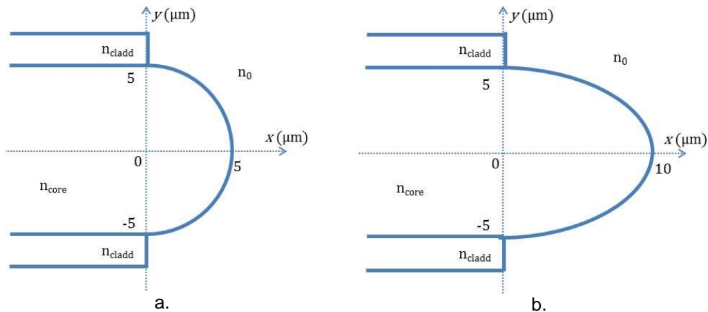
Figure 4.47. Geometrical design of SMF-28, 10\ \mu\text{m} optical fiber core diameter in 2D: (a) circular tip and (b) elliptical tip ( b = 2a )
