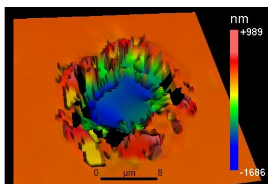
Figure 3.37. Sharp spikes/column and hillocks around a crater yielded by the larger glass microspheres ( D_s of 24 \mu\text{m} and 35 \mu\text{m} )
