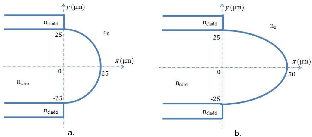
Figure 4.51. Geometrical design of MMF 50 \mu\text{m} optical fiber in 2-D: (a) circular tip and (b) elliptical tip.
