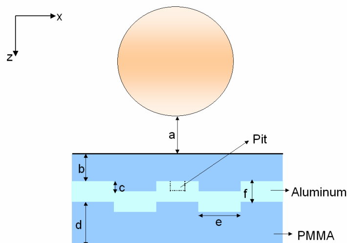
Figure 2.18. The proposed optical data-storage geometry using a 2\ \mu\text{m} diameter microsphere with refractive index of 1.59 and the measurements of a = 160\ \text{nm} , b = 480\ \text{nm} , c = 40\ \text{nm} , d = 360\ \text{nm} , e = 160\ \text{nm} and f = 200\ \text{nm} [91].
