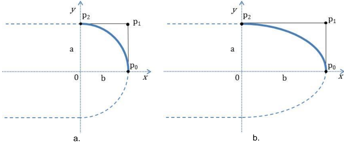
Figure 4.46. Two symmetric rational quadratic Bézier functions are able to describe the optical fiber tip; (a) circular tip and (b) elliptical tip.
