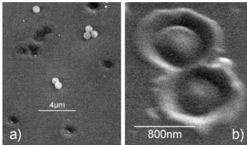
Figure 2.7. Holes observed on silicon surface during laser removal of small polystyrene spherical particles. Laser 6.5 ns pulses at \lambda = 800 \text{ nm} have been used. (a) Higher and (b) lower laser fluence (Figures is taken from [2])
