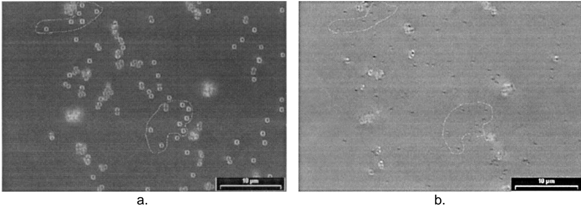
Figure 2.6. Patterns on a Si(100) substrate obtained by irradiating microspheres deposited on the surface. The source is a UV laser ( \lambda = 248 \text{ nm} ; \tau = 23 \text{ ns} ). The silicon surface is observed by an optical microscope (a) before and (b) after laser illuminations. The curved line show the microspheres location and corresponding spots observed after illumination (illustrations taken from [1]).
