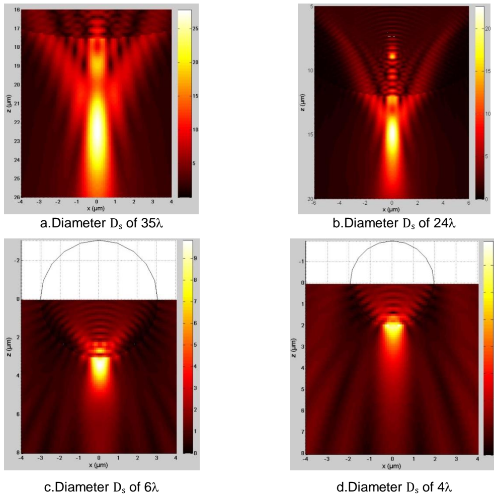
Figure 3.20. The total electric field distribution in XZ plane for a glass microsphere ( n_s = 1.5 ) with a diameter D_s of (a) 35\lambda , (b) 24\lambda , (c) 6\lambda and (d) 4\lambda
