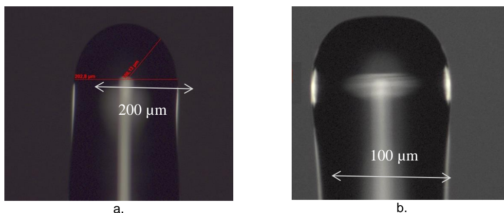
Figure 4.59. The spheroid tipped of (a) our TEQS TM coated multi-mode 200 \mu\text{m} fiber and (b) 100 \mu\text{m} silica fiber fabricated by Loyalite for our experiments
