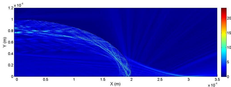
Figure 4.57. Total electric field of a half planar waveguide ( D_s = 200 \mu\text{m} ) with an elliptical tip ( b = 2a , \text{NA} = 0.22 )
