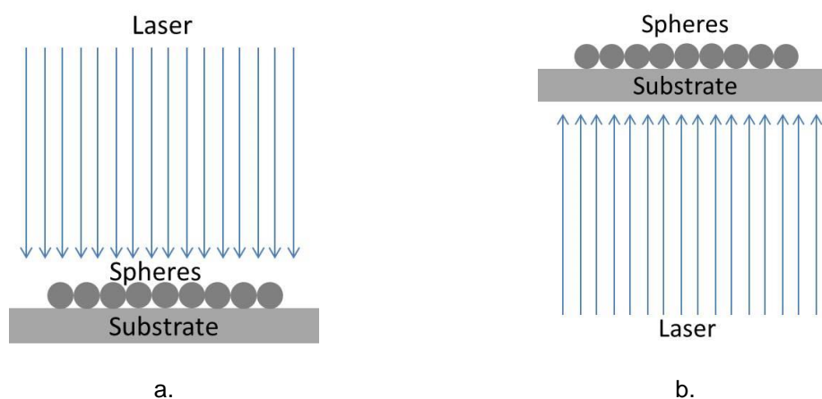
Figure 2.10. Two possible laser illumination schemes, (a) normal and (b) opposite normal direction to the spheres
