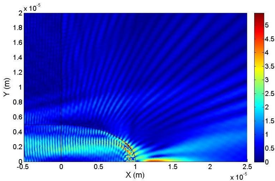
Figure 4.49. Total electric field of a half of planar waveguide ( D_s = 10 \mu\text{m} ) with a circular end (ellipticity = 0.5 or b = 2a , \text{NA} = 0.17 )
