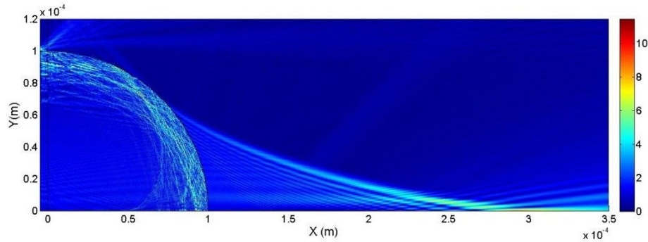
Figure 4.56. Total electric field of a half planar waveguide ( D_s = 200 \mu\text{m} ) with a circular tip ( b = a , \text{NA} = 0.22 )
