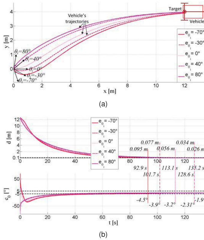
Figure 3.22: (a) UGV's trajectories and (b) its distance d and orientation errors e_\theta for several initial UGV's orientations.
