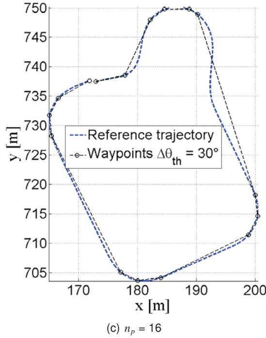
Figure 4.12: Example of waypoint selection based on a reference path and Algorithm 1 (continuation (cont.)).
