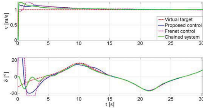
Figure 3.19: Control output.
