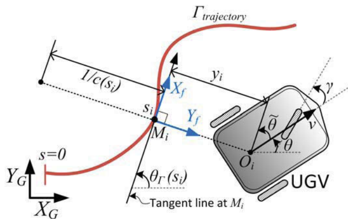
Figure 3.17: Vehicle modeling in Frenet frame.
