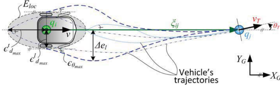
Figure 4.17: Vehicle's trajectories which starts from extreme configurations ( \pm\epsilon_{d_{max}}^l , \pm\epsilon_{\theta_{max}}^l and \pm\epsilon_{\theta_{max}}^l ) in the ellipse of localization uncertainties E_{loc} . \Delta e_l is the maximum lateral deviation of all vehicle's trajectories.
