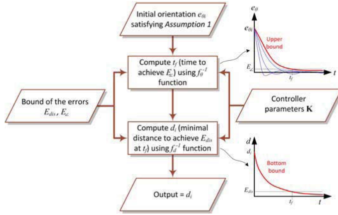
Figure 3.16: Flowchart of the analysis to obtain d_i .
