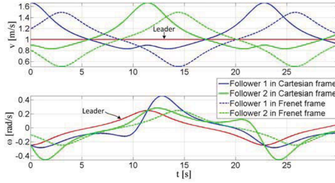
(b) Vehicles' velocities.
