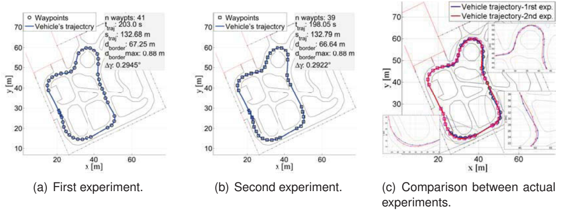
Figure 4.29: Different set of obtained waypoints using OMWS-ET.
