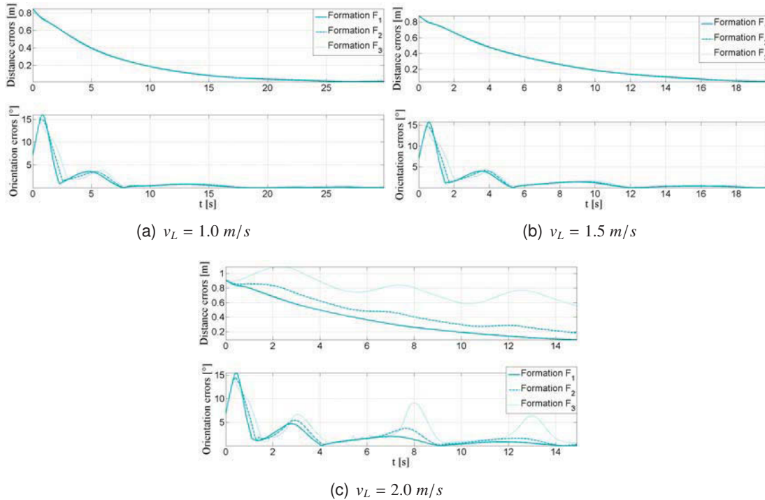
Figure 5.9: Frenet formations \mathbf{F}_1 , \mathbf{F}_2 and \mathbf{F}_3 with different leader's velocities.
