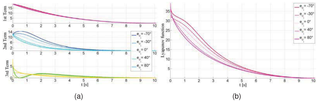
Figure 3.23: (a) Different terms of the Lyapunov function (cf. eq. (3.32)) and (b) Lyapunov function values for several initial orientations.
