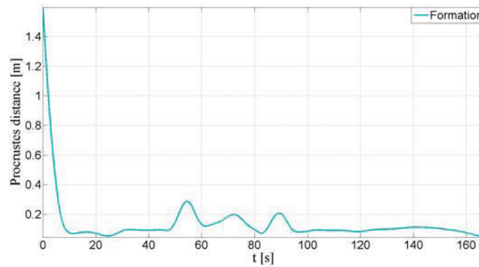
(b) Procrustes distance of the Cartesian formation.
