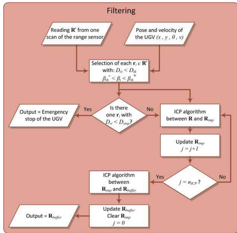
Figure C.3: Flowchart of the Filtering block.
