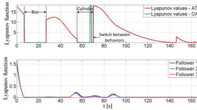
(a) Lyapunov function of each UGV (AT: Attraction to the Target and OA: Obstacle Avoidance).
