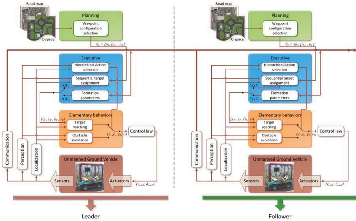
Figure 5.2: Proposed control architecture for navigation in formation of a group of UGVs.
