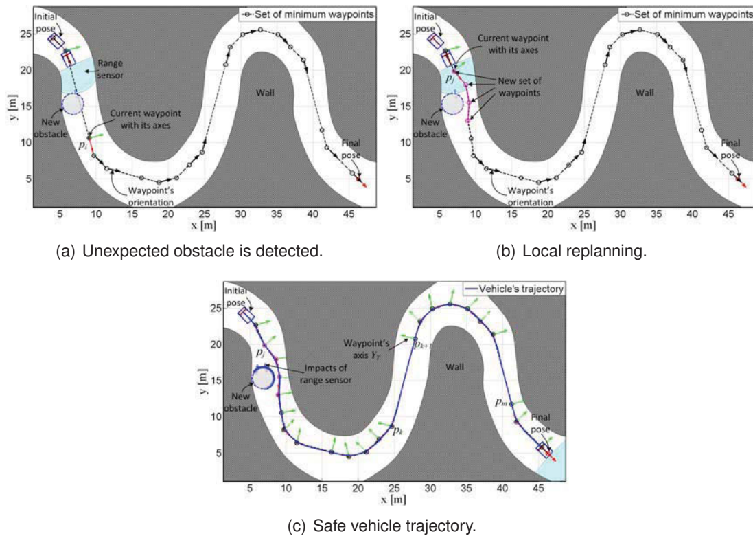
Figure 4.28: Local replanning for unexpected obstacle.
