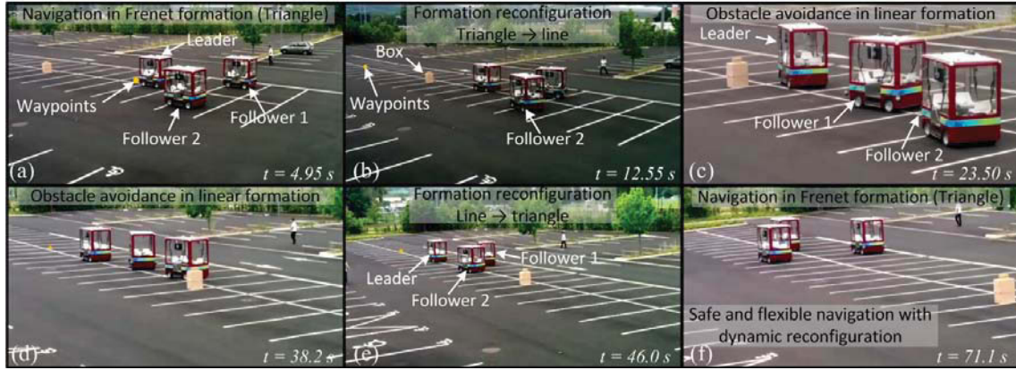
Figure 5.24: Navigation with reconfiguration (SFR-D) in Frenet formation for a group of N = 3 UGVs.
