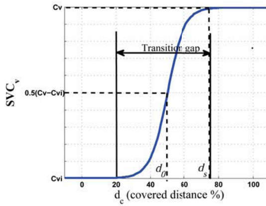
Figure 4.6: Evolution of the \mathbf{SVC}_v , used to ensure smooth control when the waypoint switching occurs.
