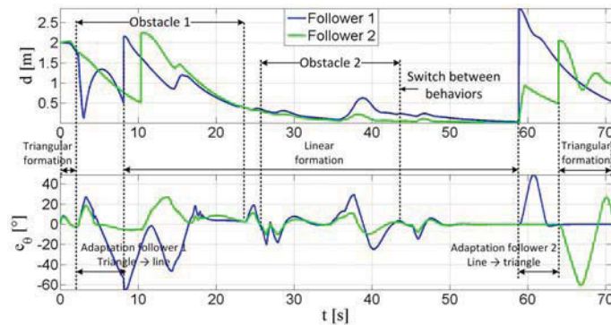
(a) Distance and orientation errors of the UGVs w.r.t. their virtual targets.
