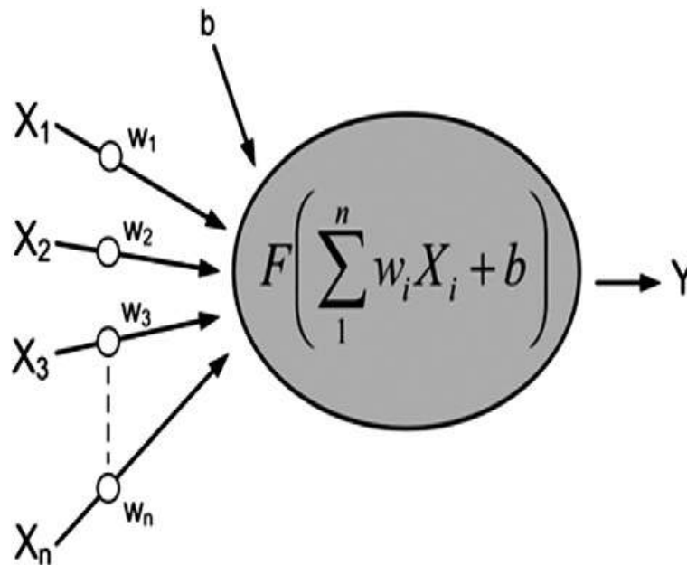
Figure 2-18. Artificial neuron.
