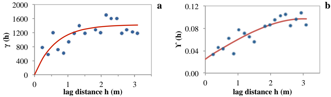
Figure 3-16. Variograms of UPV and CLEP.
