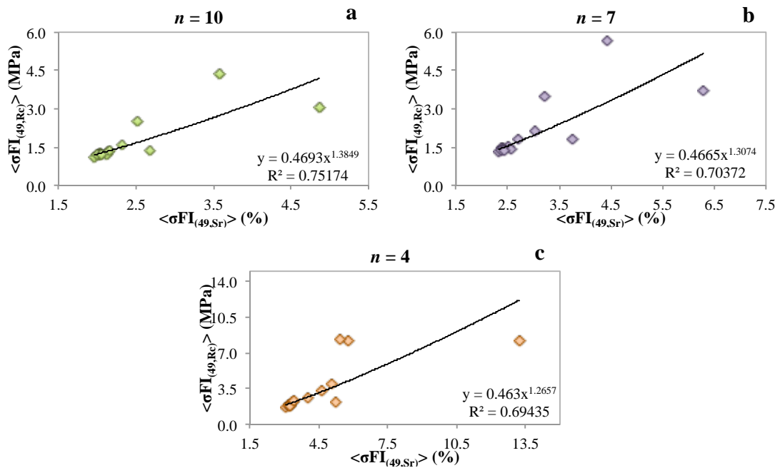
Figure 4-13. \langle\sigma FI_{AT(49,Rc)}\rangle in function of \langle\sigma FI_{AT(49,Sr)}\rangle and \langle\sigma FI_{AT(49,Rc)}\rangle for the 15 configurations for the case: a) n = 10 , b) n = 7 and c) n = 4 .
