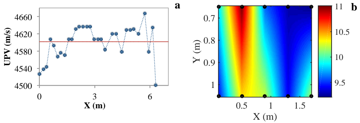
Figure 3-15. a) UPV original profile. b) CLEP original field.
