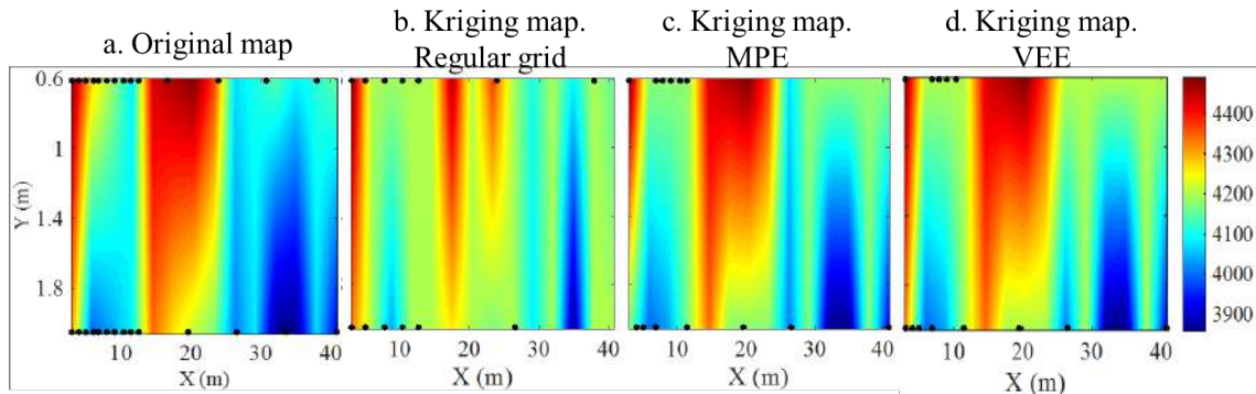
Figure 6-6. a) Original V_p _IE map with 28 measurements, b) Kriging map made with 13 measurements organized in a regular grid, c) Kriging map made with 13 measurements organized in an optimal irregular grid obtained after OSSM with MPE as fitness function, d) Kriging map made with 13 measurements organized in an optimal irregular grid obtained after OSSM with VEE as the fitness function.
