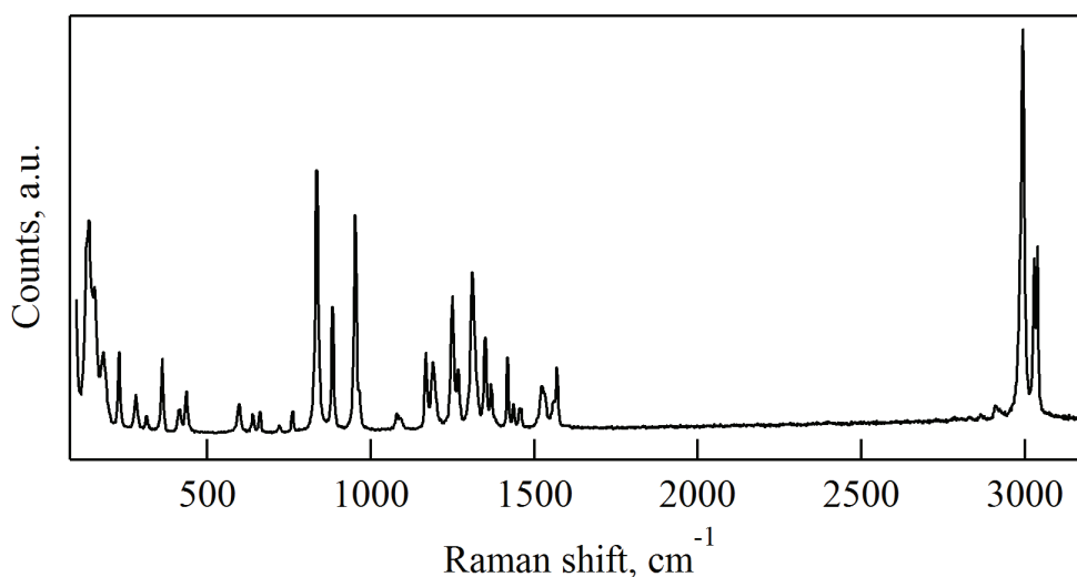
Figure 2.3 – Raman spectrum of the HMX sample used in this work.
