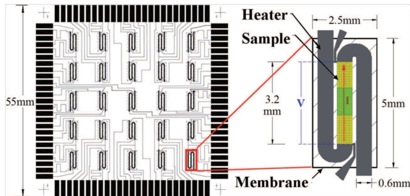
Figure 1.13 – Schematic of the PnSC device and calorimetry sensor developed by Prof. Vlassack [19].
