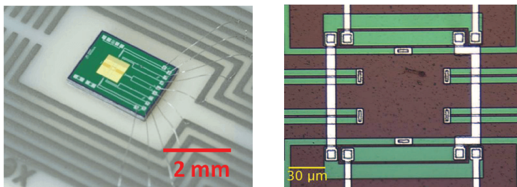
(a) Sensor mounted on a ceramic planar housing.
