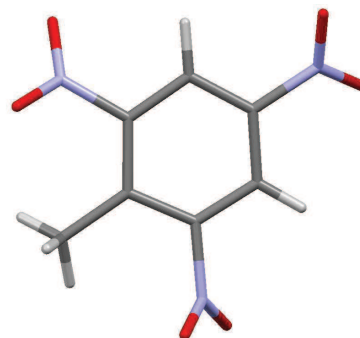
(b) Molecular conformation of TNT in the monoclinic phase.
