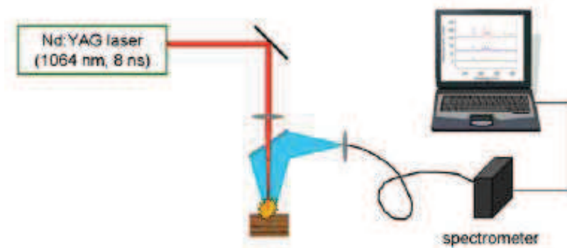
Figure 1.23 – Scheme of a Laser-Induced Breakdown Spectroscopy system [89].
