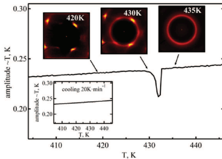
(b) Amplitude of the temperature modulation recorded simultaneously with X-ray diffraction for the heating ramp. The inset gives the curve corresponding to cooling and two-dimensional WAXS patterns measured at different temperatures.
