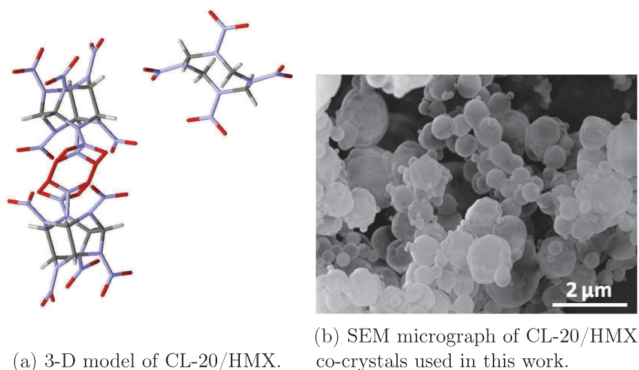
Figure 2.18 – 3-D model and micrograph of CL-20/HMX co-crystal.
