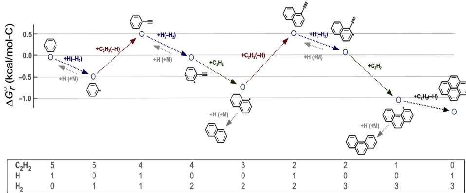
Figure 2.3: HACA mechanism as an example of formation of larger aromatic rings from phenyl for benzene at 1800K according to the illustration from Wang (2011) .
