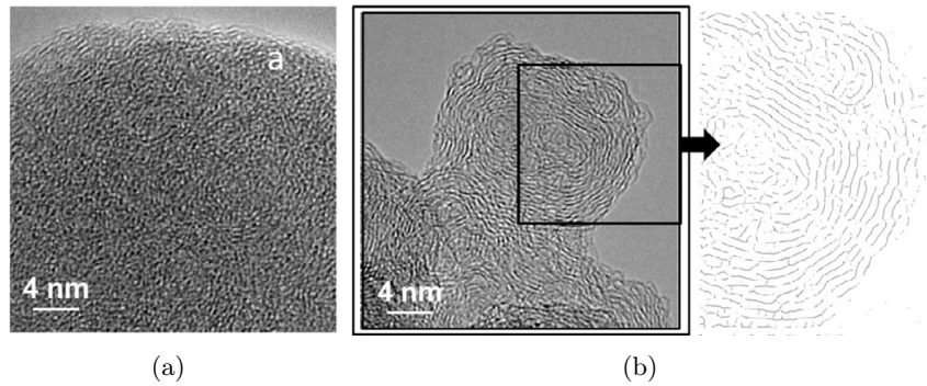
Figure 2.4: HRTEM (High-Resolution TEM) analysis example from the studies of Apicella et al. (2015): (a) nascent soot HRTEM image ; (b) mature soot HRTEM image and their resulting morphology for fringe analysis. (Reprinted with permission from Elsevier.)
