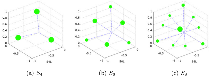
Figure 3.6: Illustration of the discrete directions and their weights, used for the H-G test and for the computation of scattering and configuration averaging in DDA, according to the level symmetric quadrature sets proposed by Fiveland (1991), values are retrieved from Lemonnier (2007). Size of the spheres is proportional to the weight of the corresponding direction cosines.
