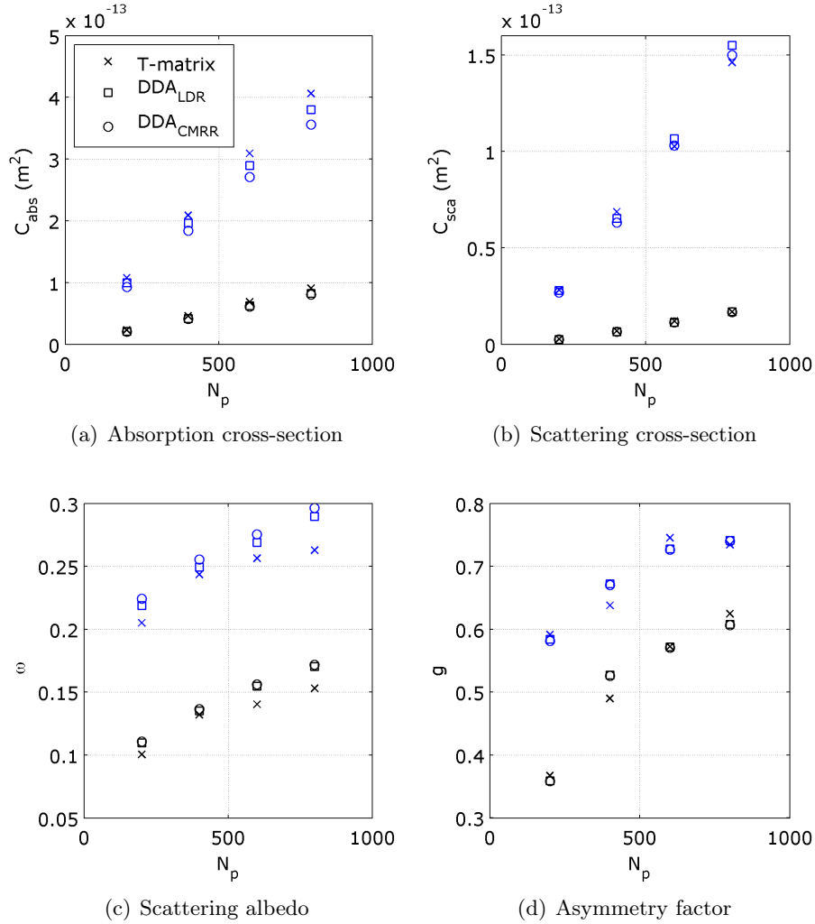
Figure 4.5: Test cases 4a and 4b of Table 4.1. Radiative properties of soot aggregates for fractal dimension D_f = 2.0 as a function of aggregate size N_p composed of d_p = 30 nm (black points) and d_p = 50 nm (blue points). Simulations are performed with optical index m = 2.0 + 1i at \lambda = 870 nm. T-matrix solution values are retrieved from Liu et al. (2008).
