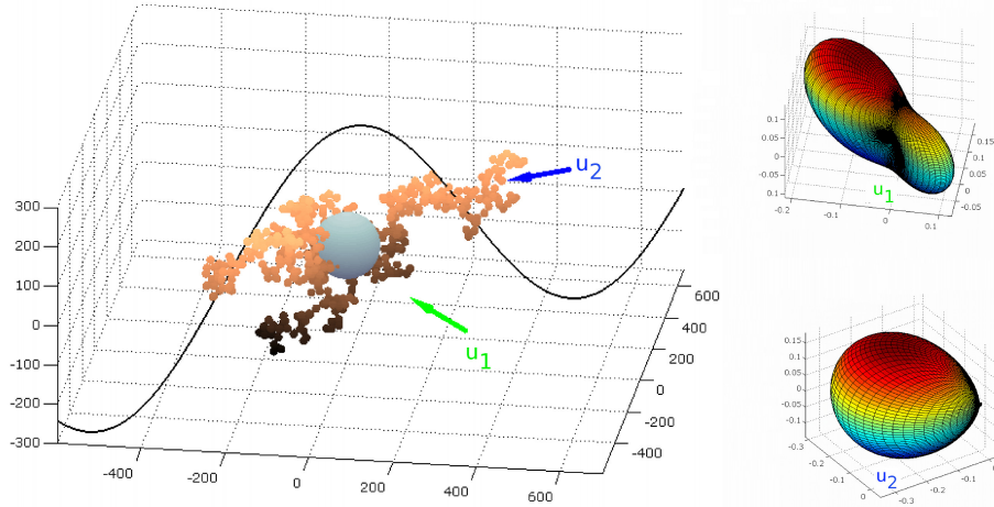
Figure 3.13: Illustration of the phase function of the soot aggregate ( N_p = 500 , d_p = 20nm , D_f = 1.7 and k_f = 2.0 ) for different incidence directions \mathbf{u}_1 and \mathbf{u}_2 using m = 2.0 + 0.5i and \lambda = 1 \mu m .
