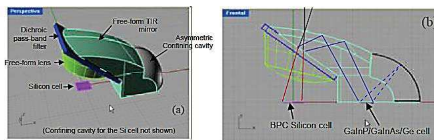
Figure 1.14: Kohler RXI-RR SOE concentrator, with the flat band-pass filter and the 3J and BPC silicon cells [18].
