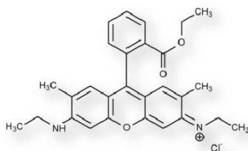
Figure 1 Molecular structure of Rhodamine 6G
