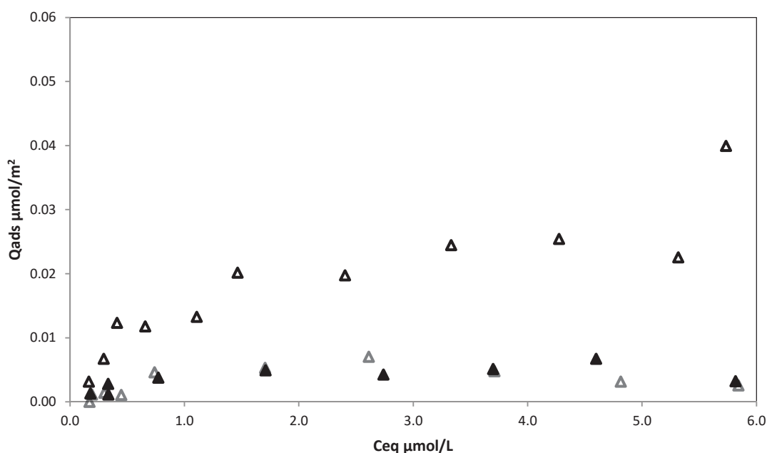
Figure 4. Adsorption isotherms for Rhodamine 6G onto Anatase Commercial nanoparticles at 25^\circ\text{C} from water at natural pH ( \Delta ), from phosphate buffer at pH 6 ( \triangle ) and at pH 8 ( \blacktriangle ).
