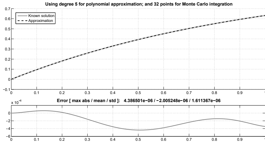
Figure 4.3: Approximation by the proposed method to the ODE that generated Figure 1.2, left plot; same differential as in Figure 4.4, different boundary conditions. Solution y(x) = 1 - \exp(-x) approximated to: \hat{y}(x) = 5.15 \cdot 10^{-3} x^5 - 3.86 \cdot 10^{-2} x^4 + 1.65 \cdot 10^{-1} x^3 - 5.00 \cdot 10^{-1} x^2 + 1.00 x .
