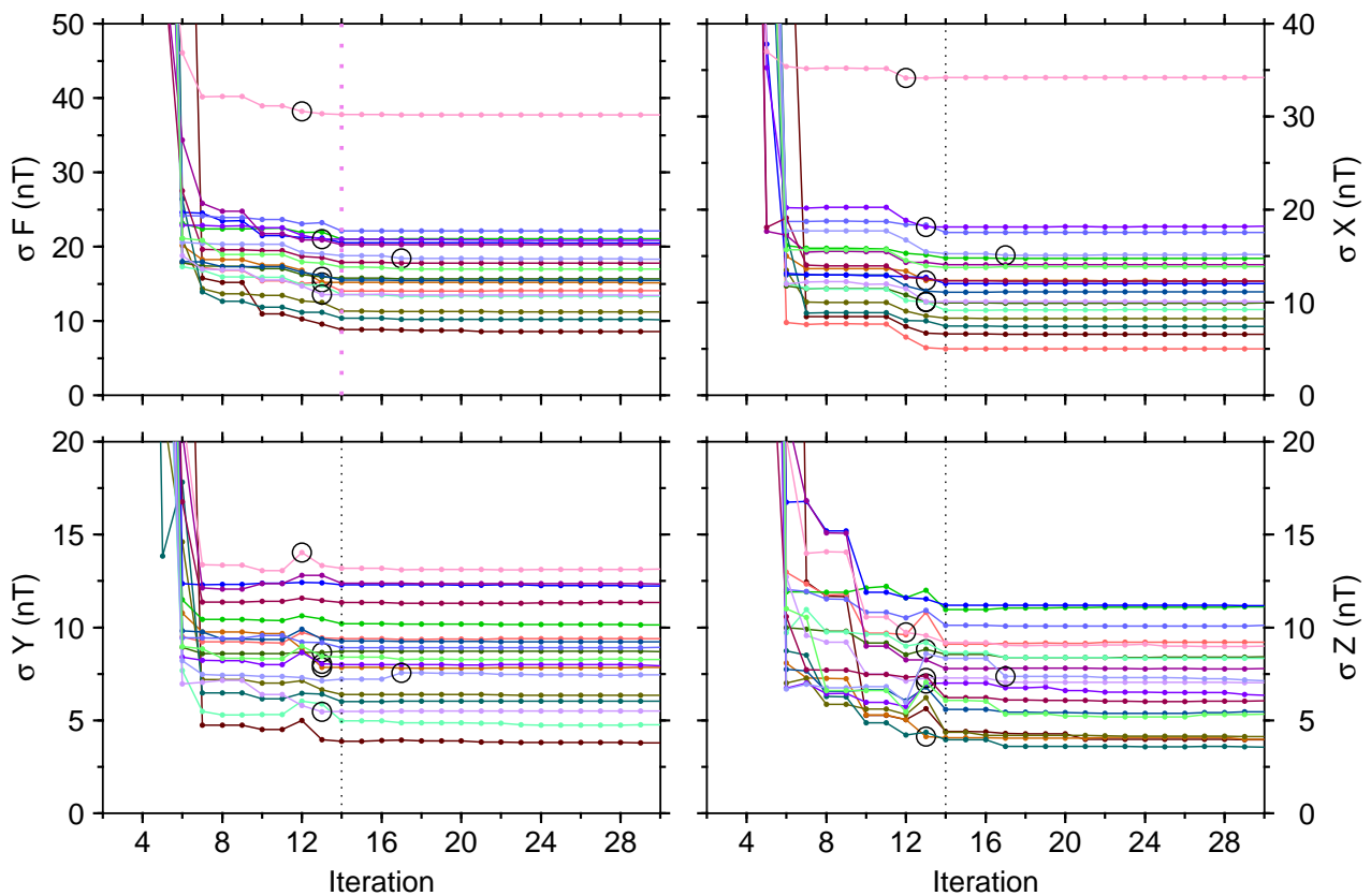
Figure 4.2: Rms residuals between synthetic data and predictions as a function of the inversion solution iteration, around the final selected one. This example corresponds to the application of the VO-ESD approach to a VO centred at \vartheta_{vo} = 21.25^\circ , \phi_{vo} = 54.67^\circ and for eighteen time periods with duration of 30 days.
