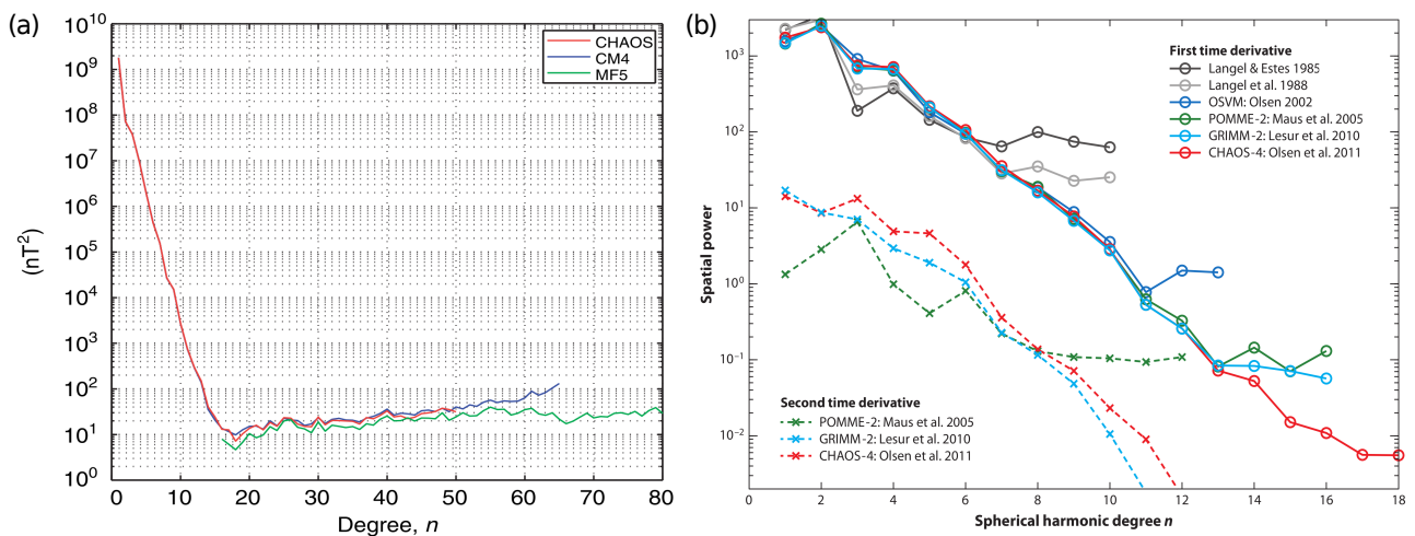
Figure 2.2: (a) Spatial power spectrum of the geomagnetic field (in \text{nT}^2 ) for different models, at the Earth's surface. Figure from Olsen et al. (2007). (b) Spatial power spectrum of first time derivative (secular variation, solid curves, in (\text{nT}\cdot\text{yr}^{-1})^2 ) and second time derivative (secular acceleration, dashed curves in (\text{nT}\cdot\text{yr}^{-1})^2 ) of the geomagnetic field for various magnetic field models, at the Earth's surface. Figure from Olsen and Stolle (2012).
