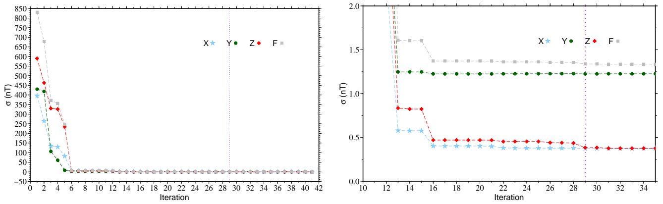
Figure 3.31: Rms residuals between synthetic data and predictions for ( left ) all inversion iterations and ( right ) for a zoom around the selected iteration solution, for each magnetic component and the field intensity for the case of synthetic Swarm orbits without noise within a VO volume centred at CLF. The selected iteration solution is highlighted with a violet vertical dotted line.
