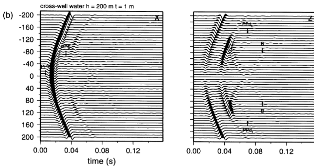
Figure 4.11: Reference seismograms extracted from [54].
