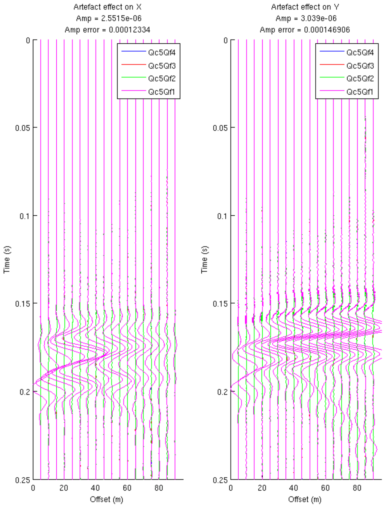
Figure 3.23: Spurious effects ( u_{ref} - u_h ) for Q_5 coarse elements and Q_4, Q_3, Q_2, Q_1 fine elements and with temporal refinement pt = 20 and spatial refinement ps = 20 .
