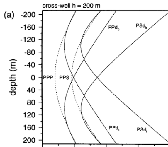
Figure 4.10: Ray-theoretical traveltimes extracted from [54].
