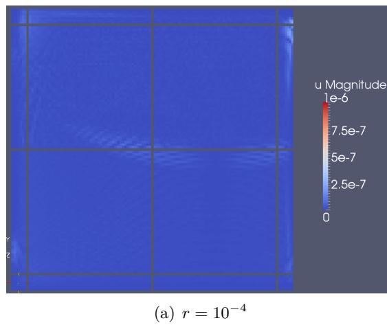
Figure 2.12: Magnitude of the displacement for a color scale divided by a factor of 1/r = 10^4 at T = 0.5\text{s} , for an heterogeneous medium (see figure 2.10).
