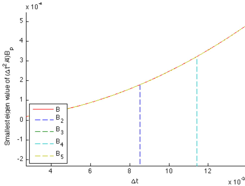
Figure 3.11: Minimum eigenvalues of B_p for p = 2, 3, 4, 5 compared to those of B .
