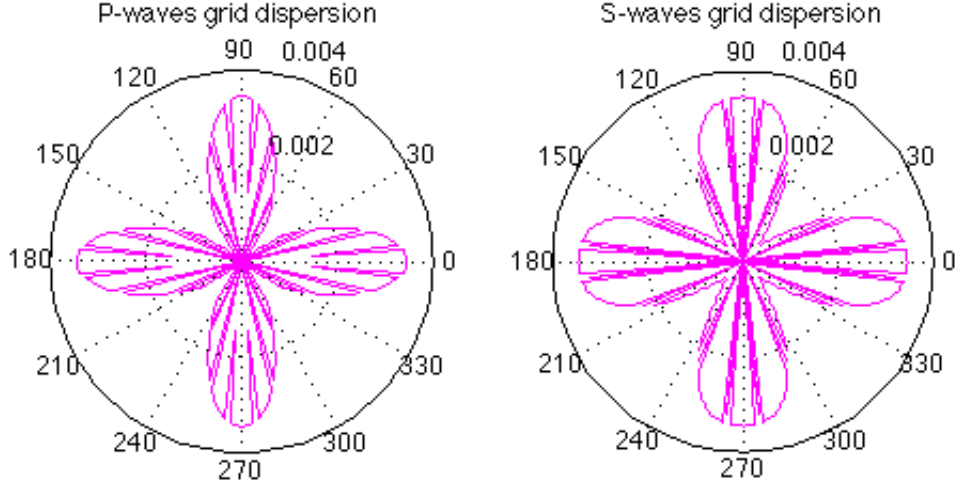
Figure 1.10: Dispersion anisotropy for Q_5 elements with 5 points per wavelength.
