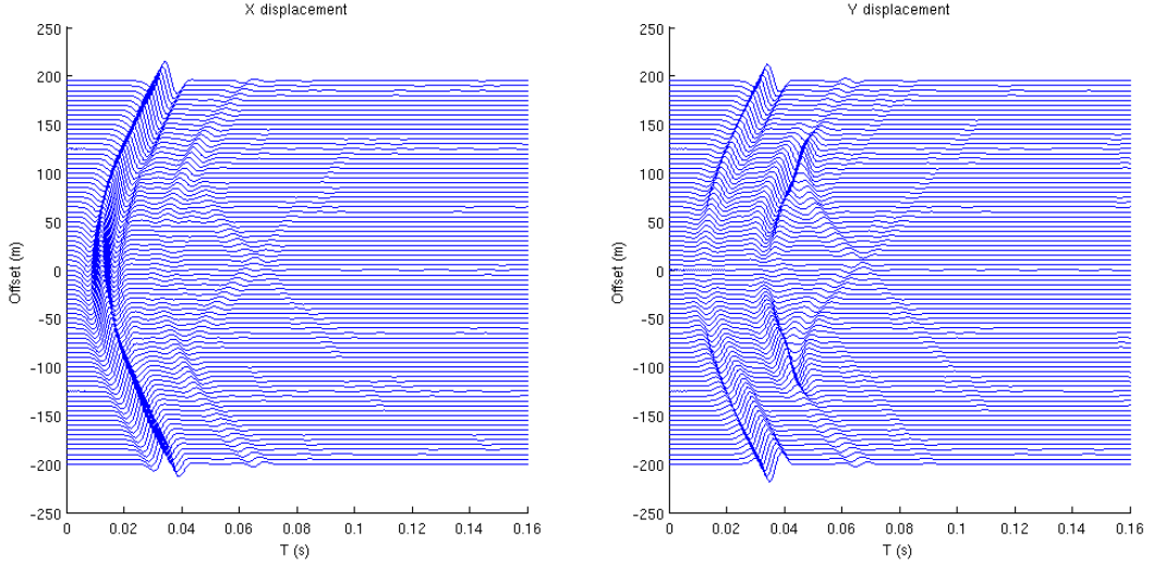
Figure 4.12: Seismograms.
