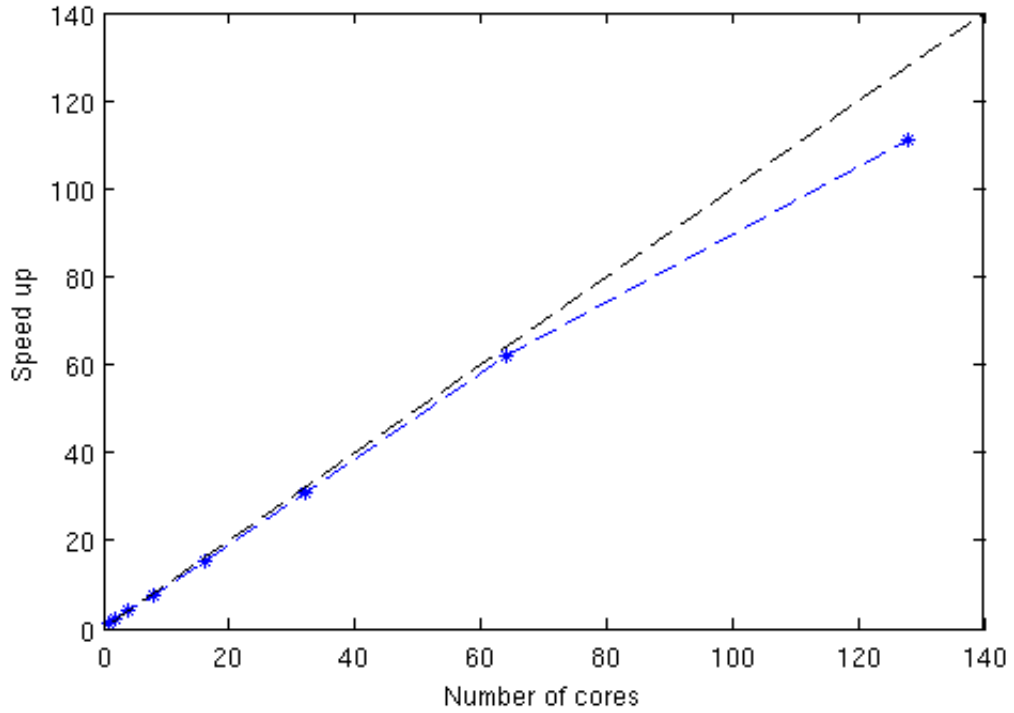
Figure 5.13: Strong scalability.
