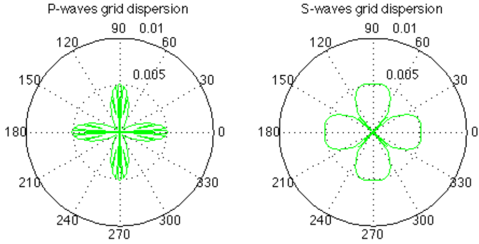
Figure 1.8: Dispersion anisotropy for Q_3 elements with 6 points per wavelength.
