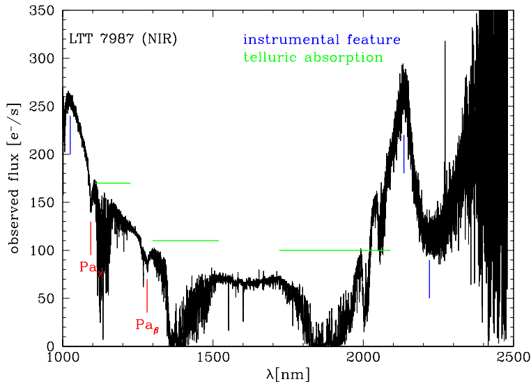
Figure 6: Near-infrared X-shooter spectrum of LTT 7987, taken from Moehler et al. (2014).
