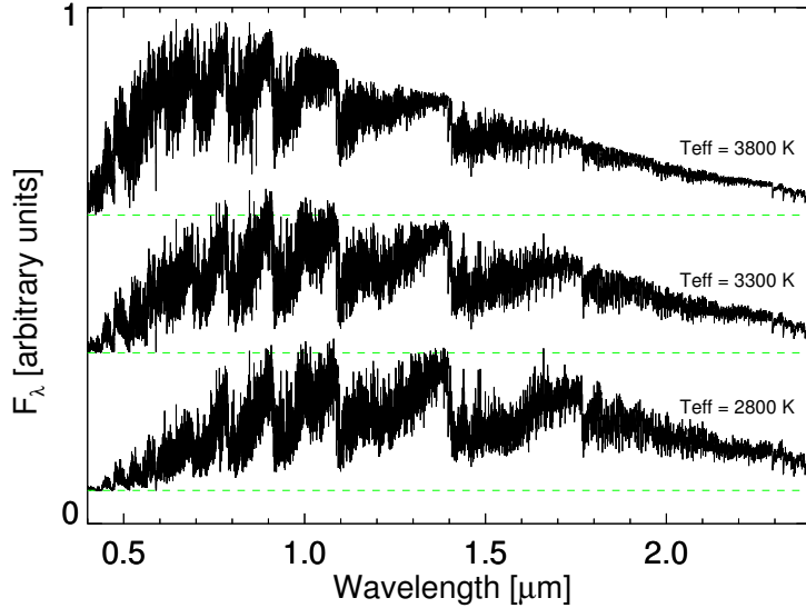
Figure 3.3: Examples of synthetic spectra of C-rich giants with different temperatures ( \log(g) = 0 , C/O = 1.10 and [Fe/H] = 0 ). The spectra are normalized around 1.35 \mu m for display purposes.
