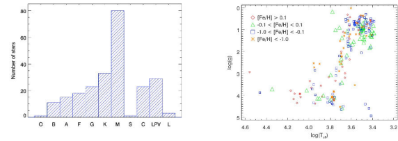
Figure 1: Distribution of the spectral types in XSL observed in Periods 84 and 85 (excluding telluric calibrators). Spectral types were retrieved from SIMBAD or based on educated guesses from the source libraries or atmospheric parameters. Figure 2: HR diagram of the 219 XSL stars (O–M, LPV, S) with calculated T_{\text{eff}} , \log g , and [\text{Fe}/\text{H}] , where [\text{Fe}/\text{H}] is presented in different colors.
