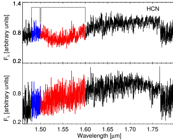
Figure 2.11: Zoom into the HCN+C 2 H 2 lines around 1.53\ \mu\text{m} . The upper panel shows an example of a carbon star, SHV 0502469-692418, in which the HCN+C 2 H 2 feature is visible. The lower panel corresponds to another carbon star, T Cae, in which the feature is missing. The red line indicates the region used to calculate the absorption bandpass, while the blue line corresponds to the “continuum” bandpass.
