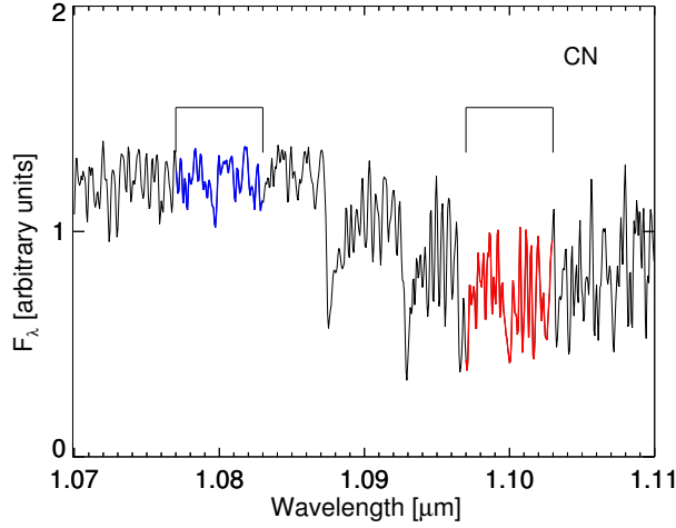
Figure 2.10: Zoom into the CN line near 1.1\ \mu\text{m} . The red line indicates the region used to calculate the W110 bandpass, while the blue line corresponds to the W108 bandpass measuring the “continuum”. This star is SHV 0502469-692418.
