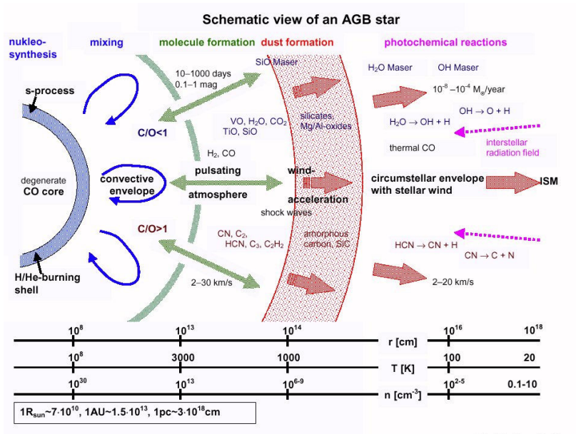
Figure 1.11: Schematic view of an AGB star ( credit dr. J. Hron ).
