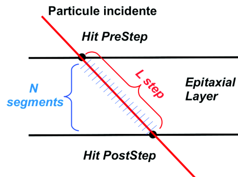
FIGURE 4.7 – Segmentation de la trace.
