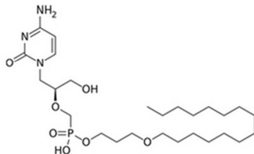
Brincidofovir
