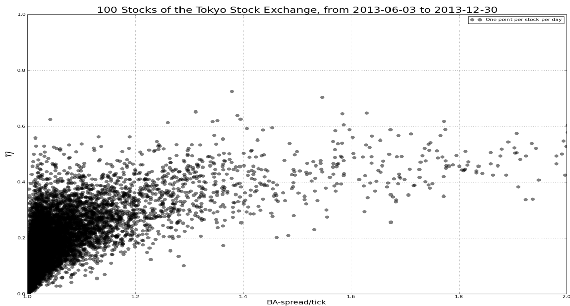
Figure III.2: Daily values of \eta for all the assets of the TOPIX 100 index, for every day so that the daily average spread is smaller than two ticks, from 2013, June 3 to 2013, December 30.
