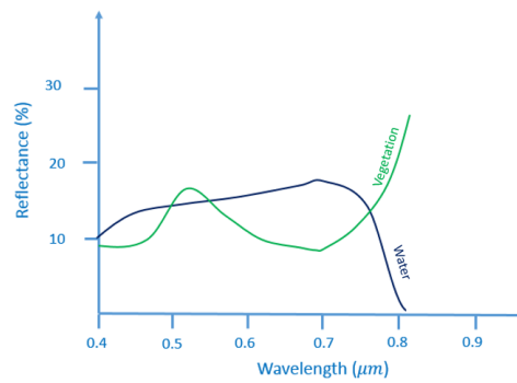
Figure 1.6: Spectral reflectance of vegetation and water.
