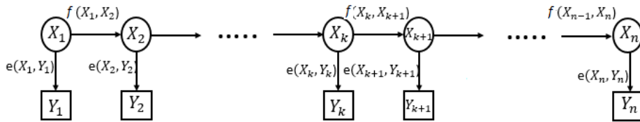
Figure 3.8: Hidden Markov chain.
