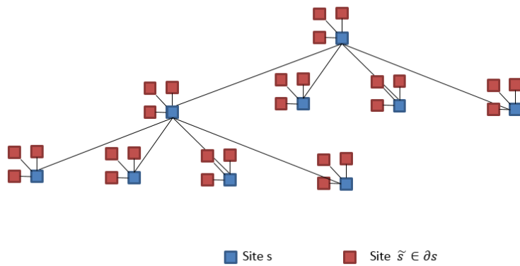
(a) Graphical model for the hierarchical Markov Mesh
