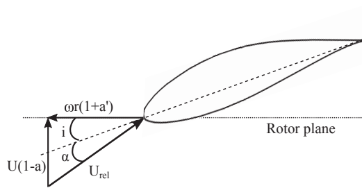
Figure 3.2: Induced velocity in the rotor plane.
