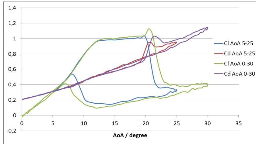
Figure C.8: Lift and drag coefficients for 2 test cases with the same oscillation frequency f = 0.3 \text{ Hz} , and different oscillation amplitudes.
