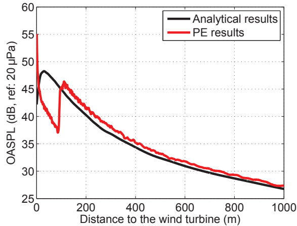
Figure 4.16: Comparison of overall SPL as a function of propagation distance for an impedance ground with \sigma_e = 200 \text{ kPas m}^{-2} between analytical solution and PE results. Observer is at 2 m height in the downwind direction. Blade position parameter \beta = 0^\circ .
