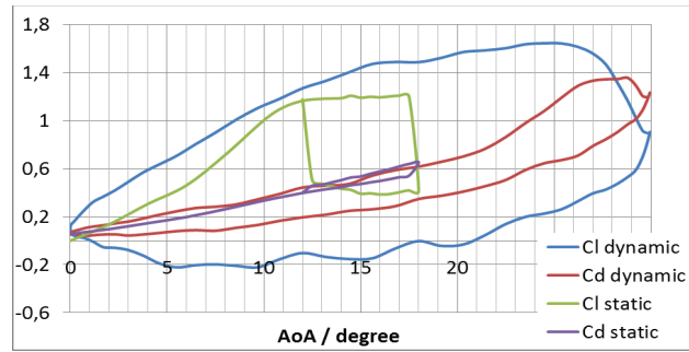
Figure C.6: (Continued) Lift and drag coefficients measured for dynamic stall cases compared to static case. Case 5, f = 2.6 Hz, range of AoA = 0 - 30^\circ .
