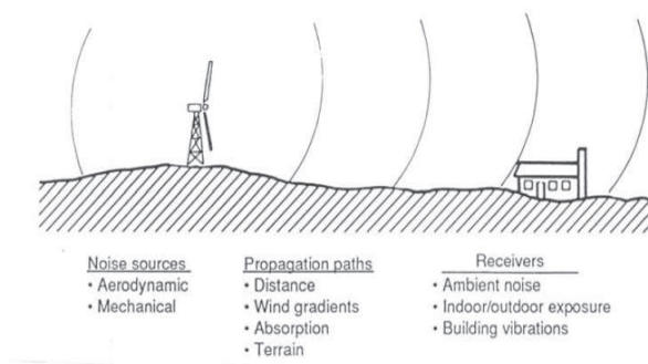
Figure 1.8: Illustration of wind turbine noise generation and propagation. Taken from [7]
