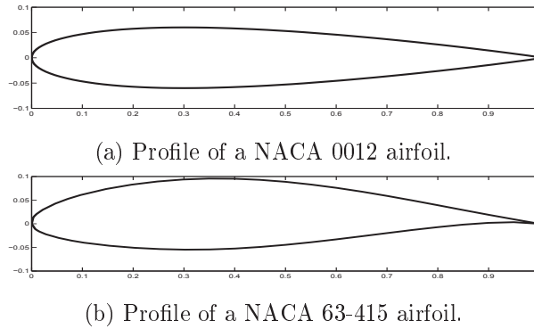
Figure 2.6: Profiles of NACA 0012 and NACA 63-415 airfoil.
