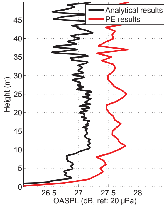
Figure 4.15: Comparison of overall SPL as a function of height for an impedance ground with \sigma_e = 200kPa \cdot sm^{-2} between analytical solution and PE results. Observer is 1000 m away in the downwind direction. Blade position parameter \beta = 0^\circ .
