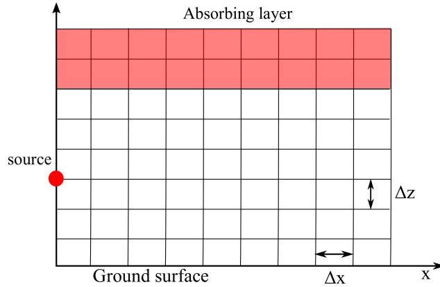
Figure 4.5: Illustration of calculation domain for PE method. Horizontal spacing is \Delta x and vertical spacing is \Delta z . Ground surface is at z = 0 , and propagation direction is along x .
